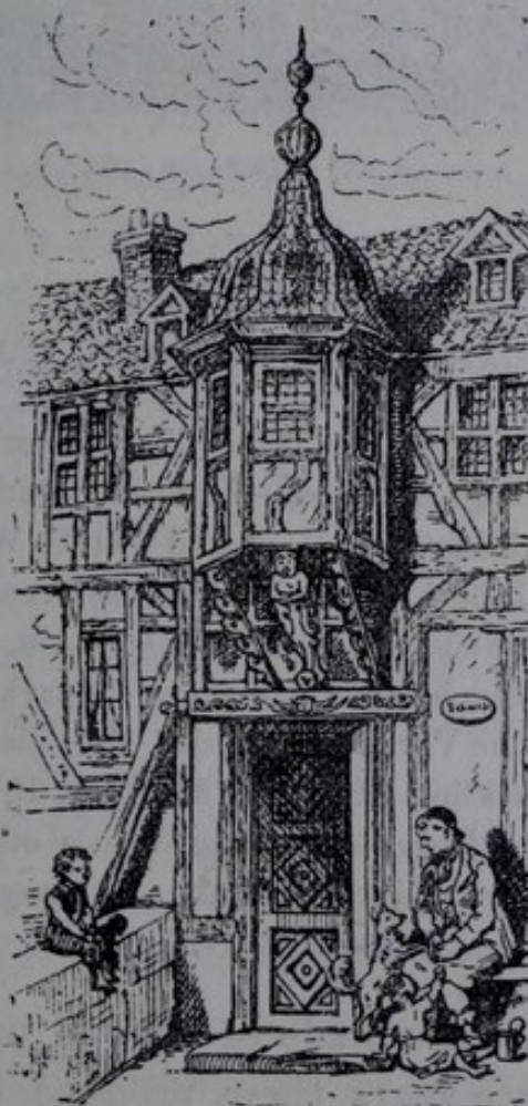
AT AHRWEILER.
