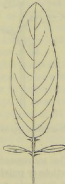
Desmodium gyrans : leaf seen from above, reduced to one-half nat- ural size. The minute stipules unusually large.
