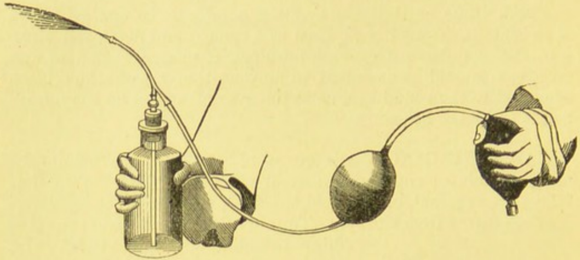
FIG. 64.—Hand Spray-Producer.
