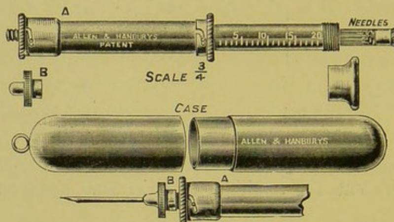
FIG. 120. Metal hypodermic syringe.
