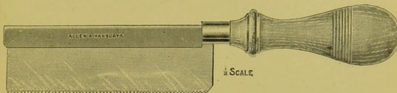
FIG. 116. Metal saw for removing plaster splints.
