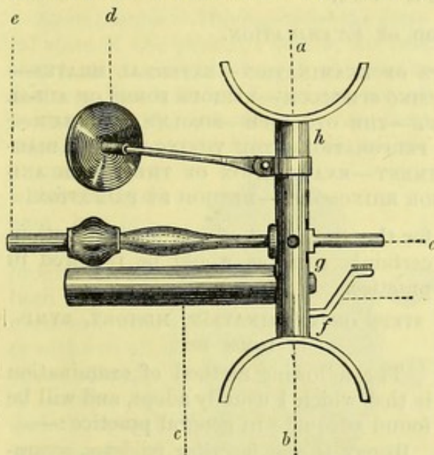
FIG 12.—Poltzer's Acoumeter. a and b , Semicircular vulcanite ends of pillar for forefinger and thumb; h , vulcanite pillar; c , steel cylinder; e , e , steel lever hammer; f , vulcanite check on which to press the lever hammer; d , brass plate at end of steel pin (which in the recent instrument, screws into the vulcanite pillar at h ). In the improved acoumeter the vulcanite pillar and check plate are made of one piece.
