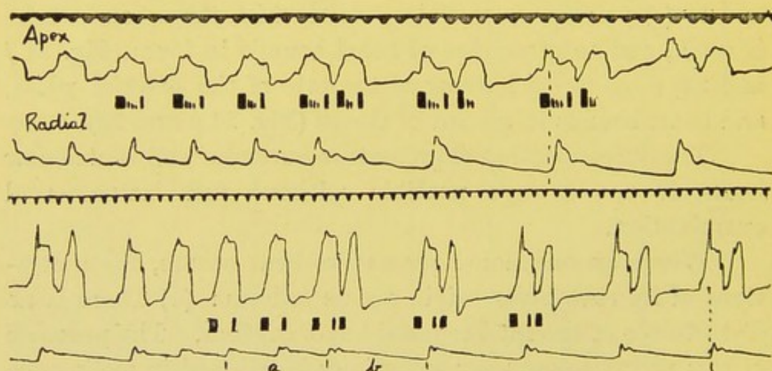
Fig. 27 and 28. Apex and radial curves and heart sounds. The normal mechanism passes into one in which premature ventricular contractions replace alternate normal beats. Fig. 27 is from a case in which mitral regurgitation was present. In Fig. 28, a = b .
