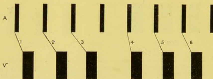
Fig. 11. The next stage of heart-block, to which the term "dropped beats" is applied. Up to the point where the chief disturbance occurs, the gaps between the auricular and corresponding ventricular contractions widen out. The impulses travel to the ventricle with increasing difficulty. The fourth auricular contraction stands isolated, it yields no response; a ventricular contraction is "dropped." Following the ventricular pause, the As-Vs interval is short, for the tissues have rested, but it again widens as successive cycles follow.
