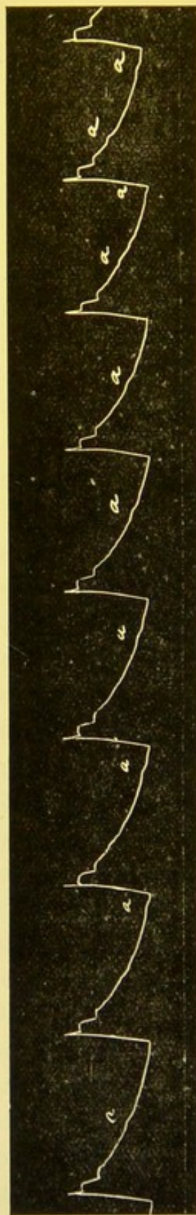
Fig. 21. A sphygmographic curve from the radial artery in a case of complete heart-block. As often happens, signs of auricular systoles ( a ) are visible in the curve and are easily recognised by their regular change of position as they are traced from one radial cycle to the next.
