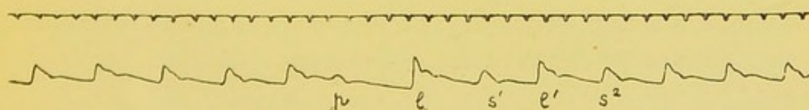
Fig. 48. Alternation of the pulse, appearing after, and as a result of, a single premature beat p . It lasts for four heart cycles.
