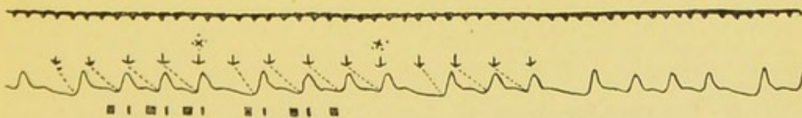
Fig. 14. A pulse curve showing "dropped beats." The arrows, which represent the positions of the regular auricular contractions, have been accurately determined in this and subsequent figures by means of polygraphic curves. The heart sounds are shown diagrammatically. The arrangement of the pulse beats depends upon the lengths of the As-Vs intervals and upon the failure of response at the points marked by asterisks. Note the widening of the As-Vs intervals and accompanying increase of pulse rate before and after each dropped beat.
