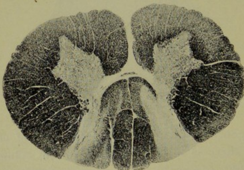
FIG. 15.—Cervical tabes—fifth cervical segment (Leyden and Goldscheider).
