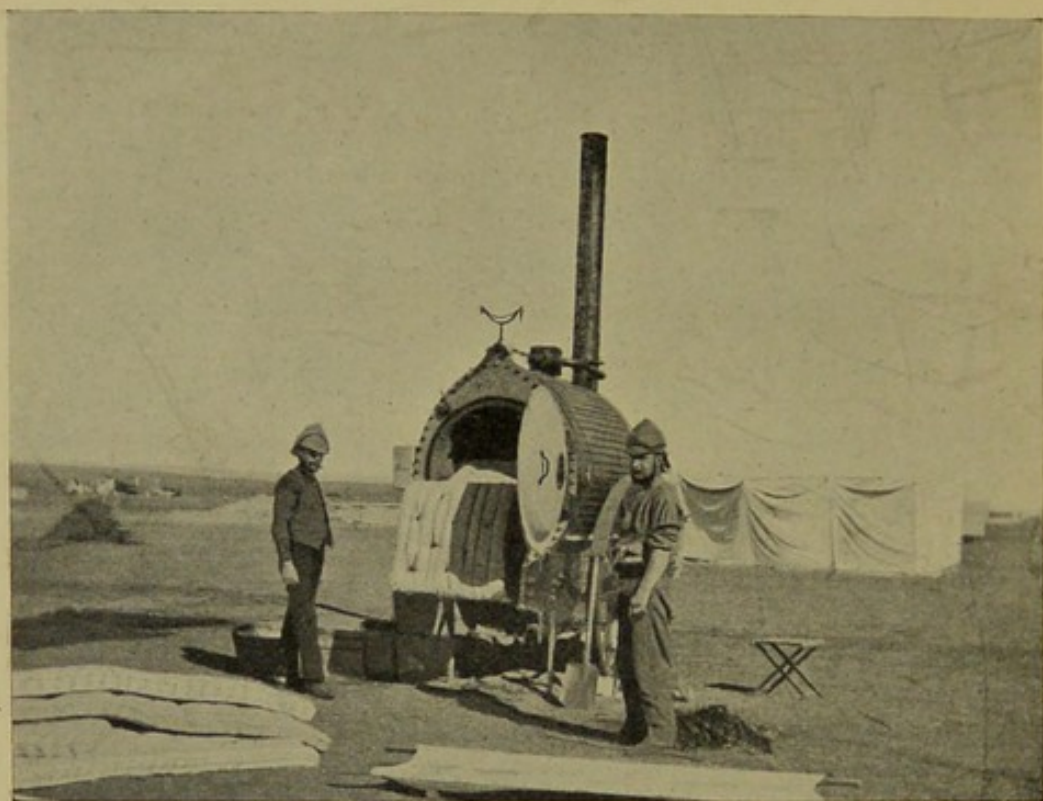
THRESH'S DISINFECTOR.
