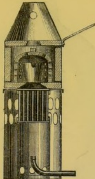
Double-jacketed furnace for operating at a white heat (section).
