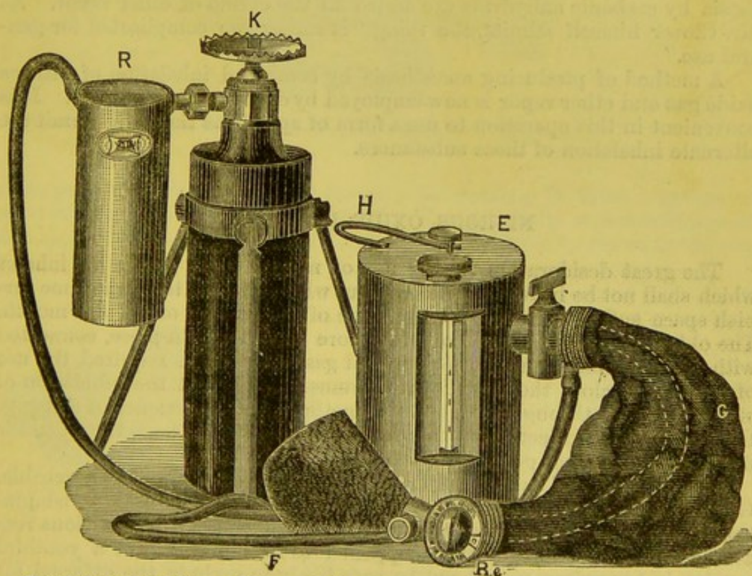
Clover's Inhaler for Ether and Nitrous Oxide: E, container for ether; F, face-piece; G, caoutchouc bag traversed by a tube, for the direct transmission of ether vapor. By a proper arrangement the vapor can be combined in the bag with nitrous oxide from the receiver R, K. Re, regulator.
