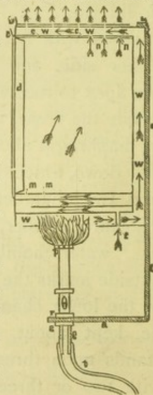
FIG. 3.—SECTION OF HOT-AIR STERILISER.
