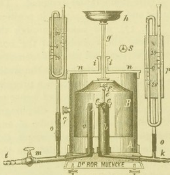
FIG. 19. MOITESSIER'S GAS-PRESSURE REGULATOR.
