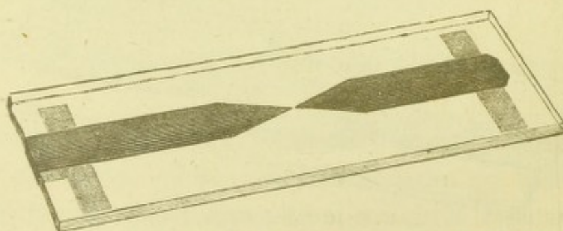
FIG. 44.—SLIDE WITH GOLD-LEAF ELECTRODES.
