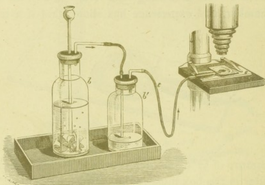
FIG. 40.—GAS CHAMBER IN USE WITH APPARATUS FOR GENERATING CARBONIC ACID.
