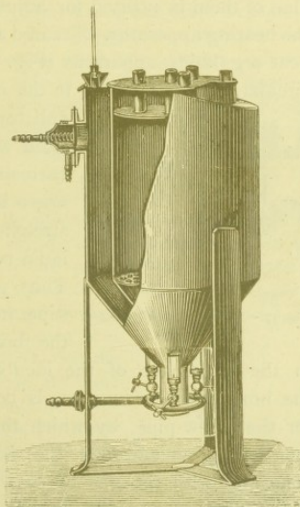
FIG. 16.—D'ARSONVAL'S INCUBATOR.
