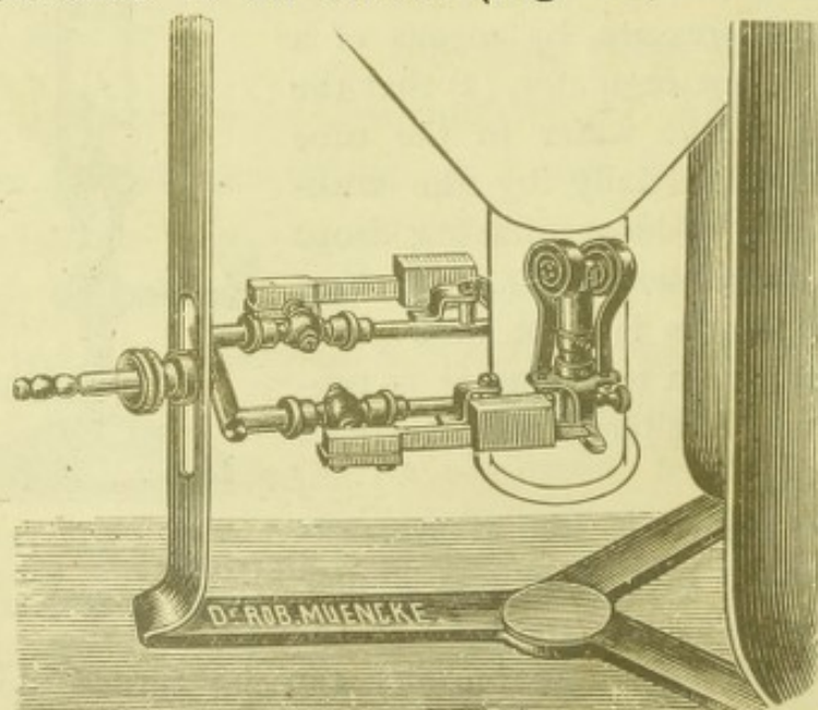
FIG. 20.—Koch's SAFETY BURNER.
