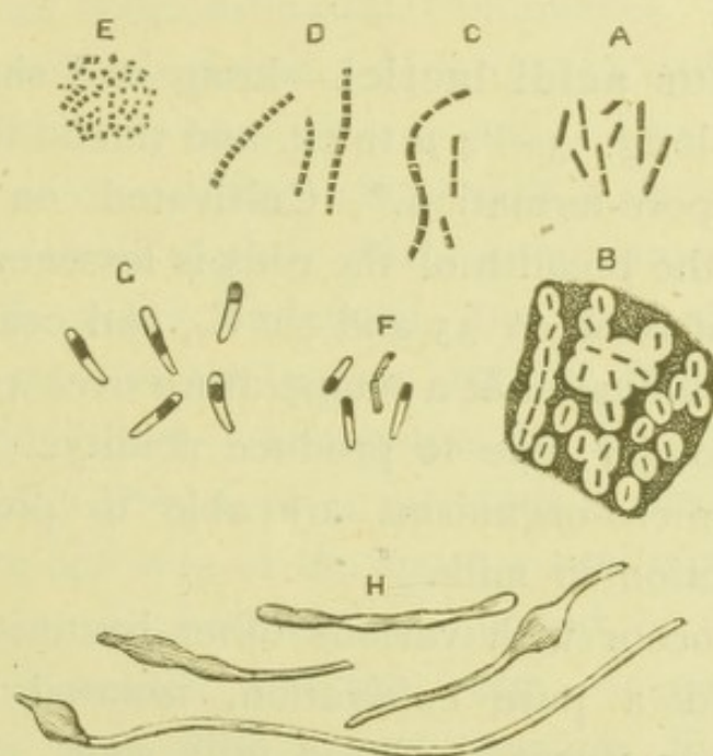
FIG. 119.— BACILLUS CYANOGENUS , \times 650 .
