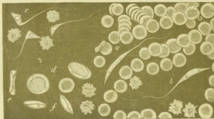
FIG. 134.—MONADS IN RAT'S BLOOD, \times 1200 .
