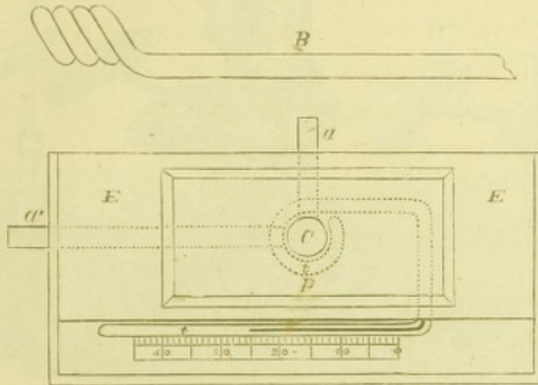
FIG. 41.—STRICKER'S COMBINED GAS CHAMBER AND WARM STAGE.
