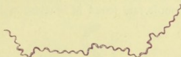
FIG. 99.— SPIRILLUM PLICATILE (Marsh Spirochæte). From sewage-contaminated water, \times 1200 .
