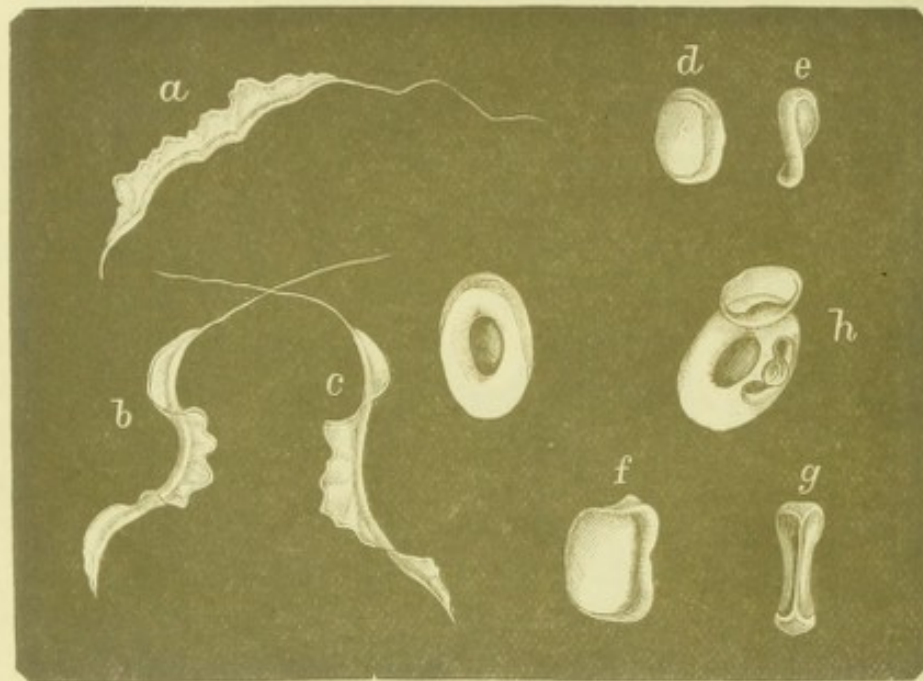
FIG. 131.—ORGANISMS IN THE BLOOD OF THE CARP.
