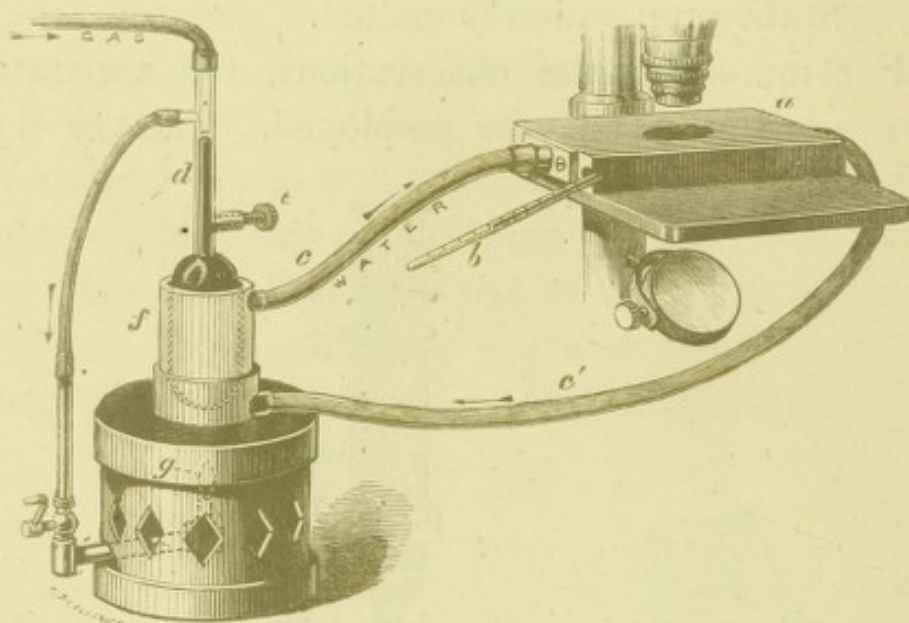
FIG. 34.—SCHÄFER'S WARM STAGE.
