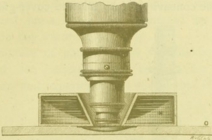
FIG. 36.—SECTION OF ISRAEL'S WARMING APPARATUS AND DROP-CULTURE SLIDE.
