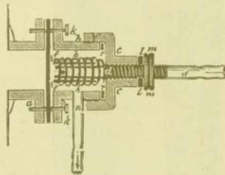
FIG. 17.—SCHLOSING'S MEMBRANE REGULATOR.
