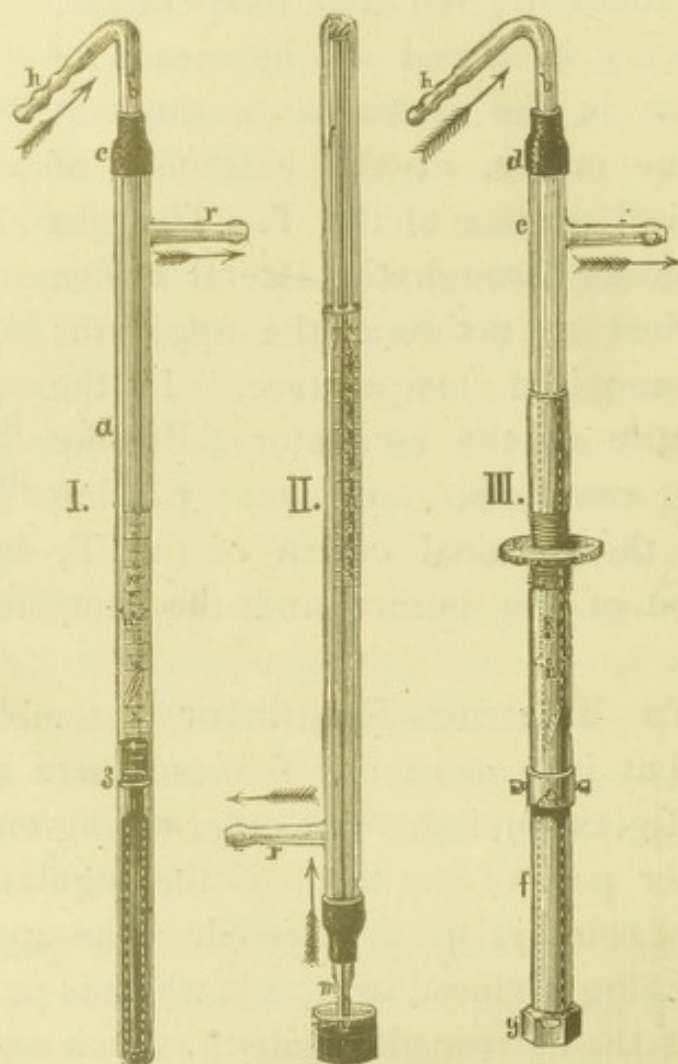
FIG. 23.—MEYER'S THERMO-REGULATOR.
