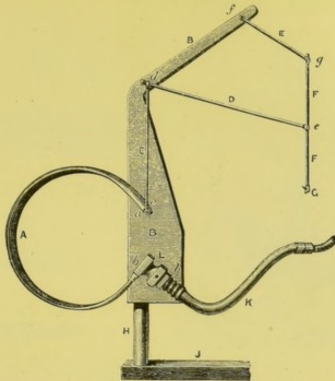
FIG. 205.—Flick's spring kymograph. A. C-spring. BB. Support. C. Rod which communicates the movements of the spring to the lever D, and thus to the writing-needle G. K. Leaden tube by which the cavity of the spring is in communication with the artery.
