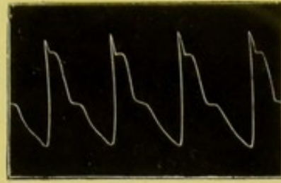
FIG. 212b.—Natural pulse.
