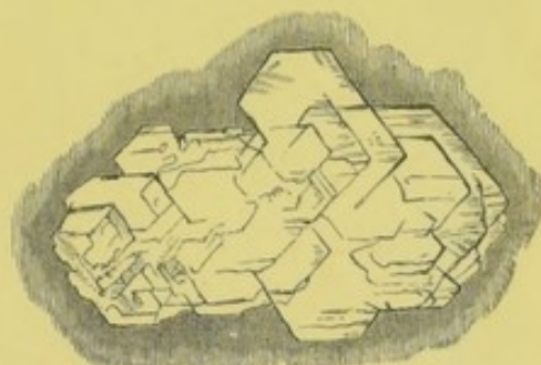
FIG. 323.—Nitrate of urea.
