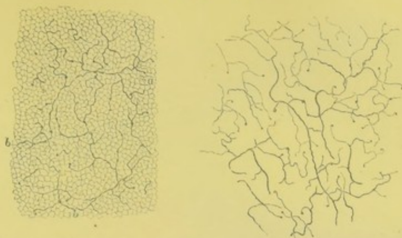
FIG. 84.—Horizontal preparation of the same kind as fig. 83, showing the deep intra-epithelial network of fine non-medullated nerve fibres viewed from the surface. a . Contours of deepest cells of anterior epithelium. b . Nerve fibres. p. 7 (Oc., 3; Obj., 7. Tube not drawn out.)
