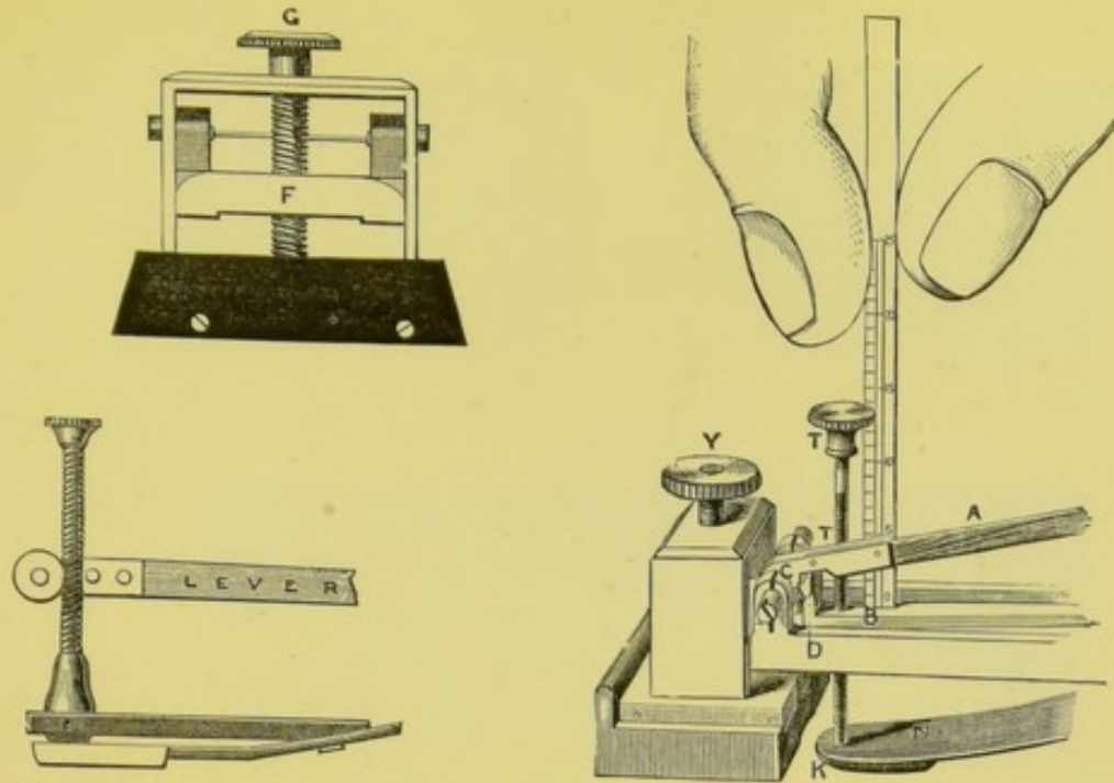
FIG. 209.—End view of the block by which the sphygmograph rests on the bones of the wrist, showing the screw, G, by which the pressure exercised by the spring on the artery can be varied (§ 39). FIG. 209b.—Breguet's improvement (§ 39).
