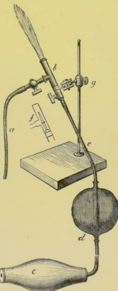
FIG. 221.—Griffin's blower and expanding regulator, as used for gas blow-pipe. The blower is used for artificial respiration (see § 49).
