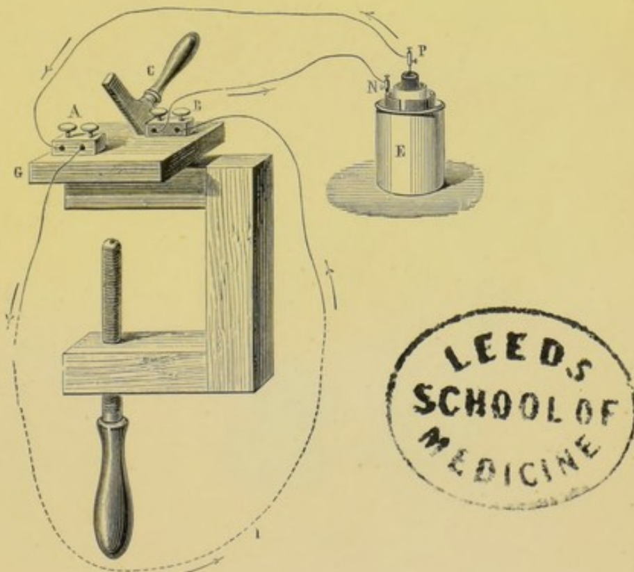
FIG. 300.—Du Bois Reymond's key.
