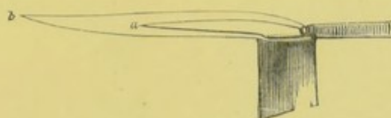
FIG. 325.—Blowpipe flame. a , reducing, b , oxidizing part of the flame.
