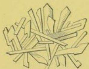
FIG. 324.—Oxalate of urea.
