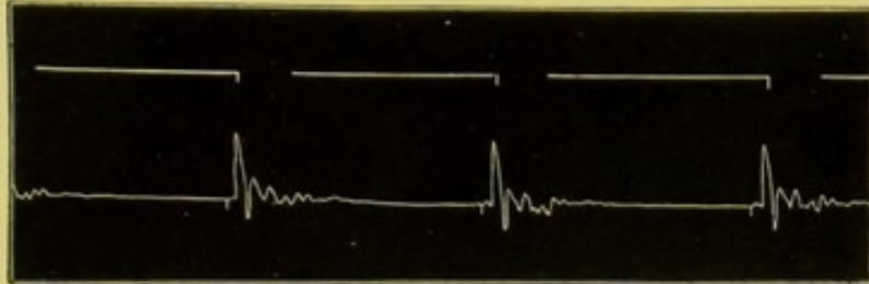
FIG. 213.—Percussion waves (§ 41.)
