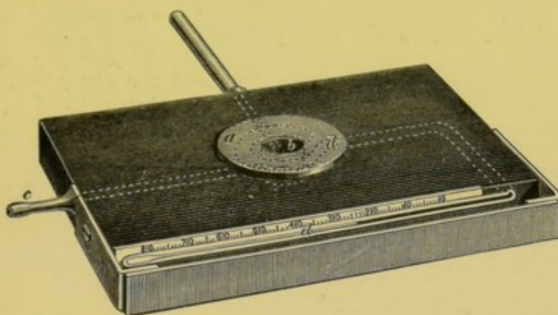
FIG. 2.—Stricker's warm stage (simple form). It consists of a block of black vulcanite about 3 inches long by 1½ wide, and ¼ inch thick. The central chamber ( b ) is closed below by a glass plate, and surrounded at the top by a perforated copper dish ( a ), the orifice of which is of the same size as the chamber. The chamber is cylindrical. The cistern of the thermometer surrounds the chamber, as shown by the dotted line ( d ). Its capillary tube lies in a trough, one side of which is formed by the back of the block and the other by a metal plate screwed on to it, the form of which is shown in the figure. The tube ( c ) leads into the chamber. A second tube leads from it through the projecting metallic arm shown at the top of the figure. This arm, which is of one piece with the disk ( a ), is of such size that the rod, fig. 13, fits on to it. By means of this rod the chamber is heated in the way already explained. In experiments with gases the gas enters by c and passes out through the projecting arm. p. 14.
