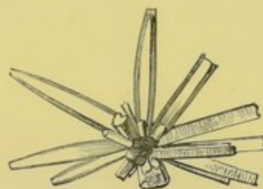
FIG. 303.—Nitrate of hypoxanthine.
