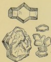
FIG. 304.—Hydrochlorate of xanthine.
