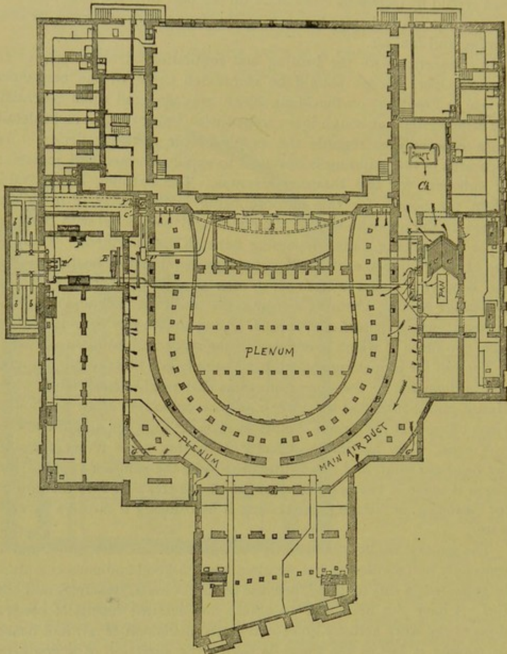
FIGURE 33.—METROPOLITAN OPERA HOUSE, NEW YORK CITY.—GROUND PLAN.
