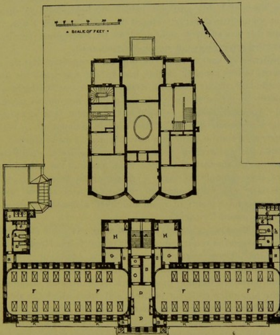
FIGURE 59.—NEW YORK HOSPITAL BUILDINGS.—PLAN OF SECOND, THIRD AND FOURTH STORIES.
