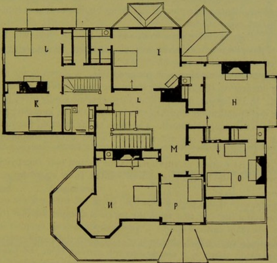
FIGURE 8.—SECOND FLOOR PLAN OF SUBURBAN HOUSE.—(See page 64.)
