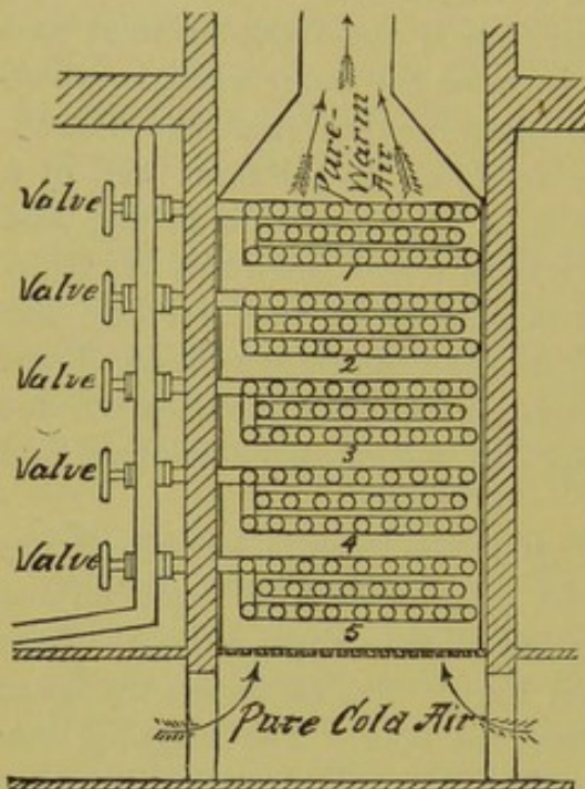
FIGURE 49.—VERTICAL SECTION OF COIL CHAMBER.
