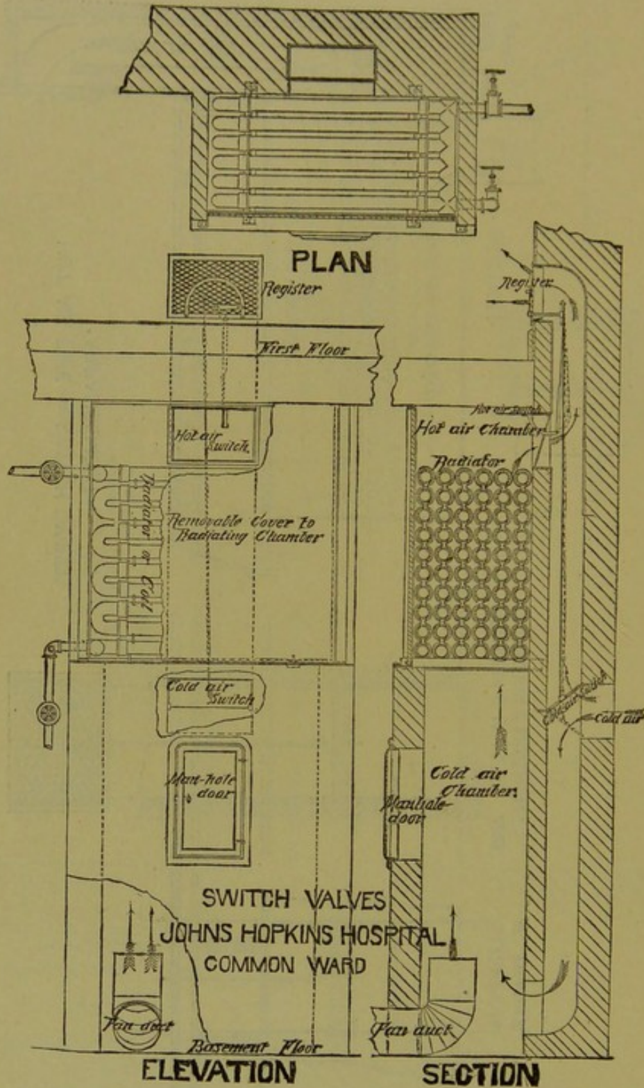
FIGURE 69.—HEATING COILS AND SWITCH VALVES.—JOHNS HOPKINS HOSPITAL.
