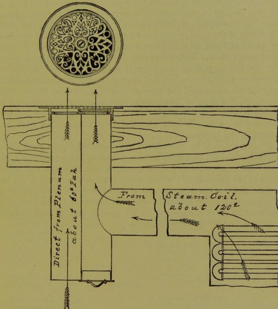
FIGURE 72.—PLAN AND SECTION OF MIXING REGISTER.
