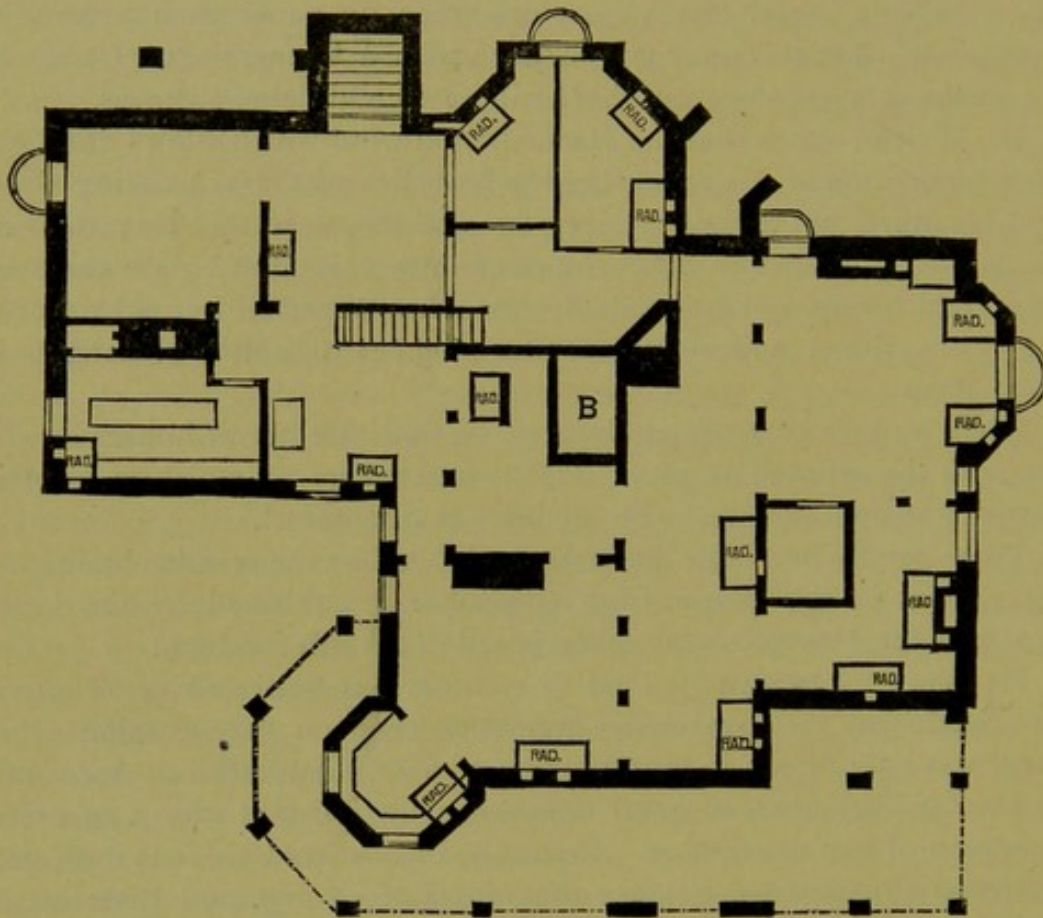
FIGURE 3.—CELLAR PLAN OF SUBURBAN RESIDENCE.—(See page 64.)
