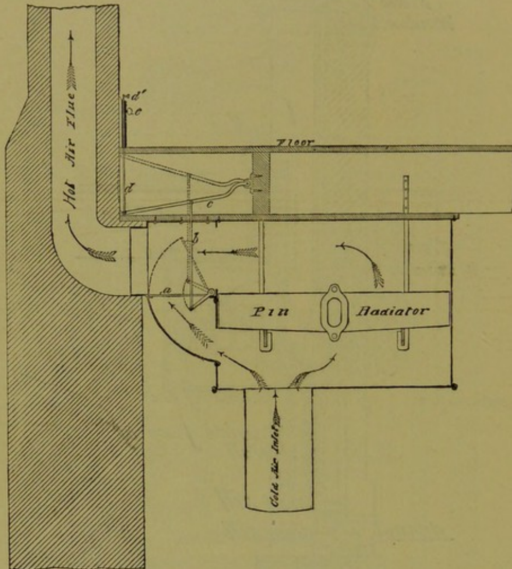
FIGURE 71.—DETAIL OF MIXING VALVE.
