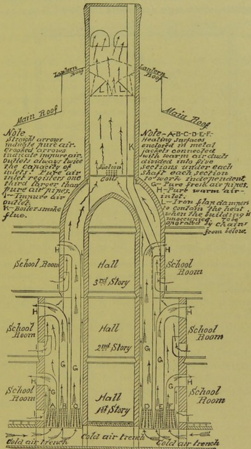
FIGURE 50.—VERTICAL SECTION OF SCHOOL BUILDING.
