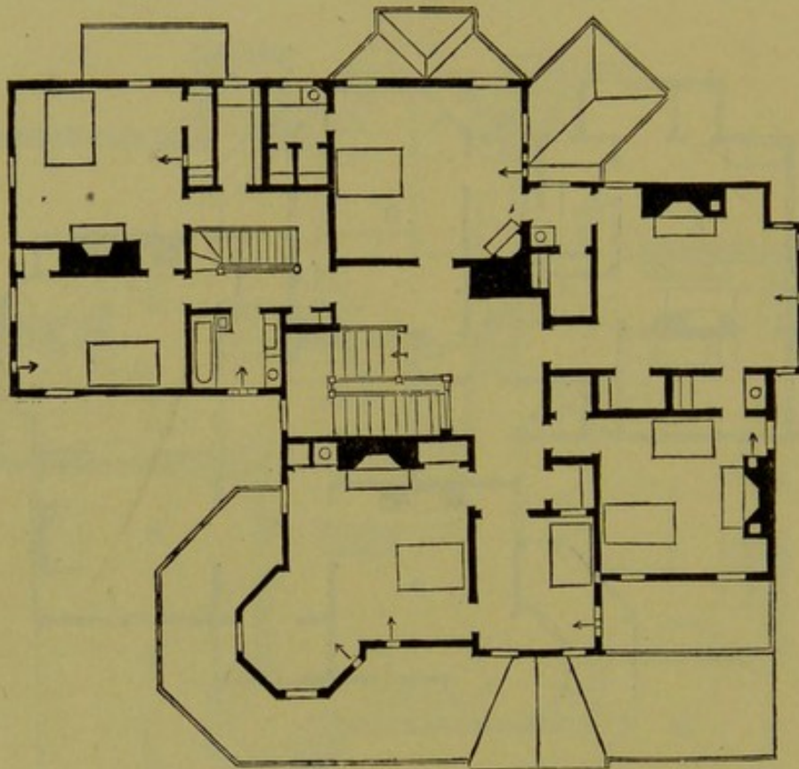
FIGURE 5.—SECOND STORY PLAN OF SUBURBAN RESIDENCE.—(See page 64.
