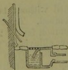
Fig. 85.—Pipes opening above Grating and Trap.
