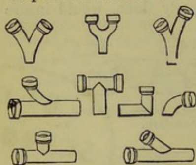
Fig. 80.—Junctions.
