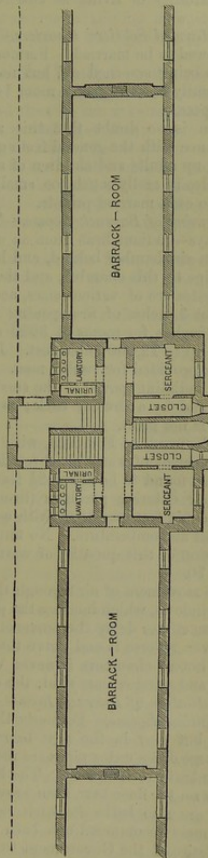
Fig. 100.—New Chelsea Barracks.
