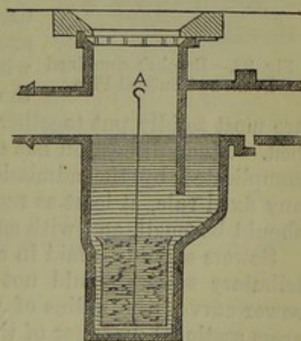
Fig. 91.—Dean's Gully Trap. A Handle of movable bucket.
