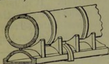
Fig. 92.—Brooks's combined Drain and Subsoil Pipe.
