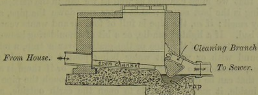
Fig. 88.—Longitudinal Section.
