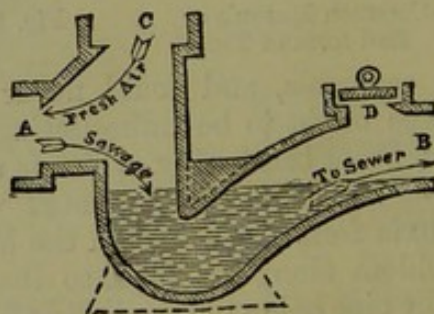
Fig. 86.—Disconnecting and Ventilating Drain Trap, No. 2, Buchan's Patent.
