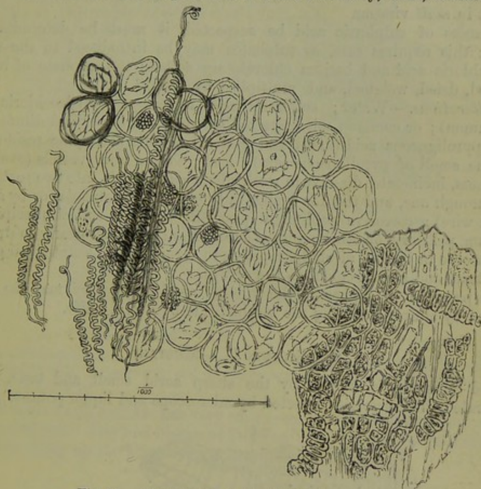
Fig. 63.—Cocoa, Under Parts, Middle Coat \times 190 .
