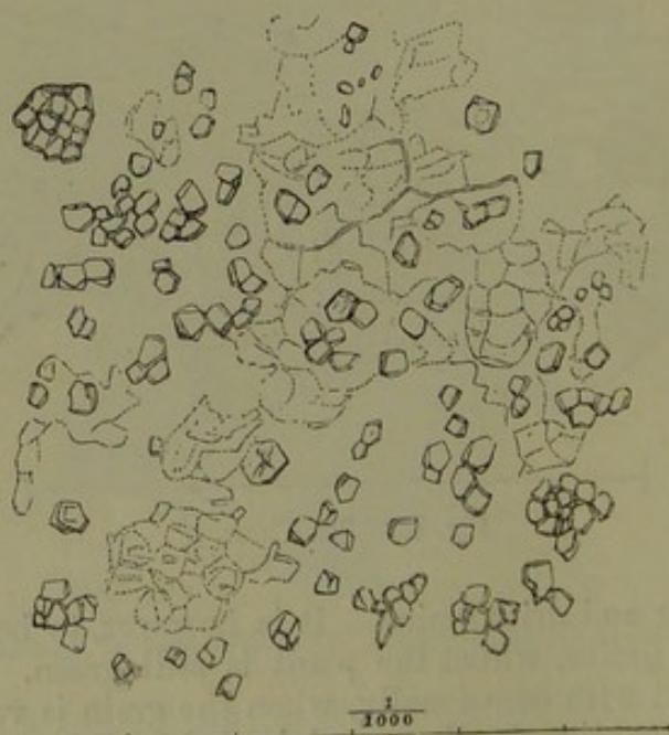
Fig. 48.—Ground Rice Flour \times 350 .
