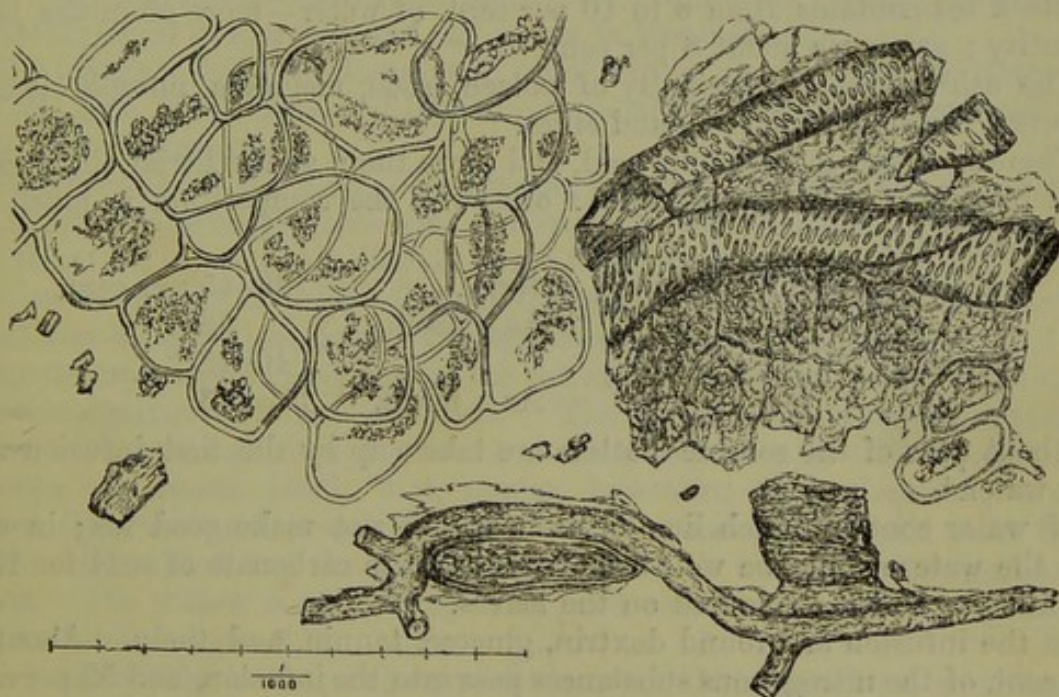
Fig. 60.—Chicory root; cells and dotted ducts.
