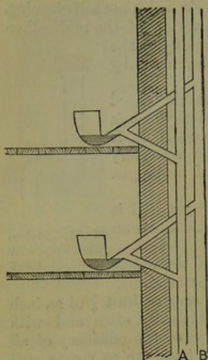
Fig. 84.—Siphon Closet Basins with ventilating pipes. A, Soil pipe passing up above the eaves, with open top. B, Subsidiary Ventilating Pipe (also passing up above eaves with open top) to prevent sucking of the siphon.
