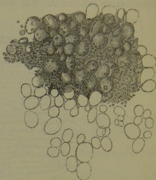
Fig. 29.—Fresh Starch-grains of Wheat (moistened). × 360.
