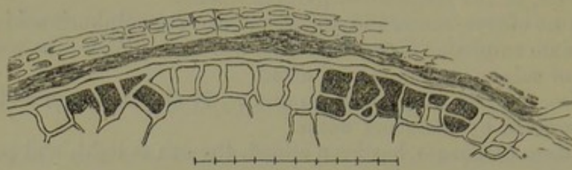
Fig. 23.—Transverse Section of Envelopes of Wheat. Scale 1000th of an inch.
