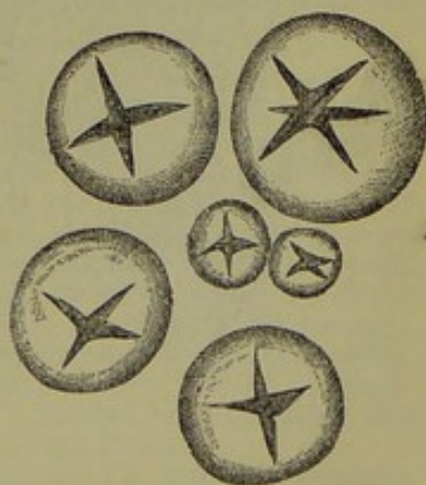
Fig. 51.—Rye-starch, with rayed hilum (after Hassall) \times 420 .
