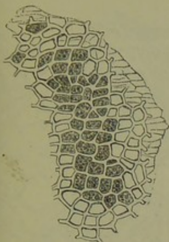
Fig. 39.—Barley (fourth coat).
