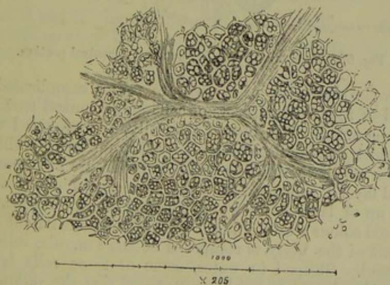
Fig. 66.—White Mustard Seed, central part, \times 205 .
