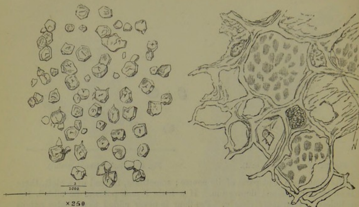
Fig. 43.—Indian-Corn Flour. See also Plate of Starches.
