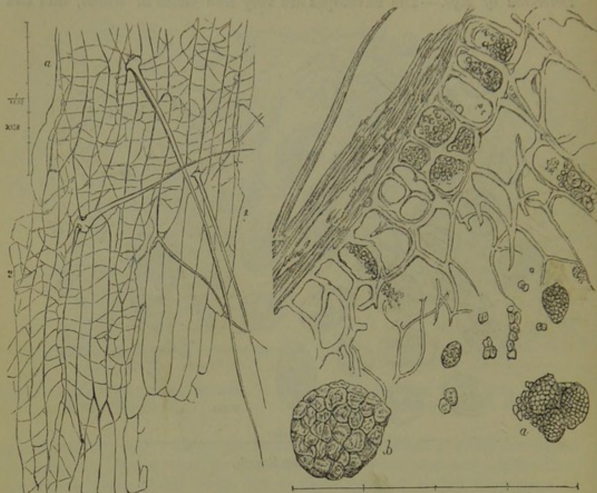
Fig. 47.—White Oat (long. sect., 2nd and 3rd coats not separable). a Compound grains \times 100 . b One do. \times 500 .
