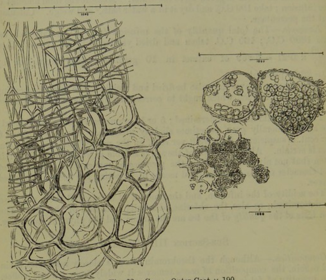
Fig. 62.—Cocoa, Outer Coat \times 190 .
