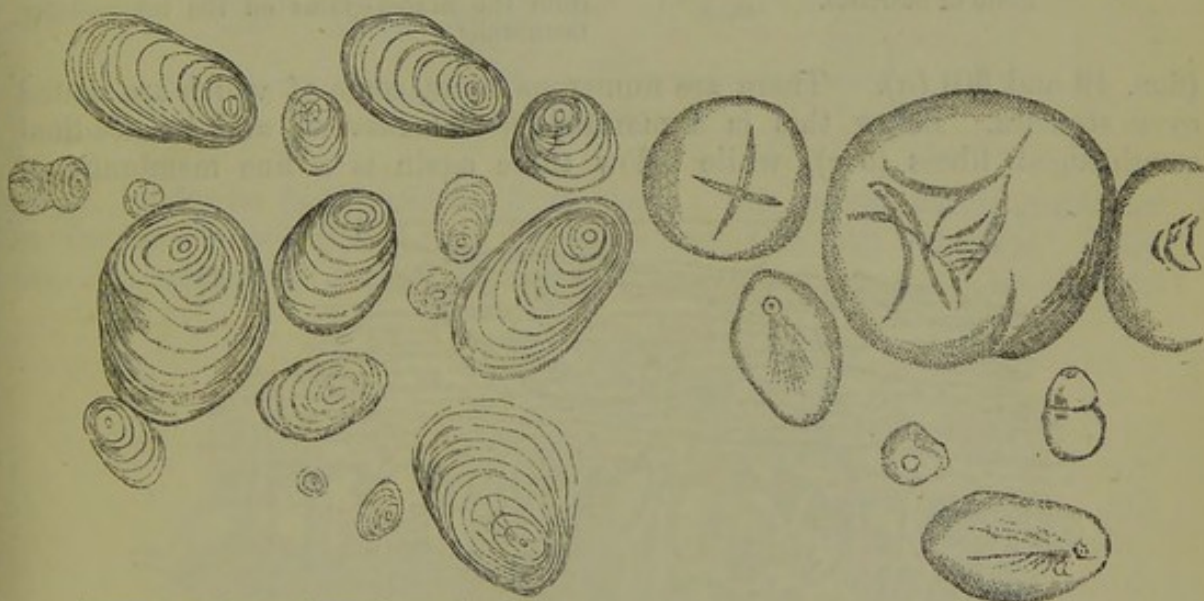
Fig. 42.—Medium and small-sized Potato Starch-grains, treated with Liq. Pot. B.P. (strength 1 to 3), and \times 285 .
