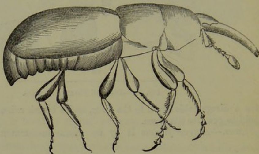
Fig. 34.—Weevil. Magnified 12 diameters.
