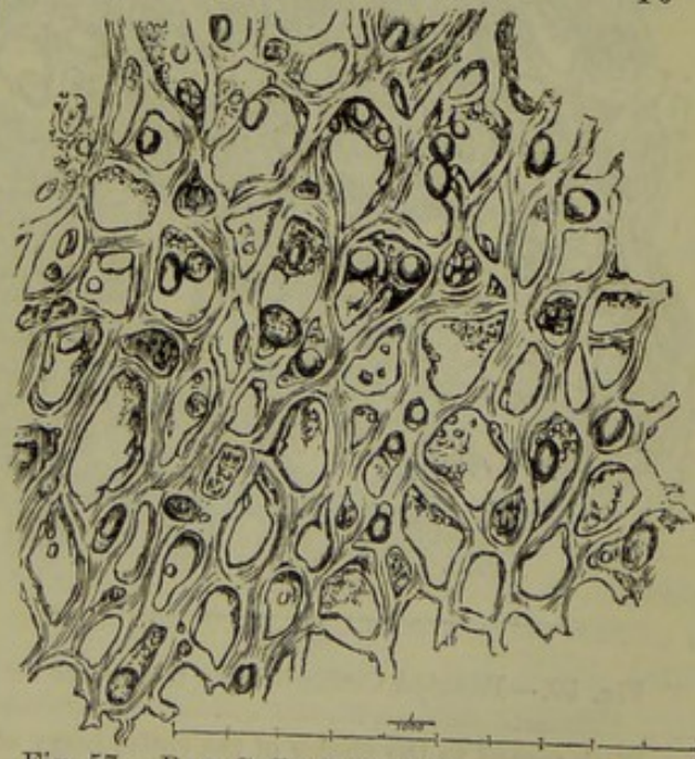
Fig. 57.—Raw Coffee-berry; transverse section \times 170 .
