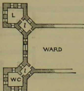
Fig. 72.—Closets (W.C.) and Lavatory (L) with intervening ventilated lobbies (I).
