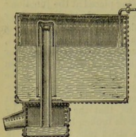
Fig. 79.—Field's Flush Tank.
