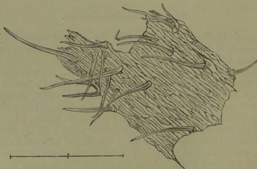
Fig. 25.—Outer Coat and Hairs of Wheat. Scale 100th of an inch.
