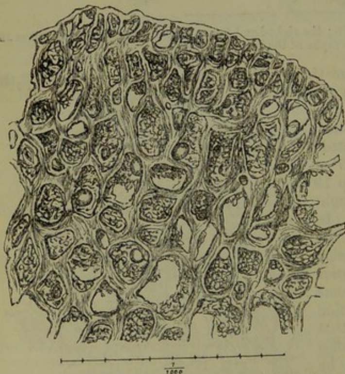
Fig. 59.—Roasted Coffee-berry; transverse section.
