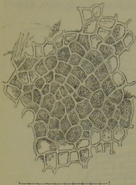
Fig. 28.—Fourth Envelope of Wheat. Scale 1000th of an inch.
