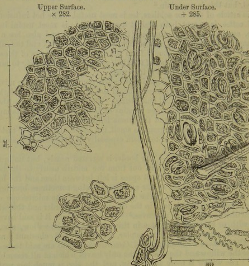
Fig. 61.—Dried Black Tea Leaf.
