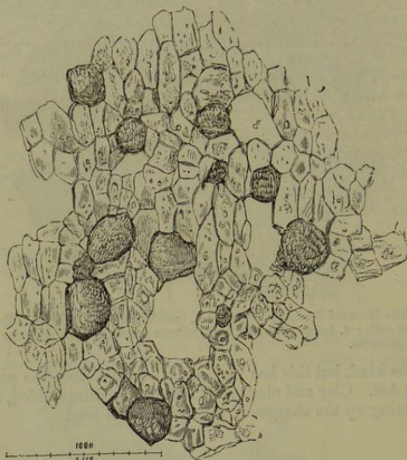
Fig. 67.—Section of Black Pepper Berry, central portion.
