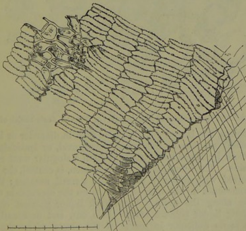
Fig. 27.—Second and Third Envelopes of Wheat. Scale 1000th of an inch.
