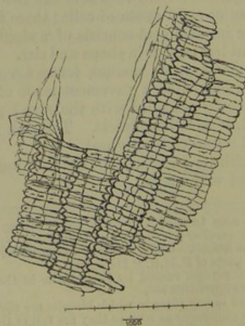
Fig. 38.—Barley (second and third coats).
