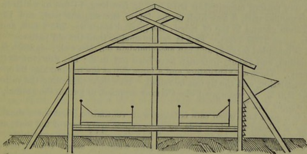
Fig. 102.—Plan of German Shed.
