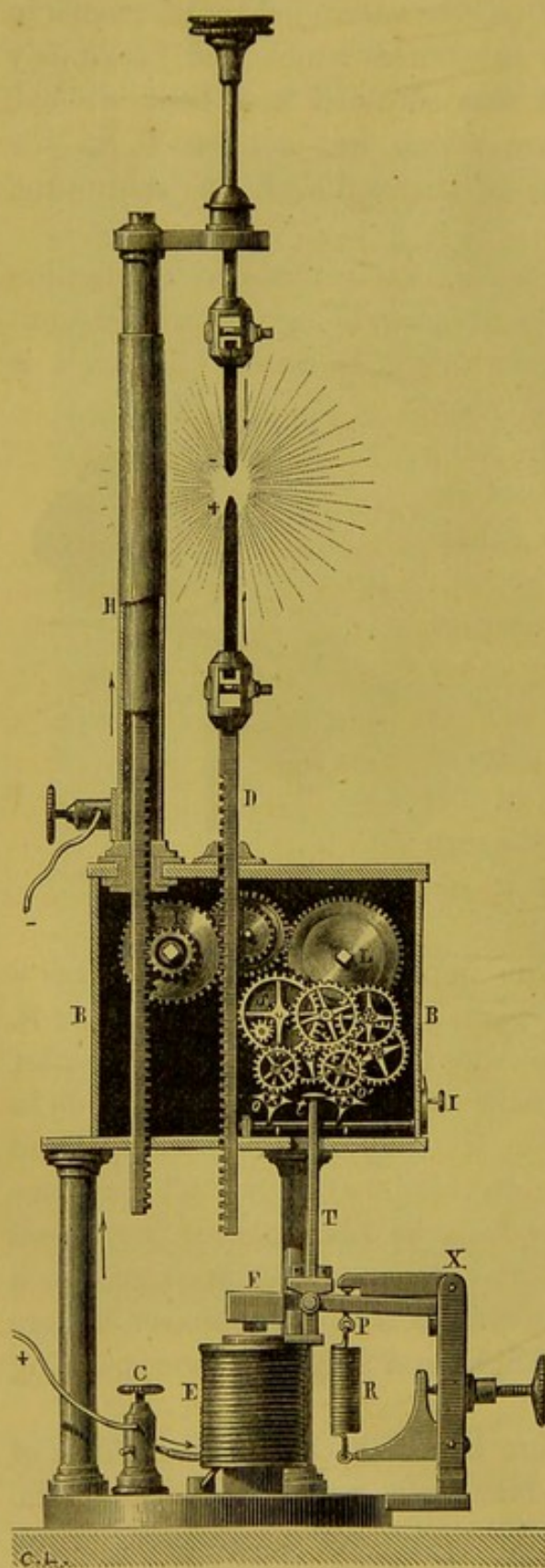
Fig. 590.—Foucault's Regulator.
