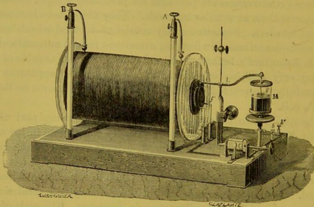
Fig. 536.—Ruhmkorff's Coil.
