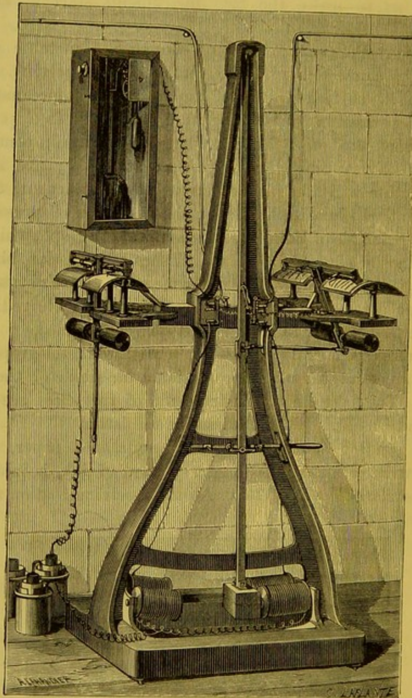
Fig. 574.—Caselli's Telegraph.
