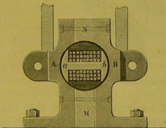
Fig. 546.—Section of Siemens' Armature.
