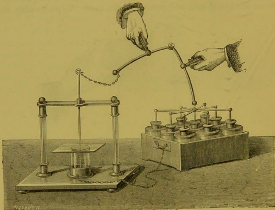
Fig. 398.—Puncture of Glass.
