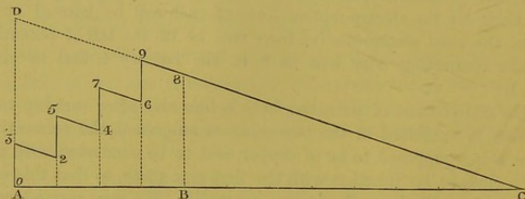
Fig. 485.—Curve of Potential for Closed Circuit.
