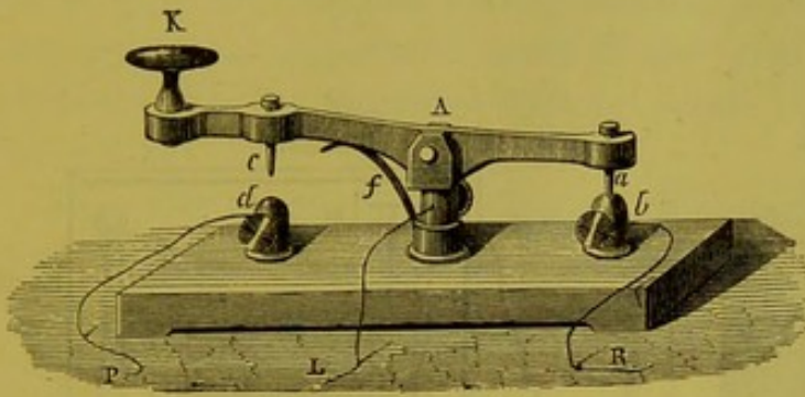
Fig. 568.—Morse's Key.
