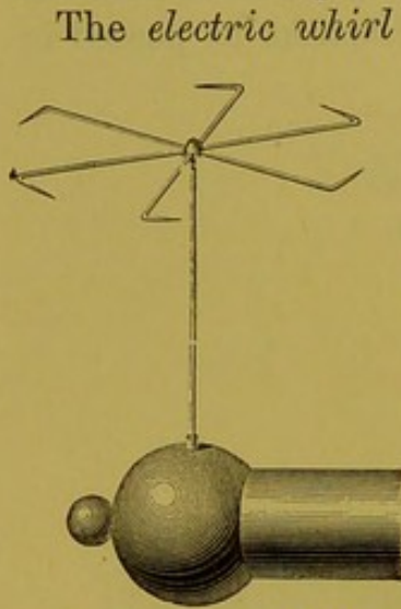
Fig. 375.—Electric Whirl.
