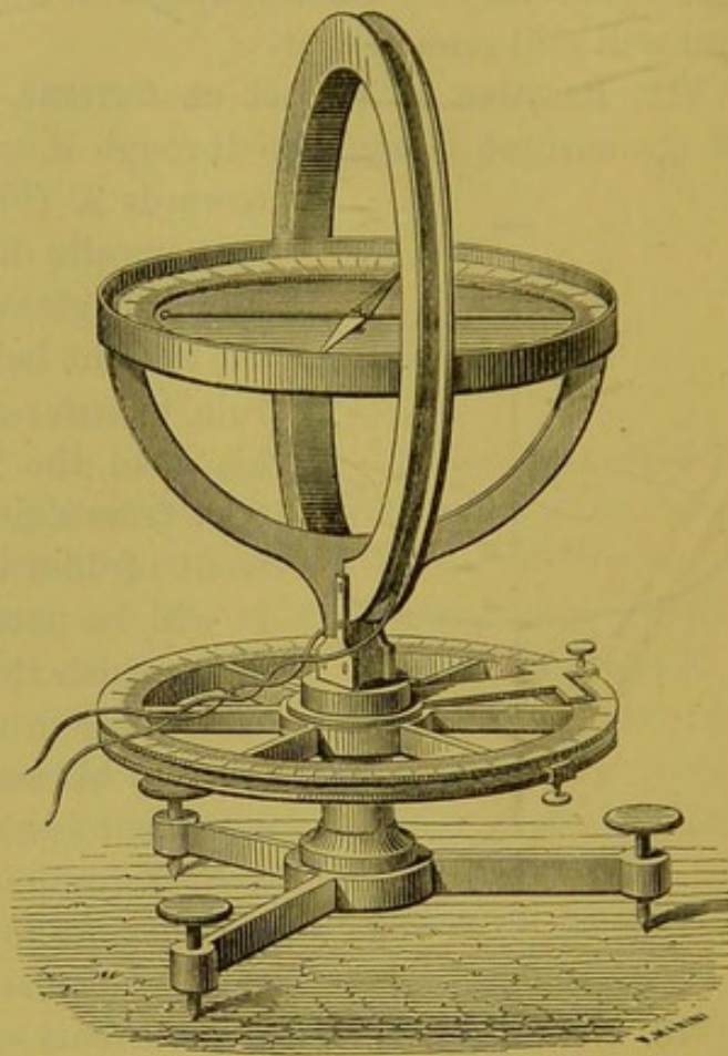
Fig. 464.—Sine Galvanometer.
