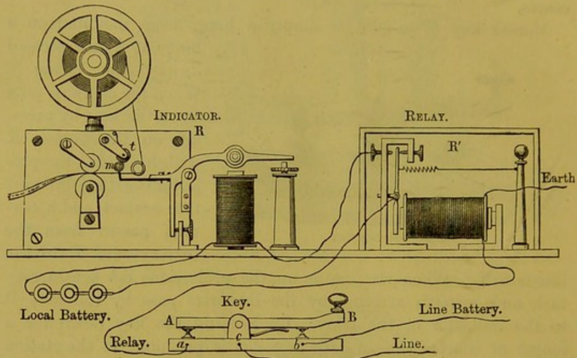
Fig. 569.—Morse's Apparatus, with Relay.
