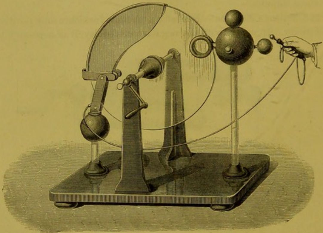
Fig. 354.—Winter's Electrical Machine.
