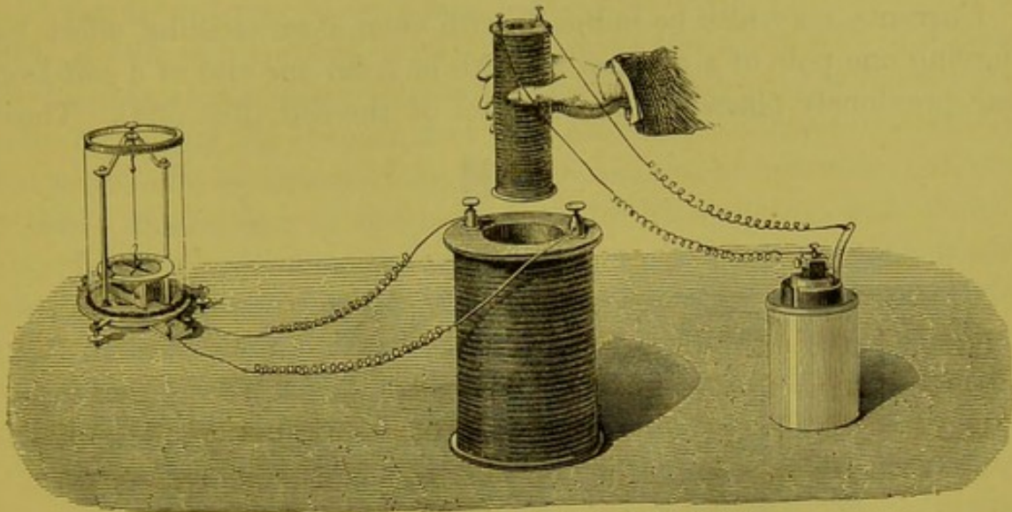
Fig. 532.—Current induced by Change of Distance.
