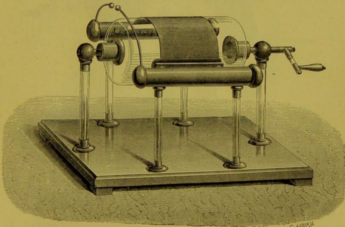
Fig. 353.—Nairne's Electrical Machine.
