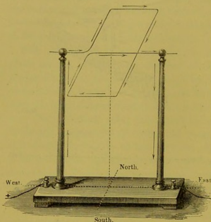
Fig. 517.—Dip of Element of Solenoid.
