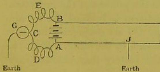
Fig. 489.—Loop Test.
