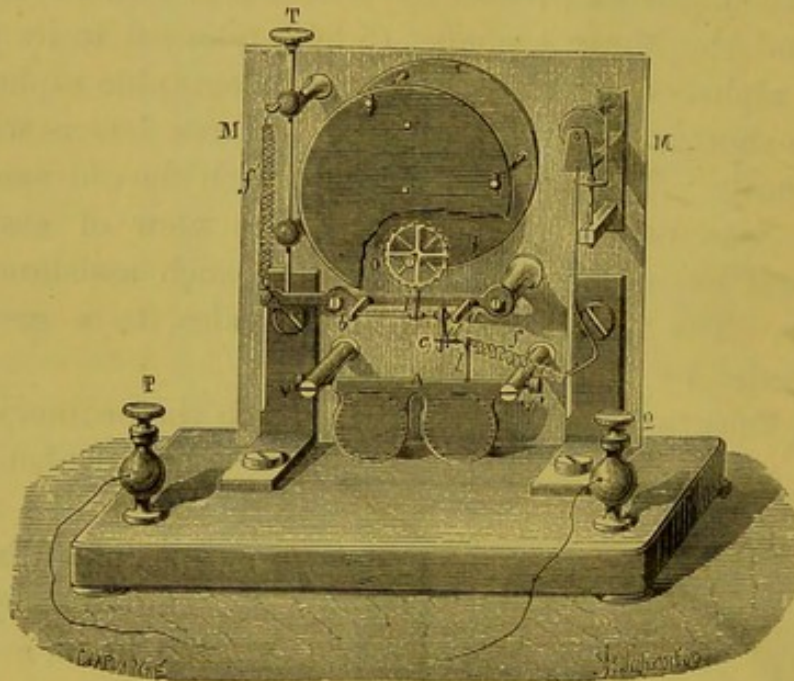
Fig. 562.—Mechanism of Indicator.
