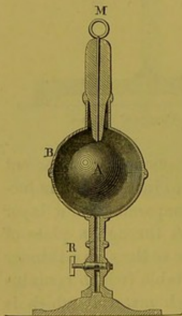
Fig. 387.—Apparatus for Specific Inductive Capacity.
