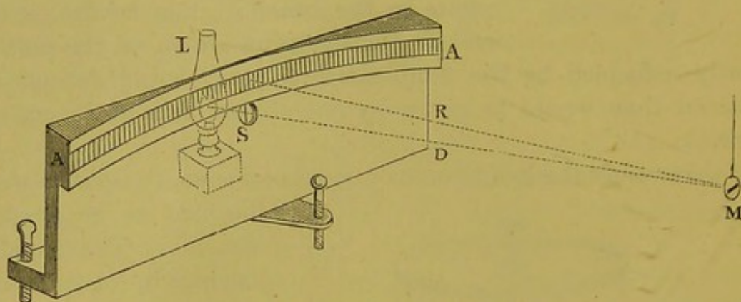
Fig. 470.—Mirror and Scale.
