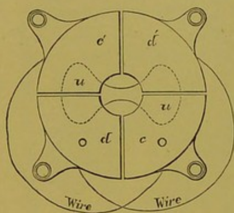
Fig. 403.—Needle and Quadrants.
