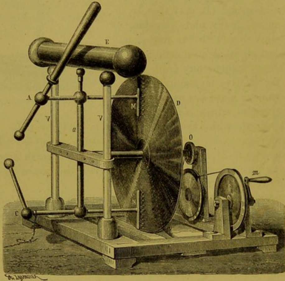
Fig. 360.—Bertsch's Electrical Machine.
