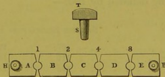
Fig. 481.—Mode of Connecting Resistance Coils.
