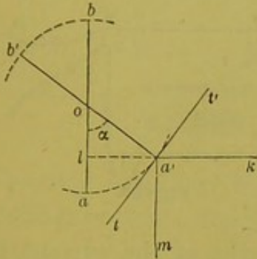
Fig. 465.—Principle of Tangent Galvanometer.
