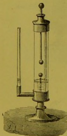
Fig. 371.—Kinnersley's Thermometer.
