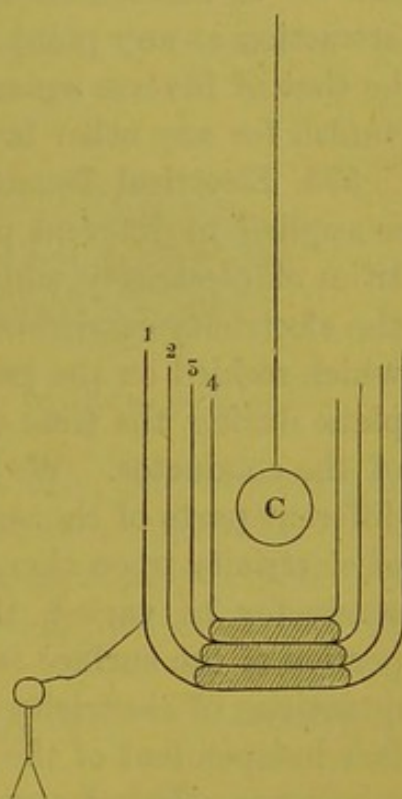
Fig. 345.—Experiment with Four Ice-pails.
