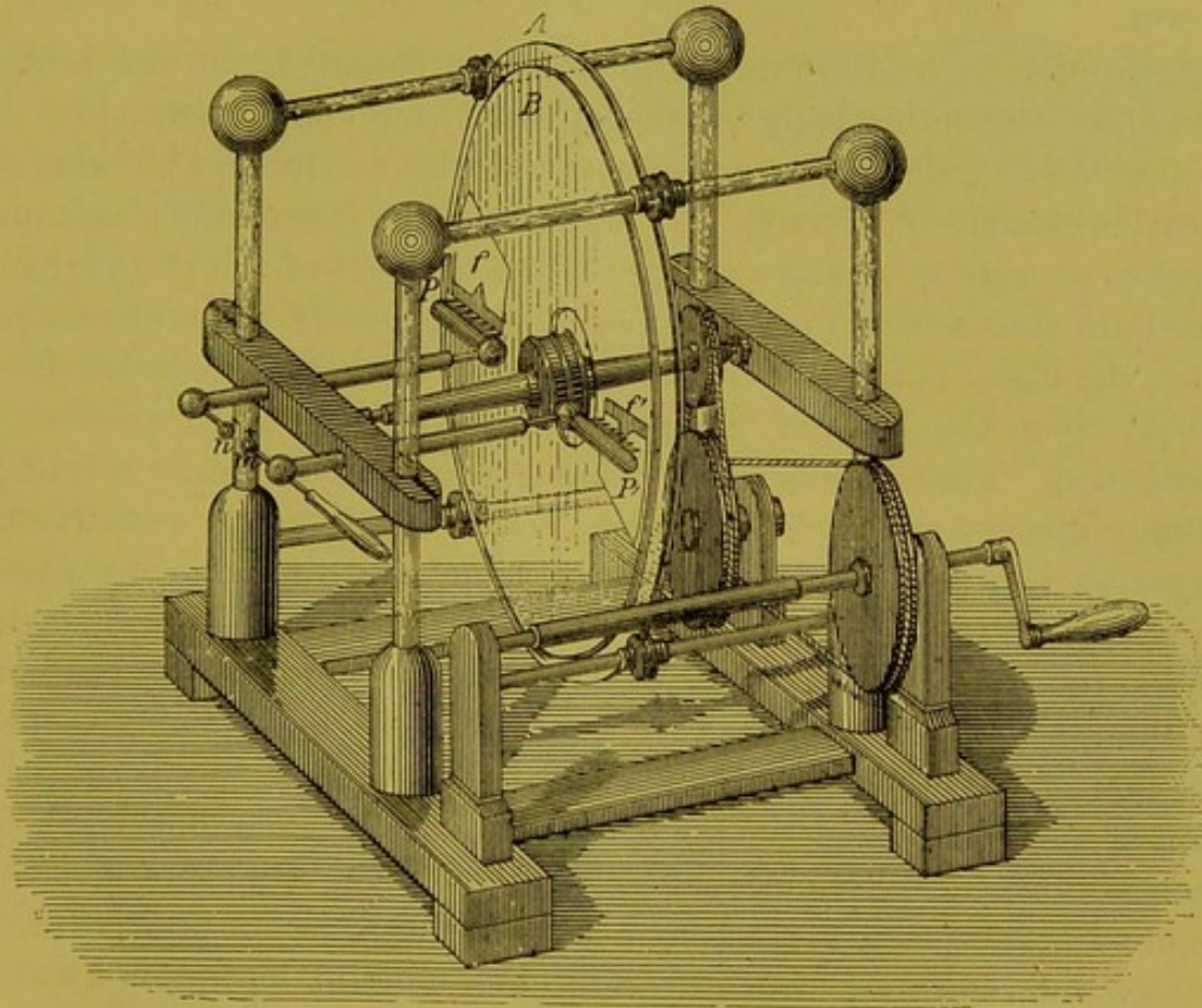
Fig. 357.—Holtz's Electrical Machine.
