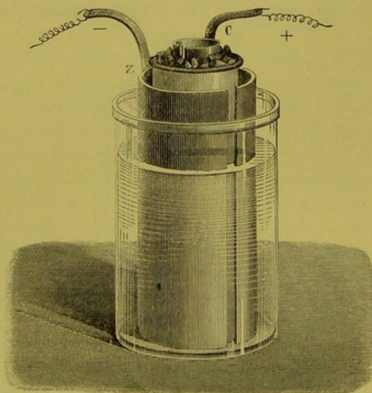
Fig. 456.—Daniell's Cell.
