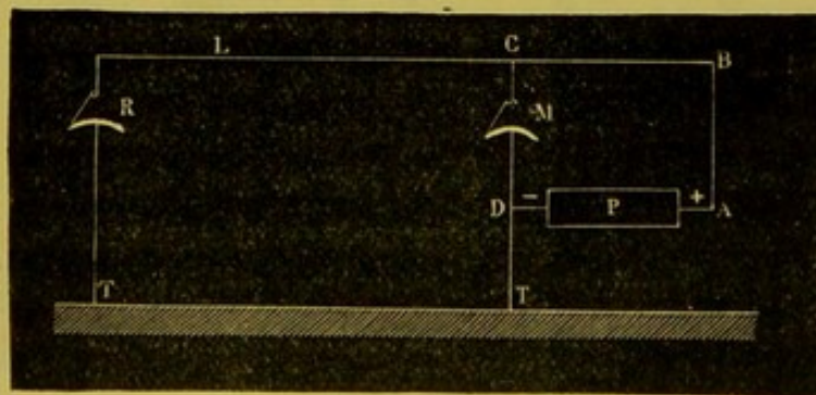
Fig. 573.—Principle of Caselli's Telegraph.
