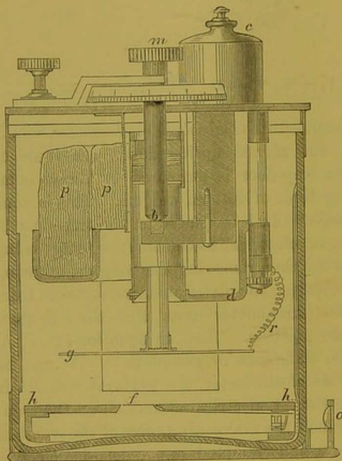
Fig. 400.—Portable Electrometer.
