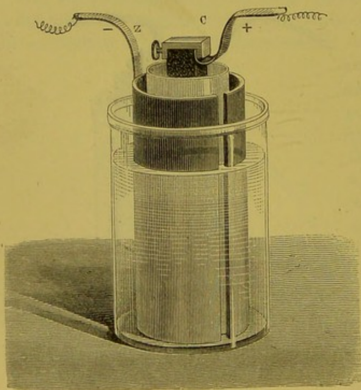
Fig. 457. — Bunsen's Cell.
