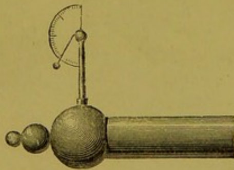
Fig. 352 — Quadrant Electroscope.
