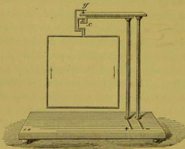
Fig. 498.—Ampère's Stand.
