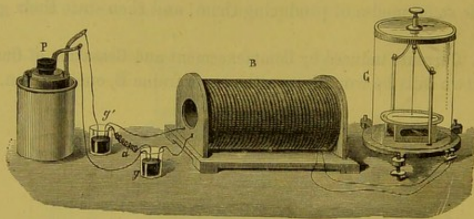
Fig. 531.—Current induced by Change of Strength.
