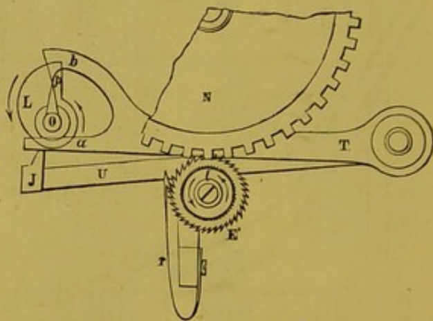
Fig. 572.—Mechanism for Printing.
