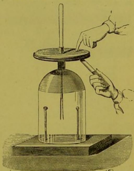
Fig. 389.—Condensing Electroscope.
