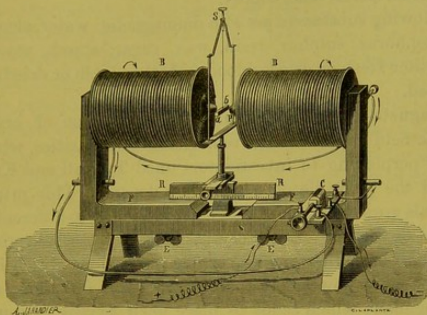
Fig. 445. — Apparatus for Diamagnetism.
