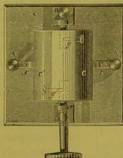
Fig. 537.—Commutator.
