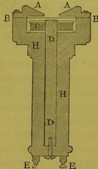
Fig. 585.—Section of Telephone.
