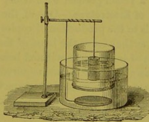
Fig. 477.—Bath and Battery in one.
