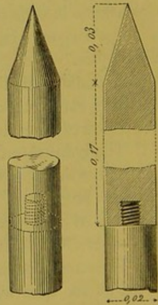
Fig. 410.—Gilded Copper Point.
