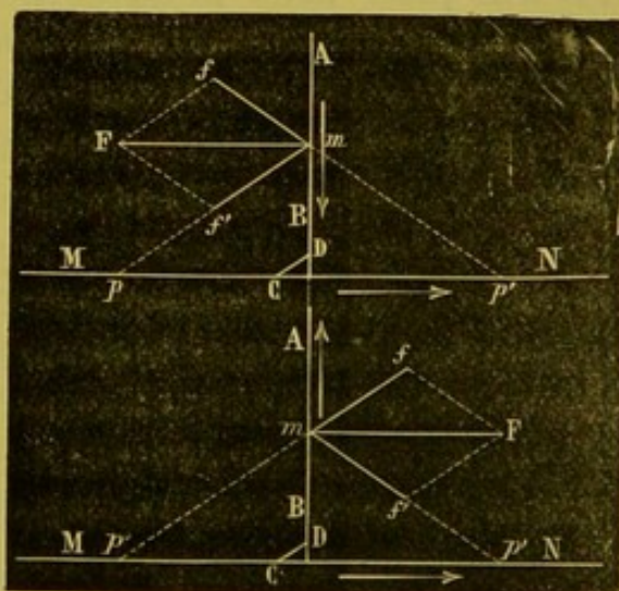
Fig. 508.—Translation Parallel to Indefinite Current.
