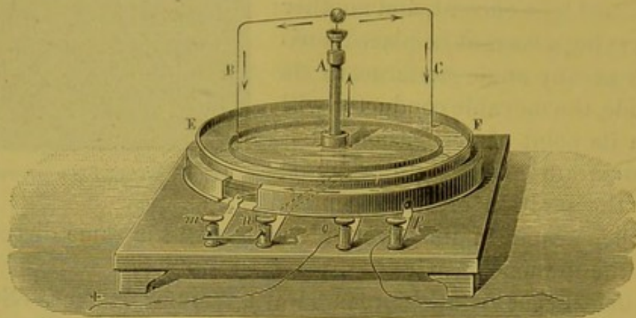
Fig. 506.—Apparatus for Continuous Rotation.
