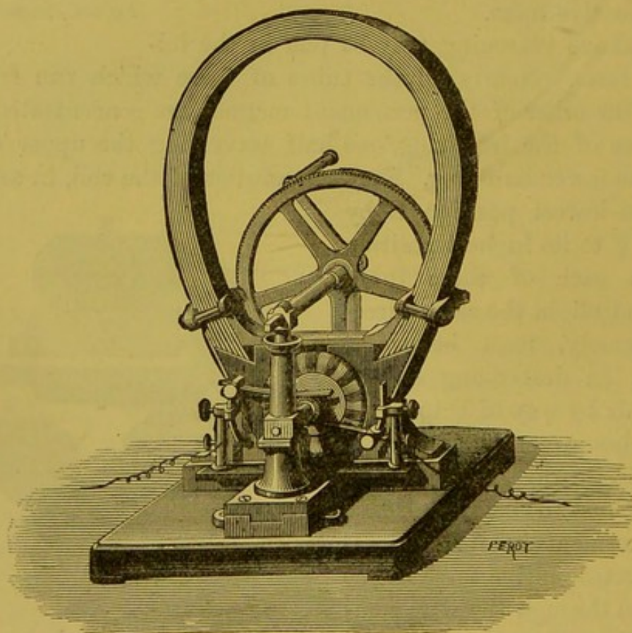
Fig. 554.—Gramme's Magneto-electric Machine, for hand-power.
