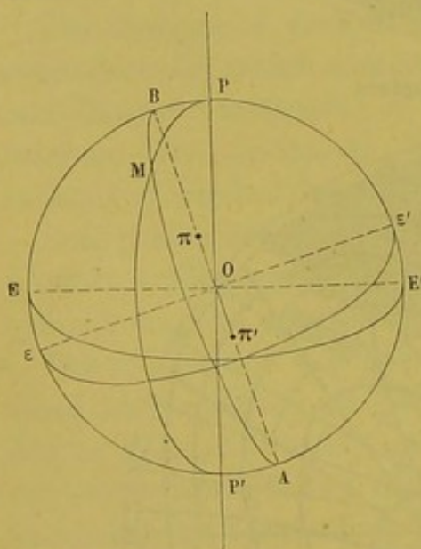
Fig. 433.—Biot's Hypothesis.
