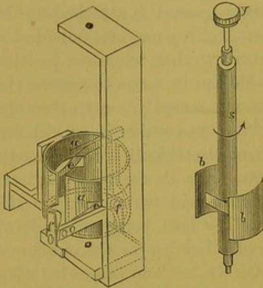
Fig. 404.—Replenisher.
