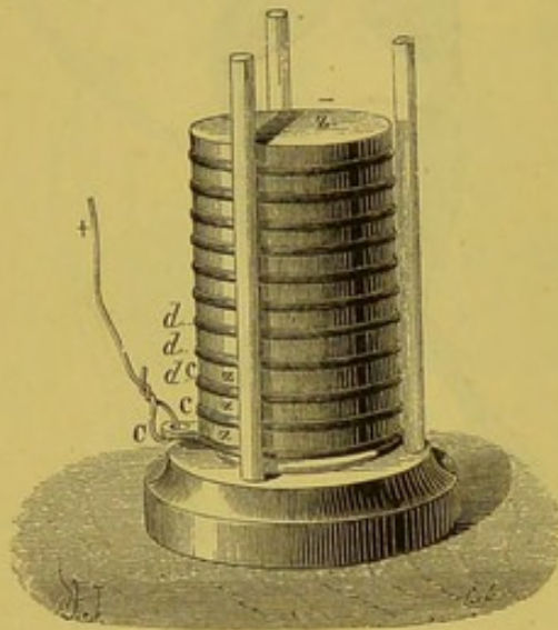
Fig. 449.—Structure of Pile.
