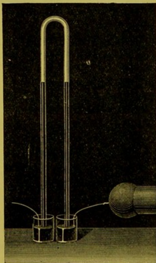
Fig. 365.—Discharge in Torricellian Vacuum.
