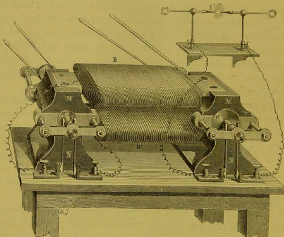
Fig. 549.—Ladd's Machine.
