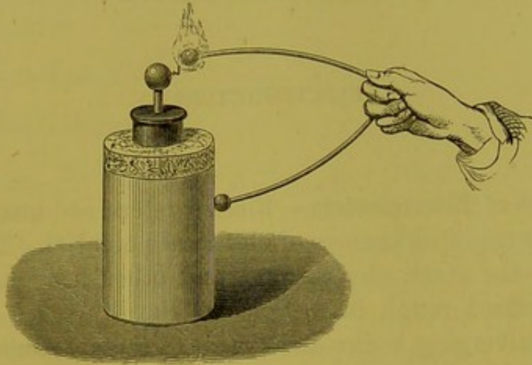
Fig. 399.—Gun-cotton Fired.
