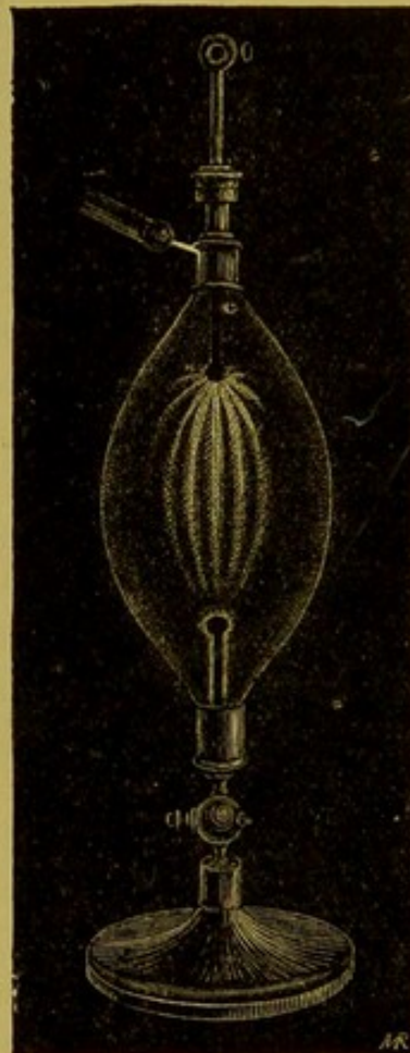
Fig. 364.—Spark in Rarefied Air.
