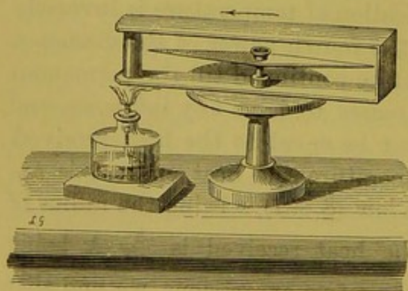
Fig. 493.—Thermo-electric Current.
