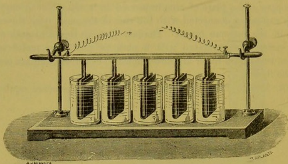
Fig. 454.—Wollaston's Battery.
