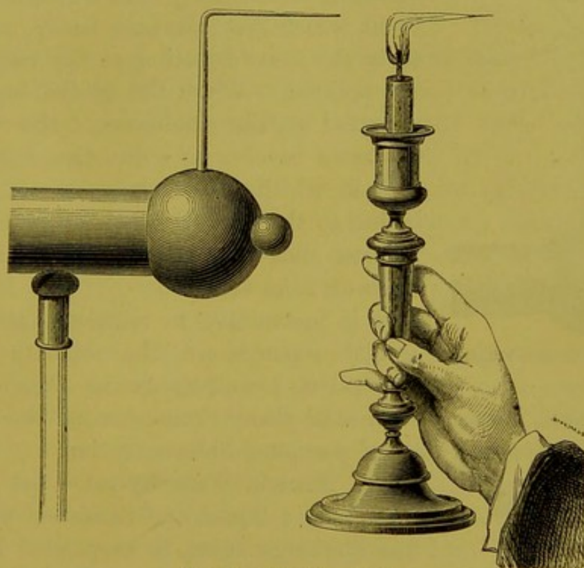
Fig. 374. — Wind from Points.
