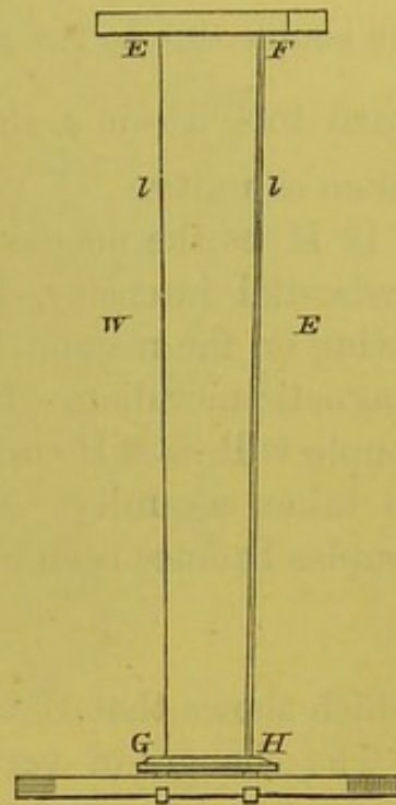
Fig. 429.—Bifilar Magnetometer.
