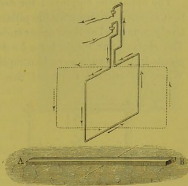
Fig. 499.—Action of Magnet on Movable Circuit.
