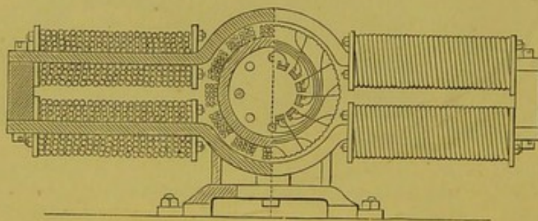
Fig. 551. —Section of Siemens' Machine.
