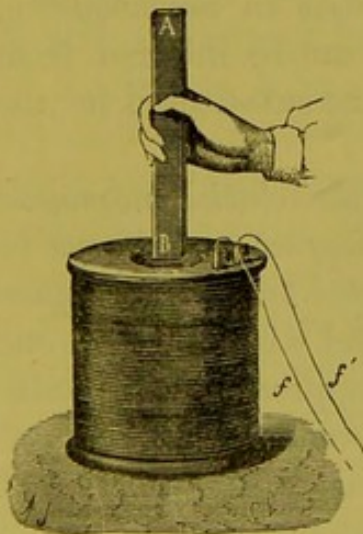
Fig. 533.—Current induced by Motion of Magnet.
