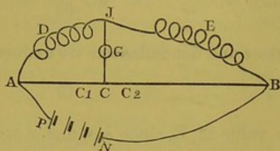
Fig. 488.—Wheatstone's Bridge.
