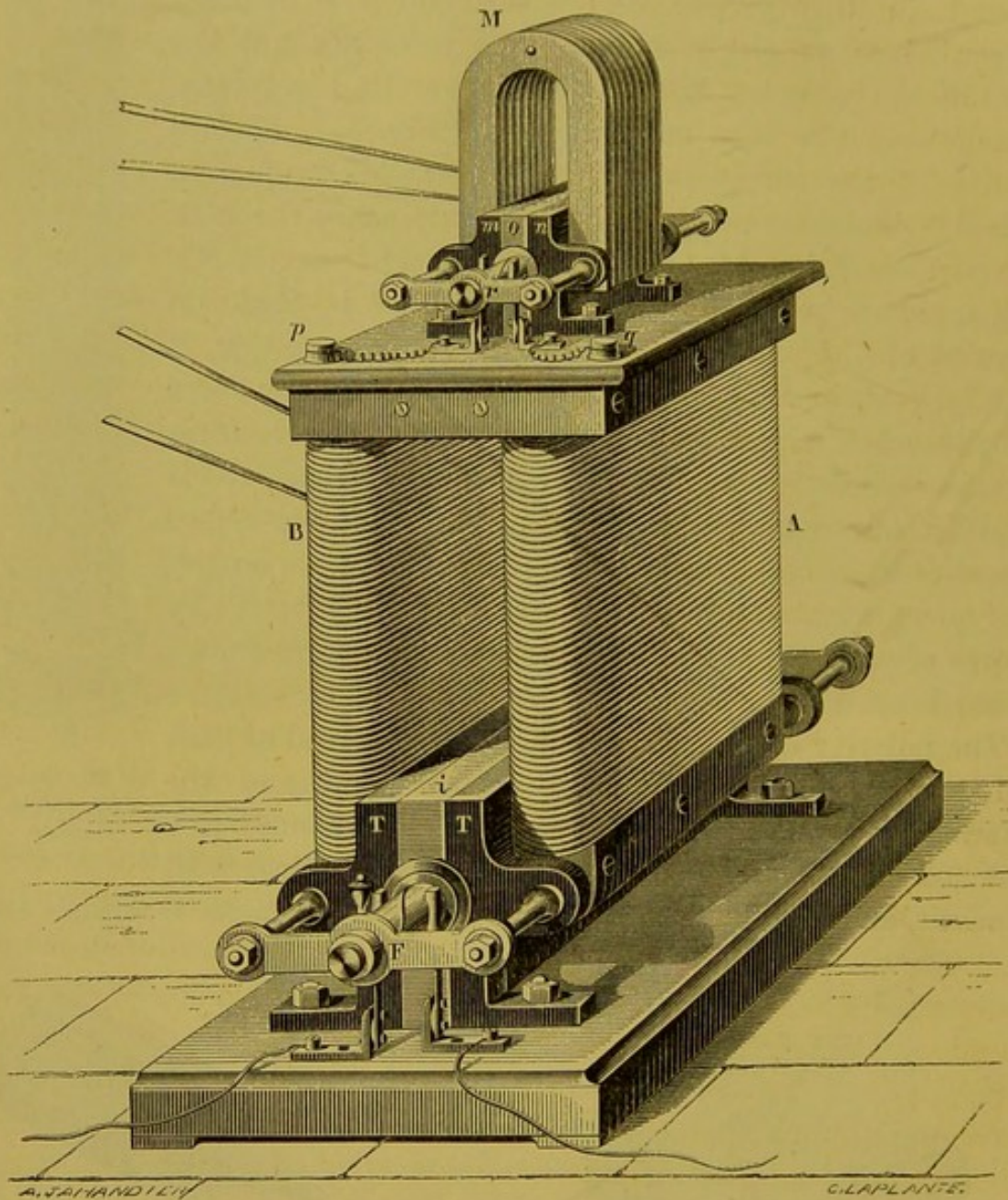
Fig. 548. — Wilde's Machine.
