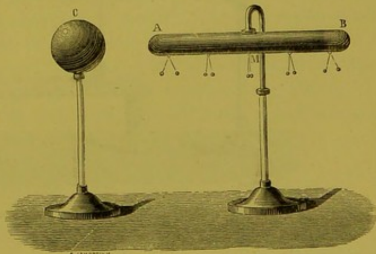
Fig. 335.—Electrification by Influence.
