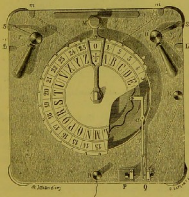
Fig. 564.—Breguet's Manipulator.
