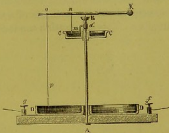
Fig. 511.—Position assumed by Vertical Current.
