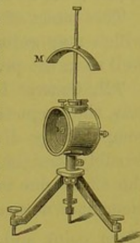
Fig. 471.—Thomson's Mirror Galvanometer.
