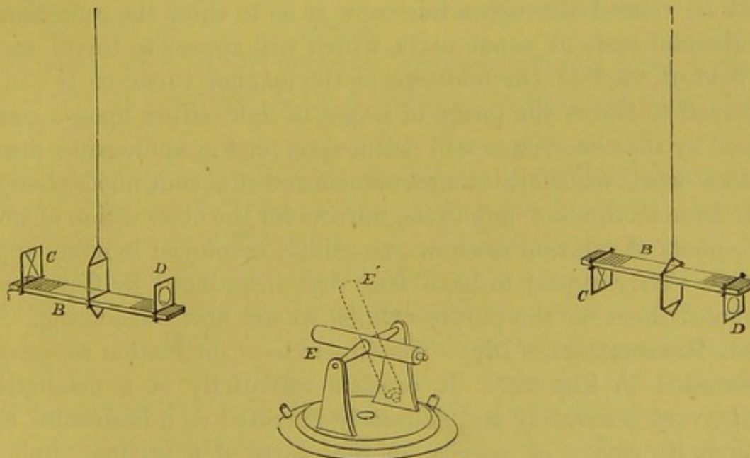
Fig. 426.—Declination Magnet.
