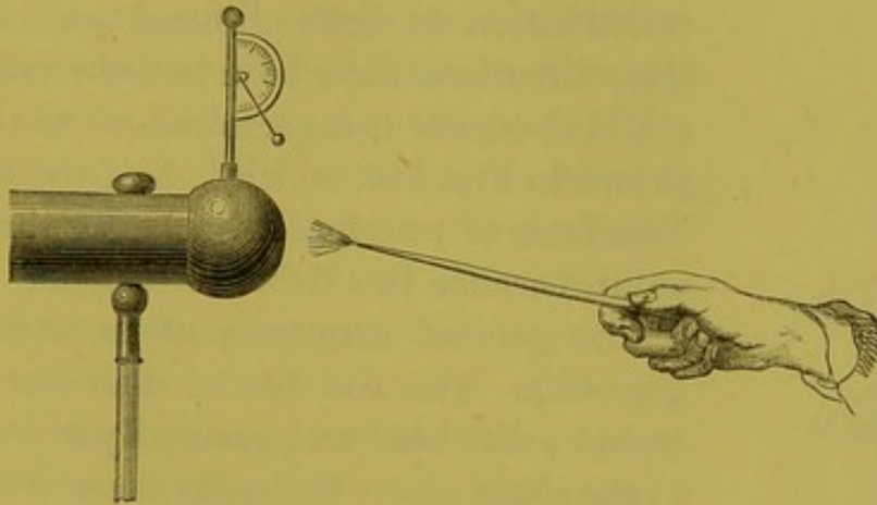
Fig. 408.—Conductor Discharged by presenting a Point.
