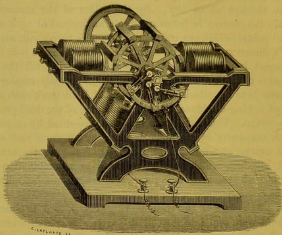
Fig. 580.—Froment's Engine.
