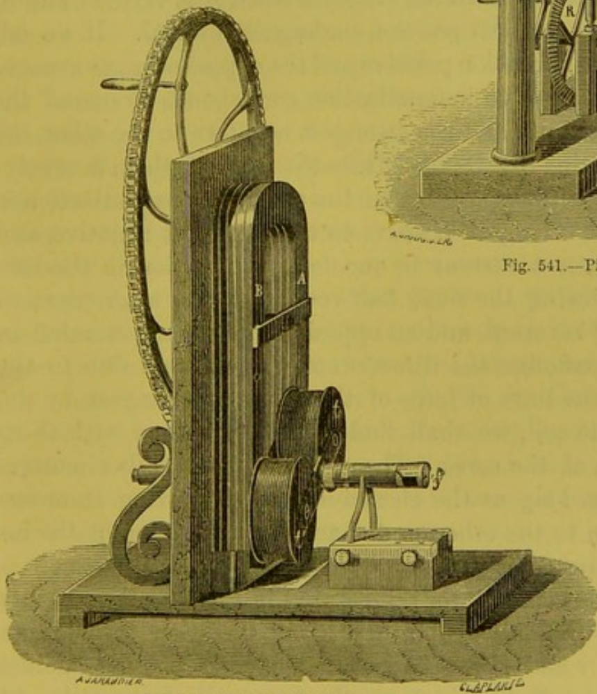
Fig. 542.—Clarke's Machine.
