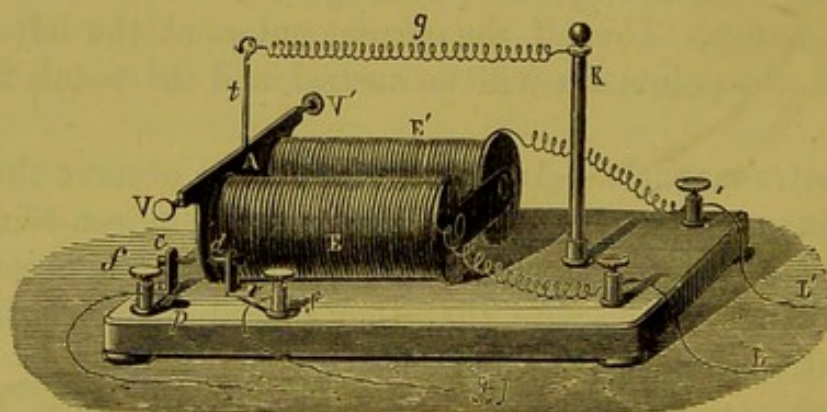
Fig. 529.—Electro-magnet with Opposing Spring.
