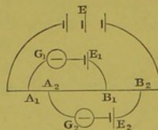
Fig. 486.—Latimer Clark's Method.
