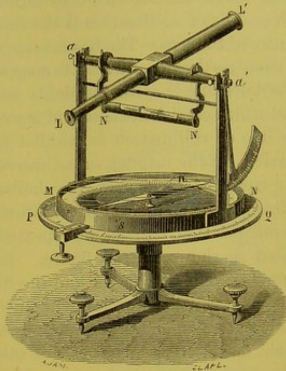
Fig. 425.—Declination Theodolite.
