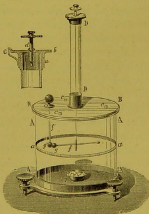
Fig. 339.—Coulomb's Torsion-balance.
