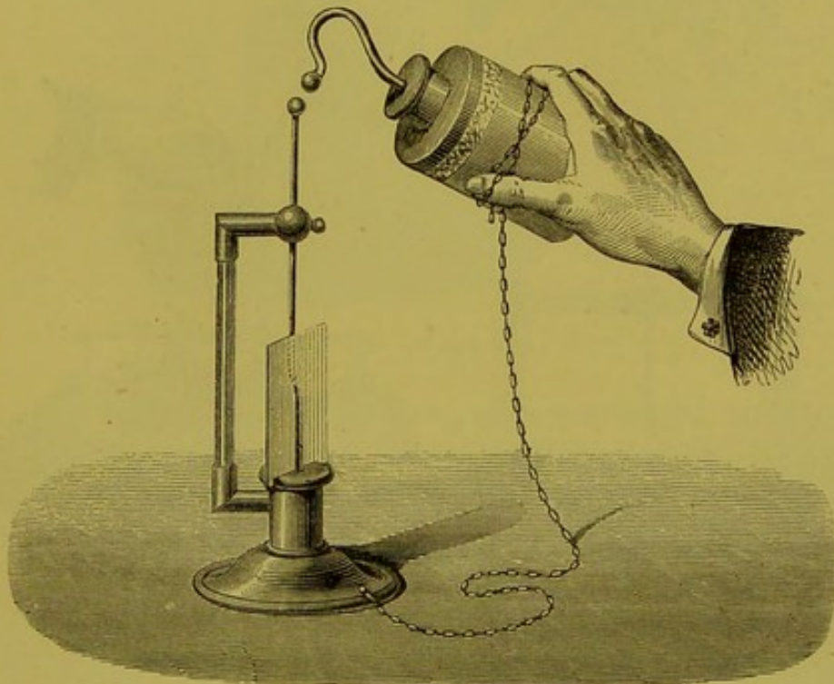
Fig. 397.—Puncture of Card.
