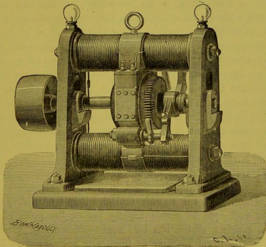
Fig. 555.—Gramme's Dynamo-electric Machine, for steam-power,
