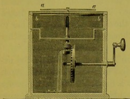
Fig. 556.—Arago's Rotations.
