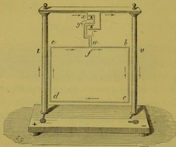
Fig. 502.—Attraction of Parallel Currents.
