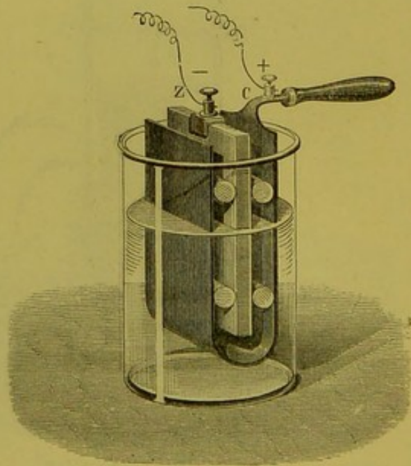
Fig. 453.—Wollaston's Cell.
