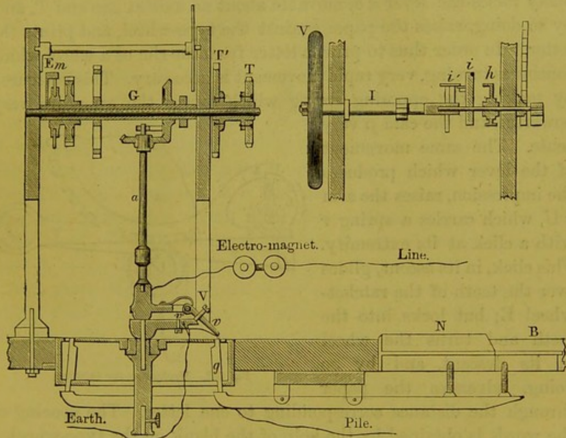
Fig. 571.—Type-shaft and Printing-shaft.
