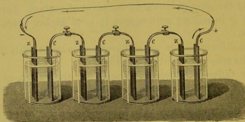
Fig. 447. —Battery of Four Elements.
