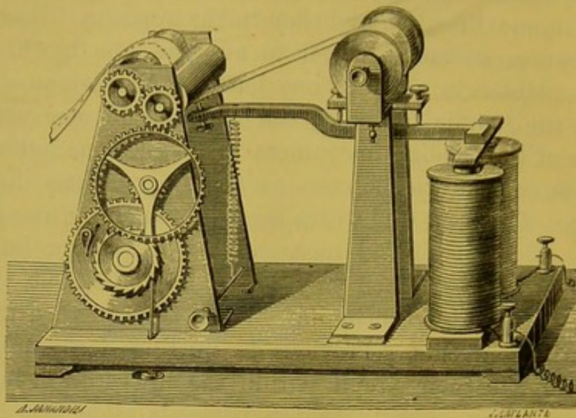
Fig. 566 —Morse's Telegraph.
