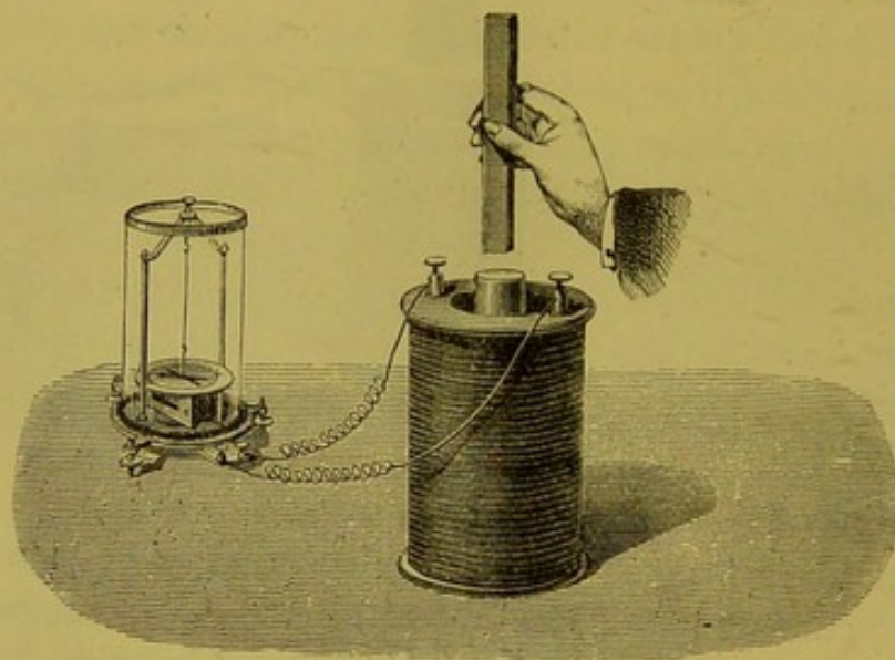
Fig. 534. —Current induced by Magnetization of Soft Iron.
