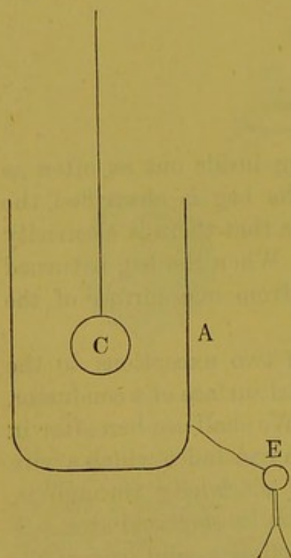
Fig. 344.—Ice-pail Experiment.
