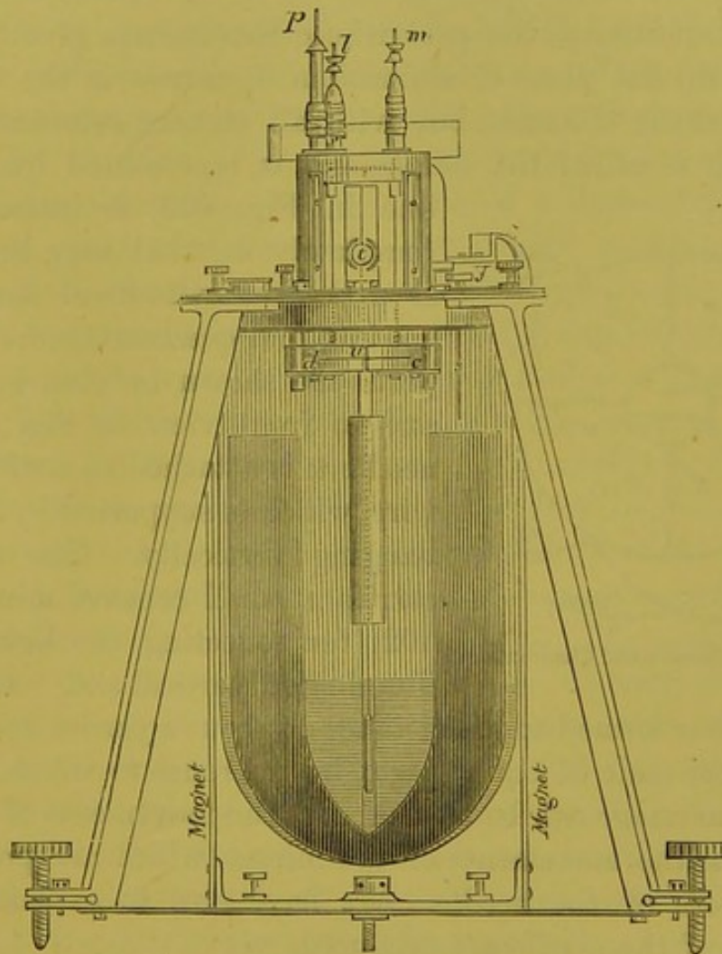
Fig. 402.—Quadrant Electrometer.
