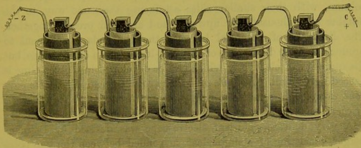
Fig. 458.—Bunsen's Battery.
