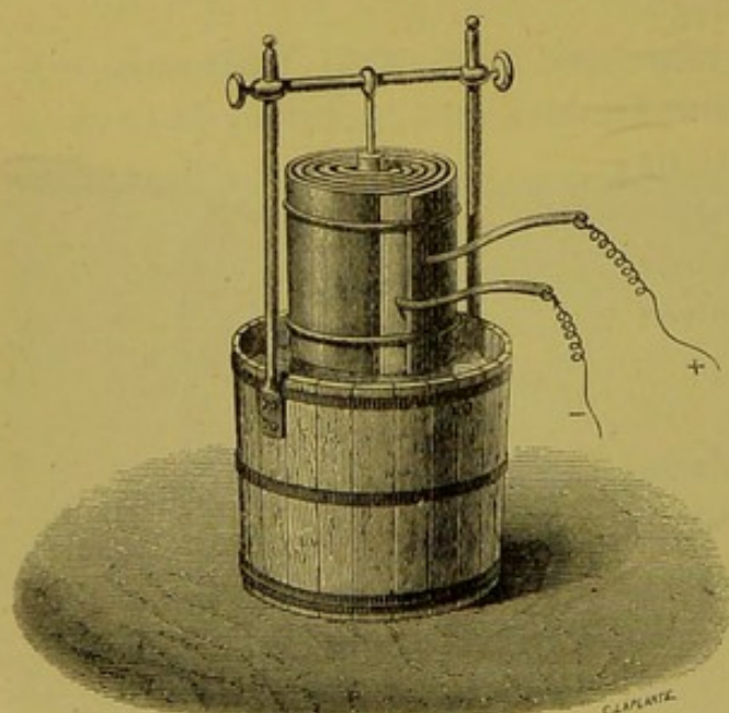
Fig. 455.—Hare's Deflagrator.
