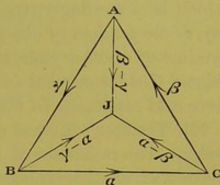
Fig. 491.—Theory of Conjugate Branches.
