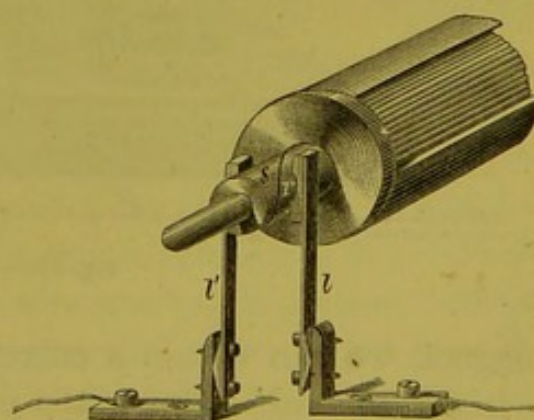
Fig. 547.—Commutator.
