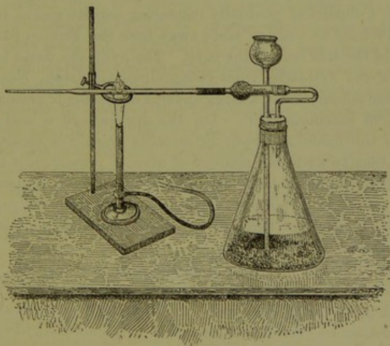
Fig. 24.—Marsh's apparatus.
