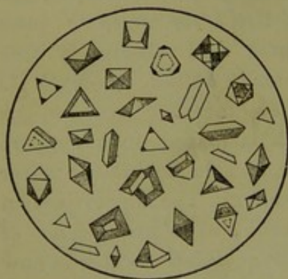
Fig. 23.—Crystals \text{As}_2\text{O}_3 .
