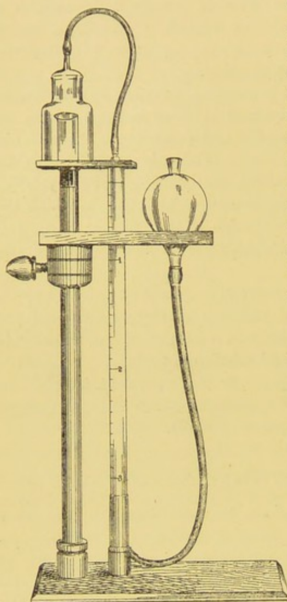
FIG. 5. Ureameter (the author's form).
