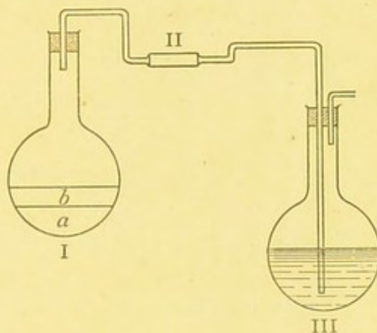
FIG. 16.—I, Flask containing, a , mixture of sal-ammoniac (one part by weight) and quicklime (two parts by weight); b , a layer of powdered quicklime; the flask with its contents is heated over a Bunsen flame; II, Wide glass tube containing the infected strip; III, Flask containing water to receive the ammonia.
