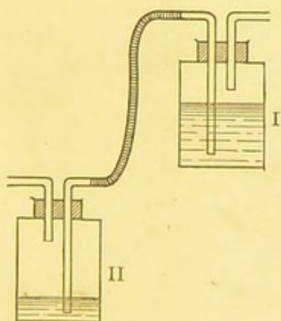
FIG. 8.—Aspirating Apparatus.
