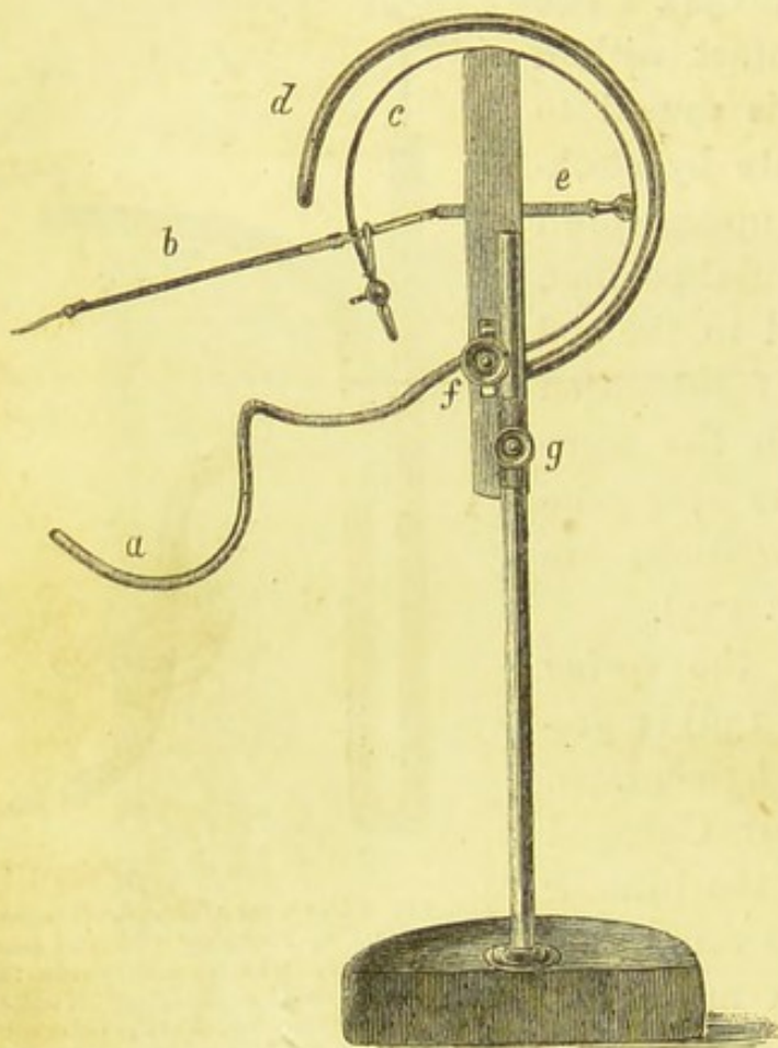
Fig. 136.—A form of Fick's Spring Kymograph. a , tube to be connected with artery; c , hollow spring, the movement of which moves b , the writing lever; e , screw to regulate height of b ; d , outside protective spring; g , screw to fix on the upright of the support.
