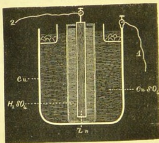
Fig. 277.—Diagram of a Daniell's battery. (After Balfour Stewart).
