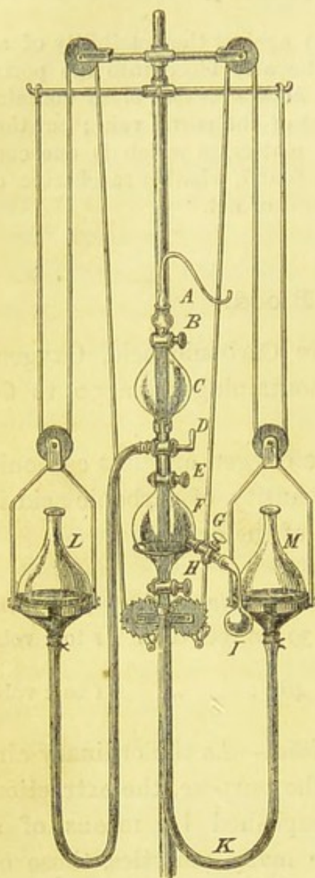
Fig. 80.—Ludwig's Mercurial Pump.
