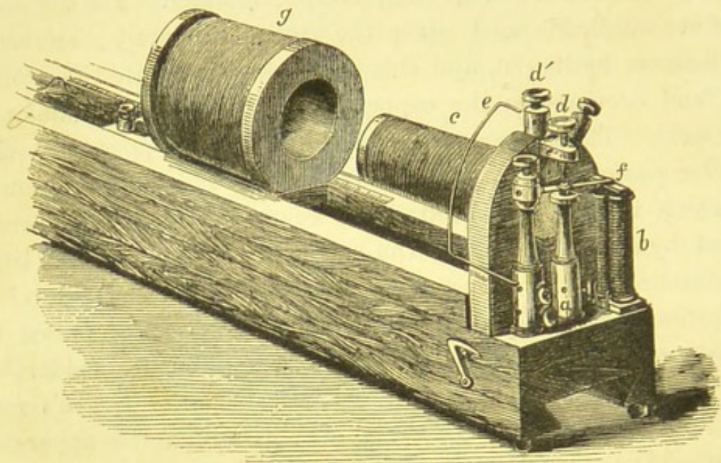
Fig. 278.—Du Bois Reymond's induction coil.
