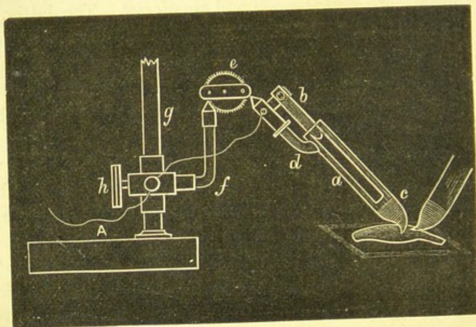
Fig. 275.—Diagram of Du Bois Reymond's non-polarisable electrodes. a , glass tube filled with a saturated solution of zinc sulphate, in the end, c , of which is china clay drawn out to a point; in the solution a well amalgamated zinc rod is immersed and connected by means of the wire which passes through A with the galvanometer. The remainder of the apparatus is simply for convenient application. The muscle to the end of the second electrode is to the right of the figure.
