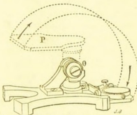
Fig. 21.—Method of packing Nachet's microscope.
