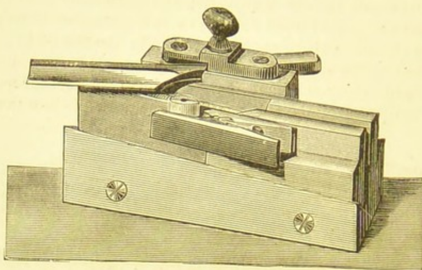
Fig. 5.—Section Cutter (Rivet's).
