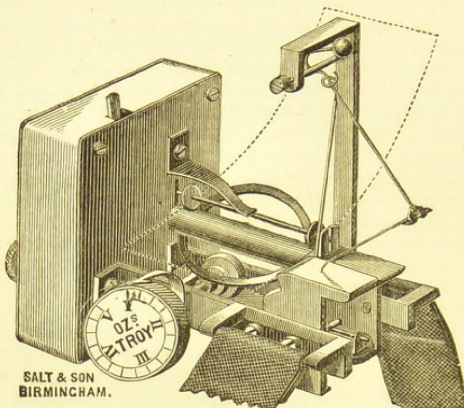
Fig. 43.—Dudgeon's Sphygmograph.
