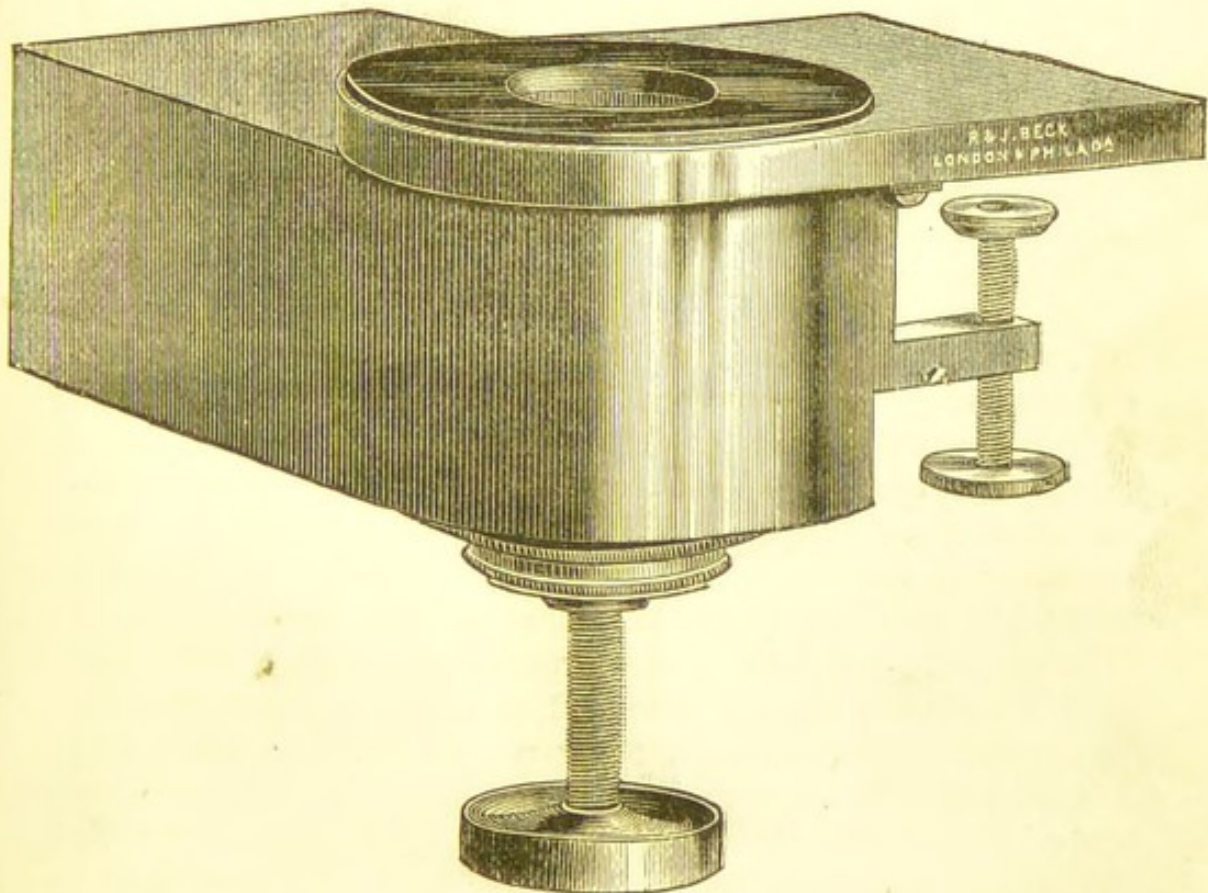
Fig. 4.—Rutherford's Microtome, with ice-box.
