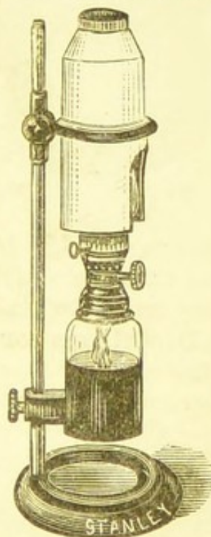
Fig. 23.—Lamp for work with microscope.
