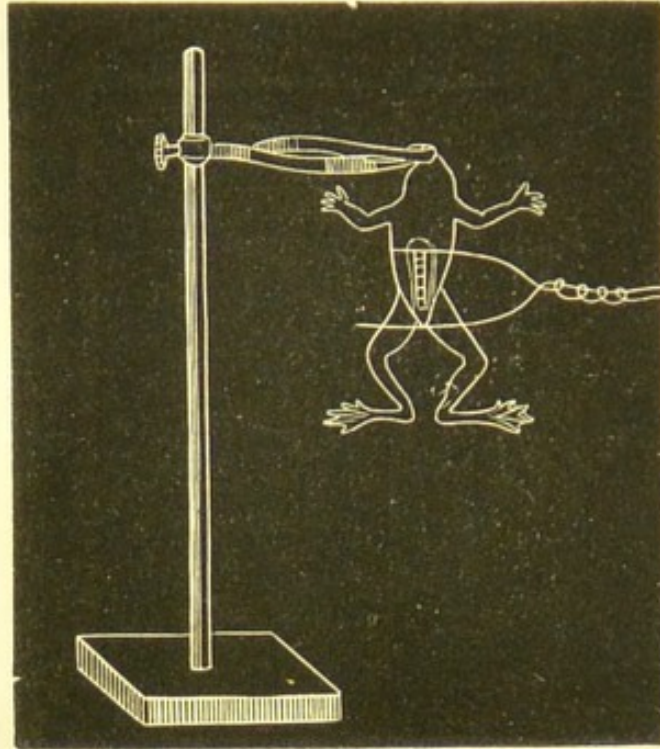
Fig. 34.—Galvani's Experiment.
