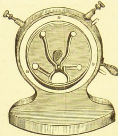
Fig. 36.—Commutator.
