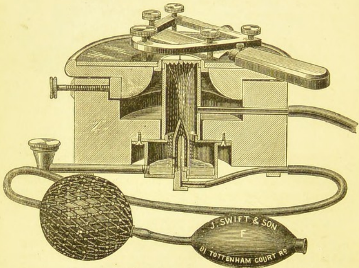
Fig. 7.—Groves' modification of Williams' Microtome.
