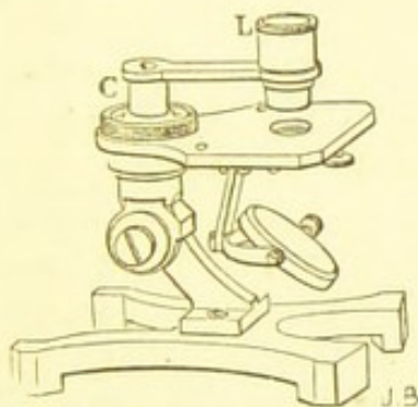
Fig. 20.—Nachet's microscope as a dissecting microscope.
