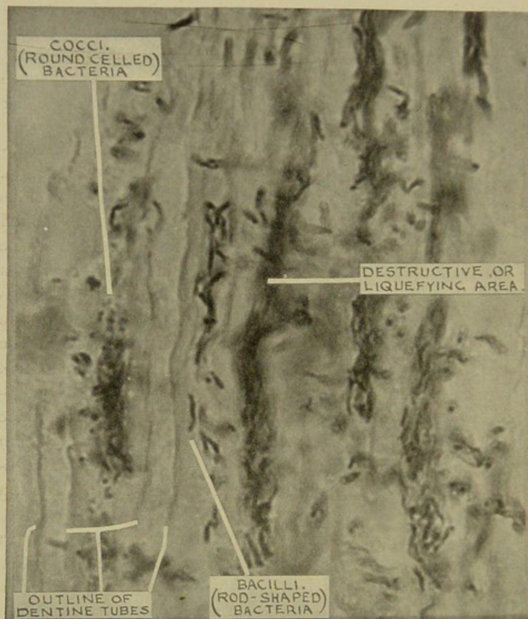
Fig. 21.—Longitudinal Section of Carious Dentine. \times 2250
