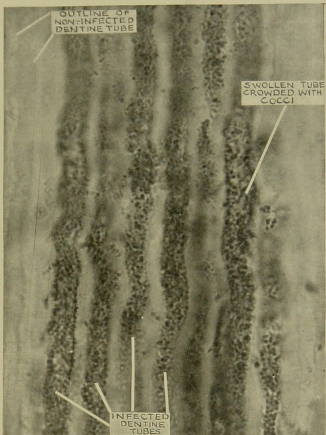
Fig. 20.—Longitudinal Section of Carious Dentine. \times 2250 (B 972) 65 9
