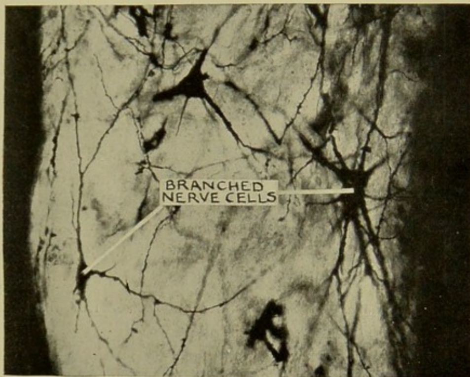
Fig. 5.—Longitudinal Section of Spinal Cord. \times 125
