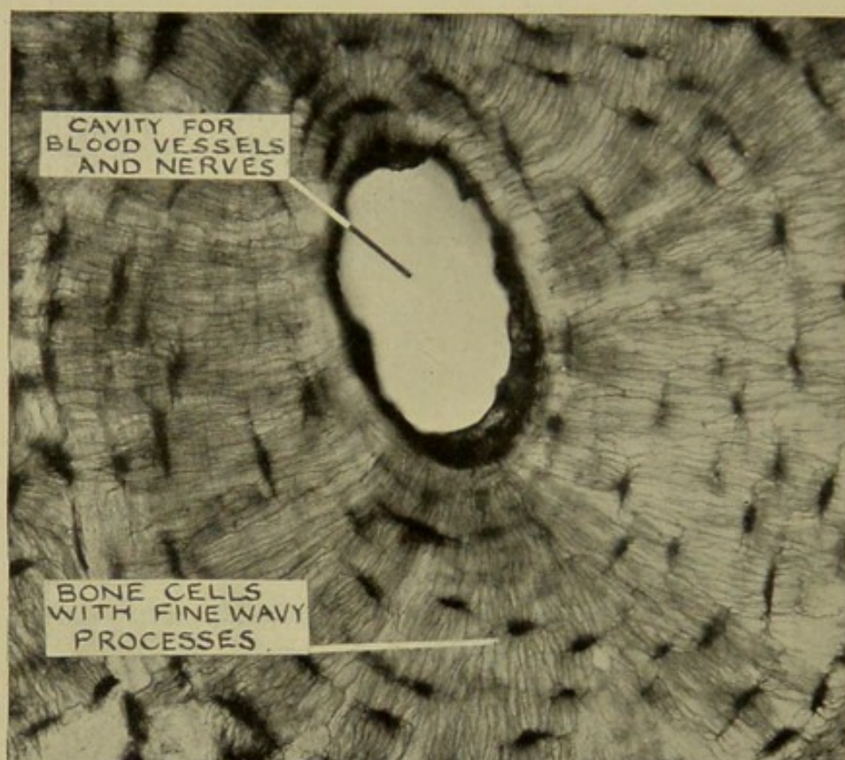
Fig. 2.—Transverse Section of Bone. \times 230
