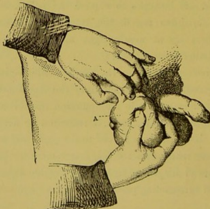
FIG. II. — Reduction of Scrotal Hernia by Taxis.
