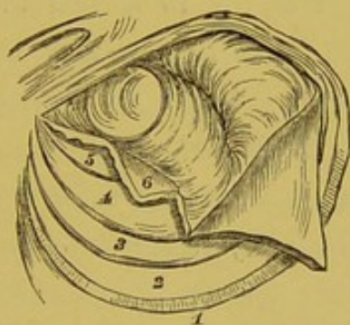
FIG. 9.—Coverings of Femoral Hernia. 1, skin; 2, superficial fascia, cribriform fascia; 3, crurale sheath; 4, femoral sheath; 5, septum crurale; 6, peritoneum.
