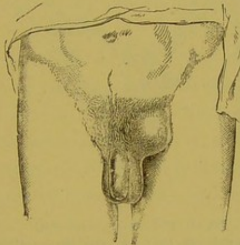
FIG. 50.—Direct Inguinal Hernia.
