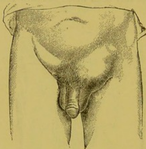
FIG. 51.—Oblique Inguinal Hernia. Bubonocoele on right side, but passing through external ring on left.
