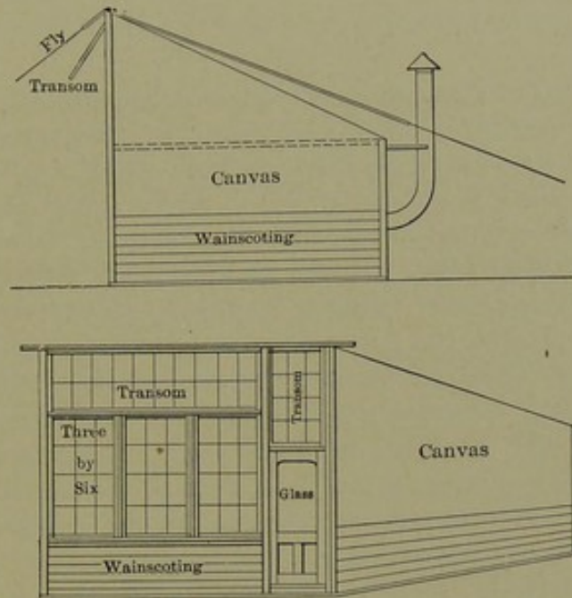
FIG. 125.—The Lapham tent.
