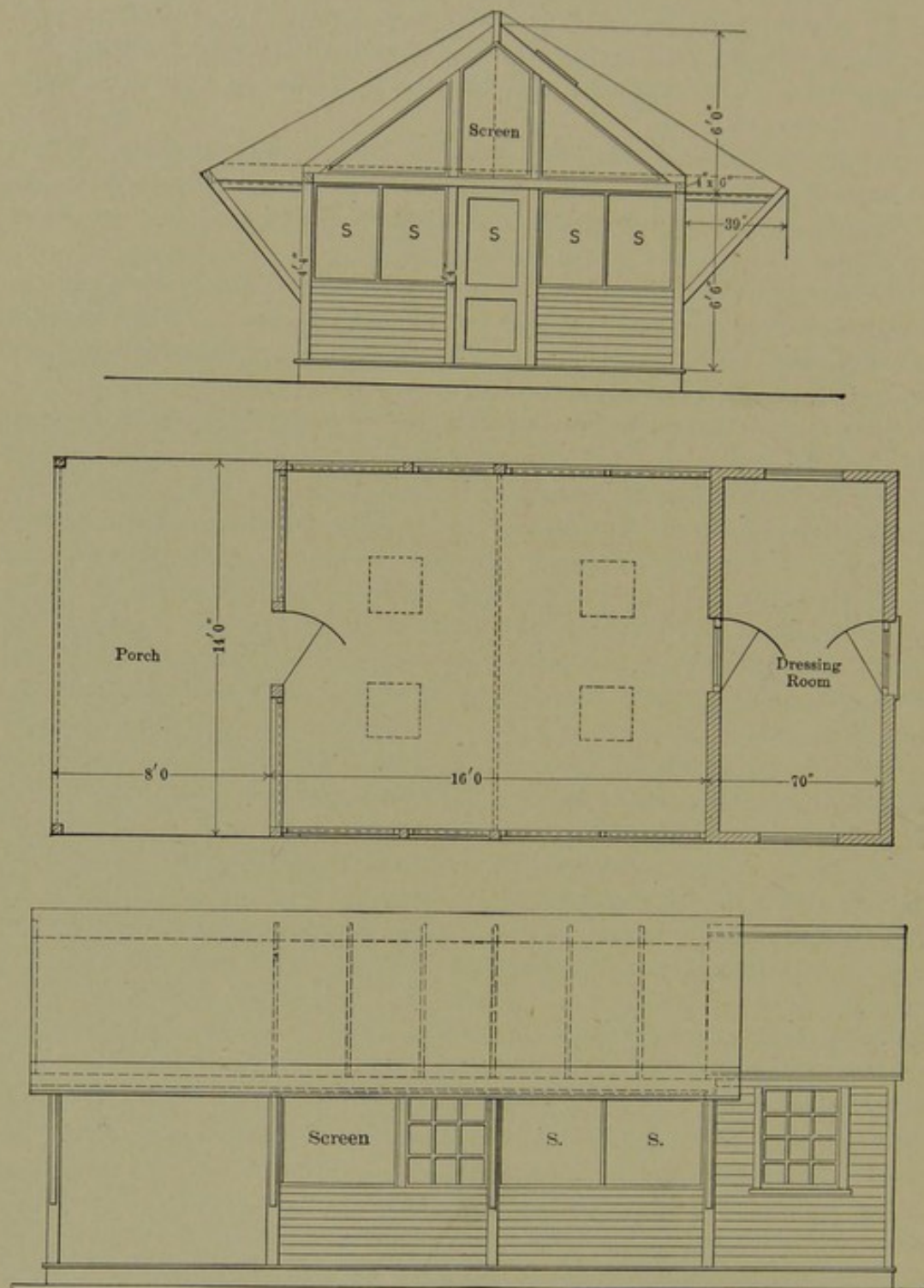
FIG. 126.—Dr. Biggs's tent-house.
