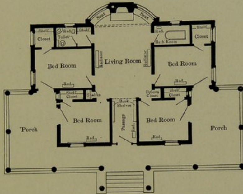
FIG. 127.—Plan of Nathan Cottage at Saranac Lake. (See page 222.)
