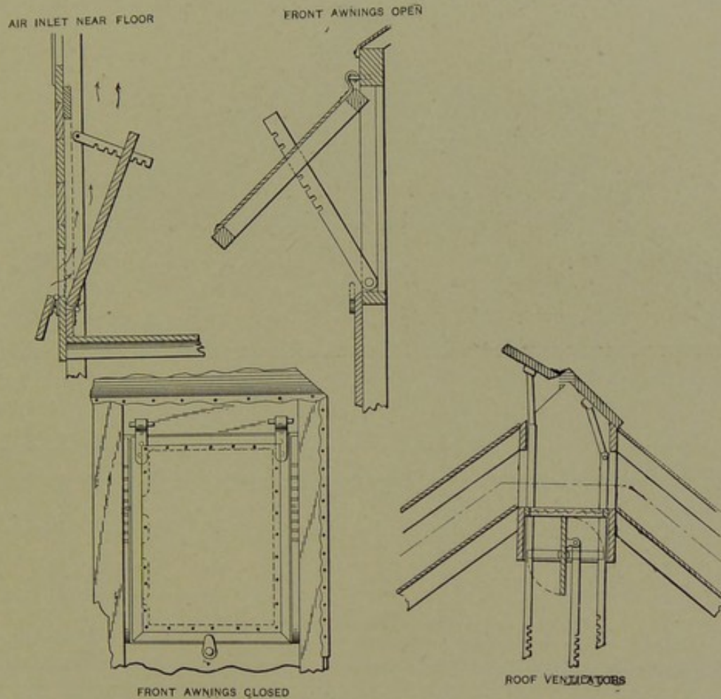
FIG. 120.—Details of the Tucker tent.
