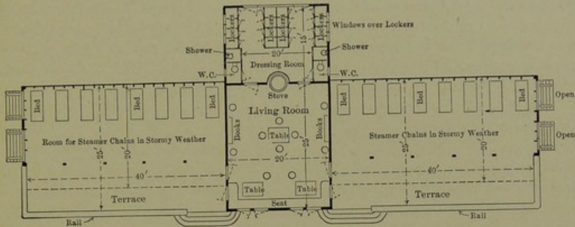
FIG. 123.—Ground plan of improved lean-to.
