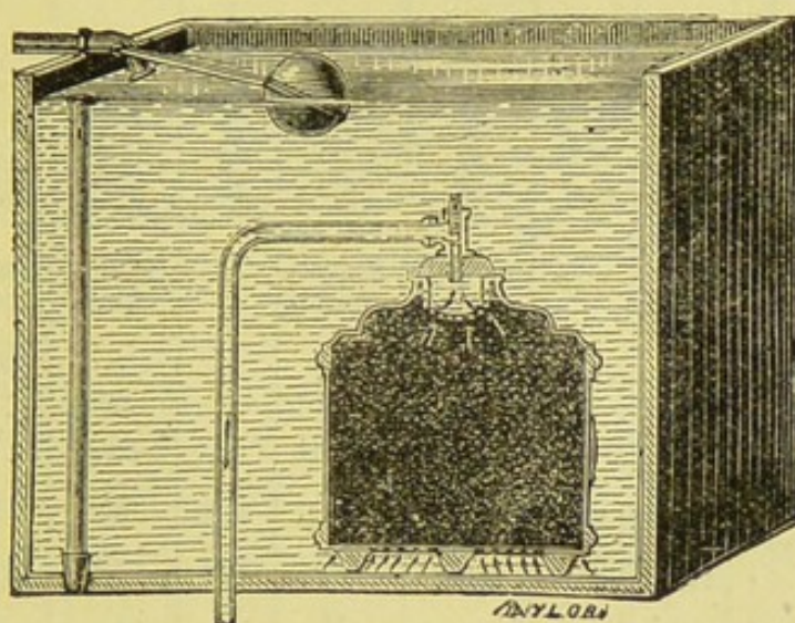
No. 121.—CISTERN CHARCOAL FILTER.
