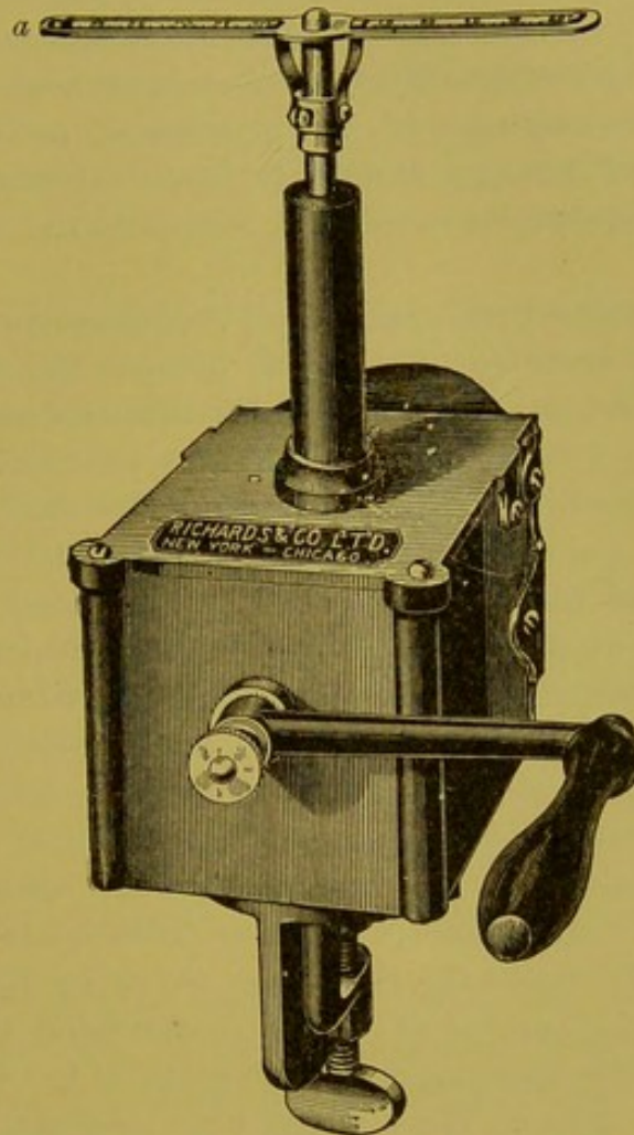
FIG. 17.—Daland's Haematocrit. Two capillary tubes in place on the horizontal whirling beam. The instrument is to be fastened to the edge of some solid and bulky piece of furniture by means of the thumb-screw seen at the bottom of the cut. If not very tightly secured, it will work loose when the handle is revolved rapidly.
