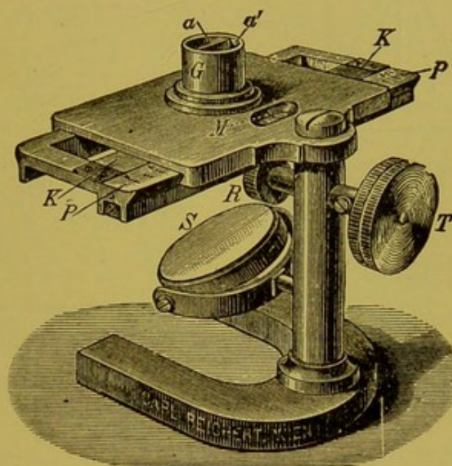
FIG. 19.—v. Fleischl's Hæmometer. a , Partition into which blood is put; a' , partition into which water is put; G , mixing cell; K , K , colored glass slip (see Fig. 11, A ); P , P , metal frame on which scale is marked; R , S , reflector; T , screw which moves the frame, P , P .
