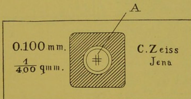
FIG. 5.—Thoma-Zeiss Counting Slide. A, Ruled disc.
