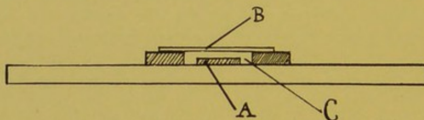
FIG. 4.—Thoma-Zeiss Counting Slide. A, Ruled disc; B, cover-glass; C, moat.
