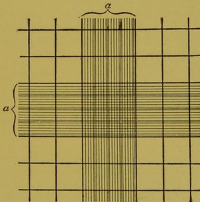
FIG. 10.—Modified Ruling of Thoma-Zeiss Counting-chamber.
