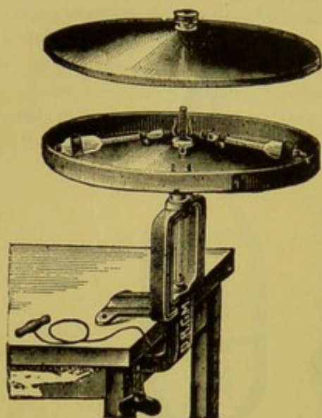
Fig. 192.—Gerber's acid butyrometer.
