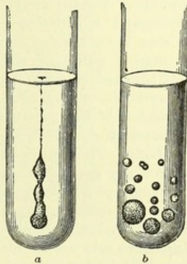
FIG. 166.— Bacillus œdematis maligni , cultures in nutrient gelatin; a , long stick culture; b , colonies at bottom of gelatin tube. (Flügge.)
