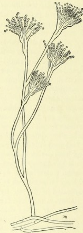
FIG. 188. — Penicillium glaucum ; m , mycelium, from which is given off a branching pedicel bearing spores. \times 150 .
