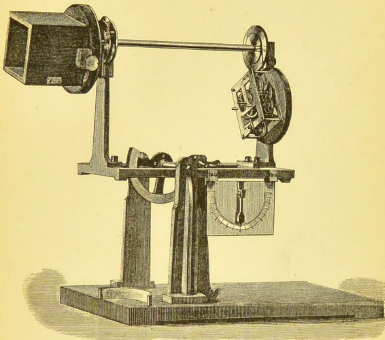
Klinostat with Adjustable Stand.
