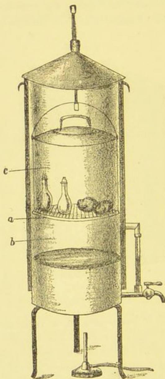
Koch's Steam-chest.
