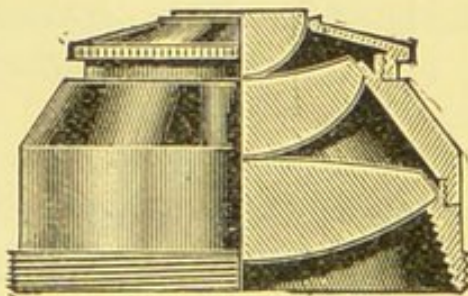
Abbe's Condenser.
