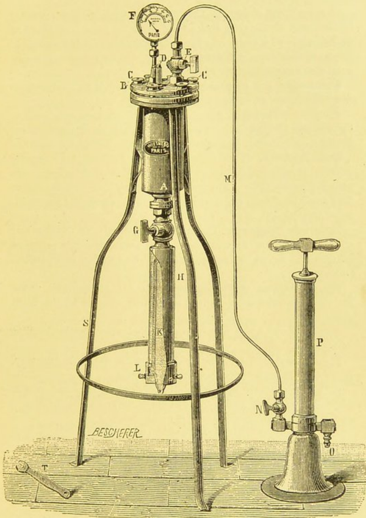
Pasteur-Chamberland filter with pressure. A. Container. H. Filter. K. Porcelain. P. Air-pump.
