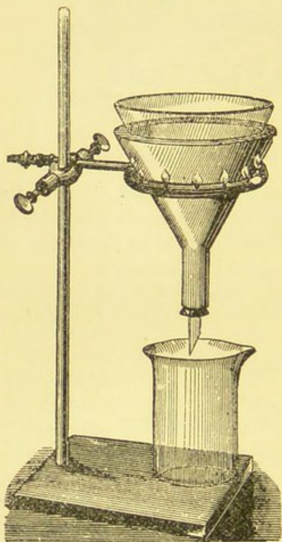
Hot-water filter.
