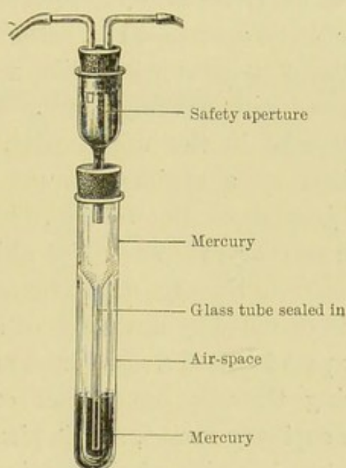
FIG. 12.—SCHENK'S THERMO-REGULATOR.
