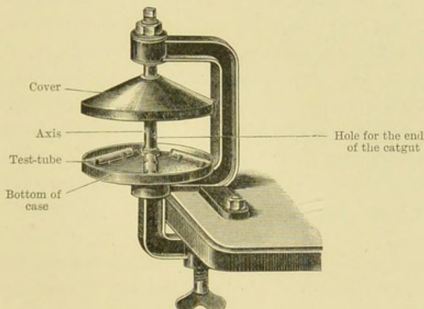
FIG. 21.—GÄRTNER'S CENTRIFUGE.
