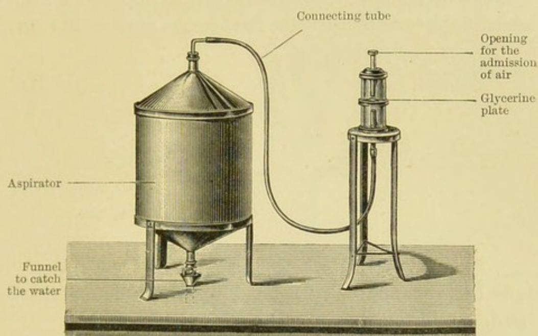
FIG. 28.—POUCHET'S AËROSCOPE.
