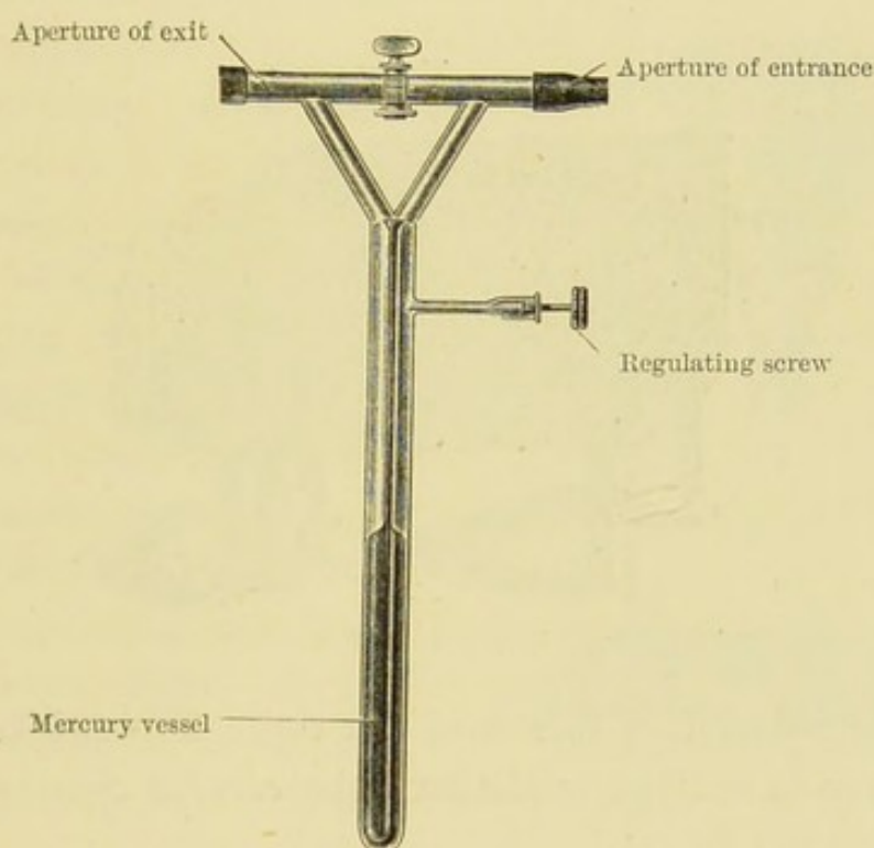
FIG. 13.—ALTMANN'S THERMO-REGULATOR.
