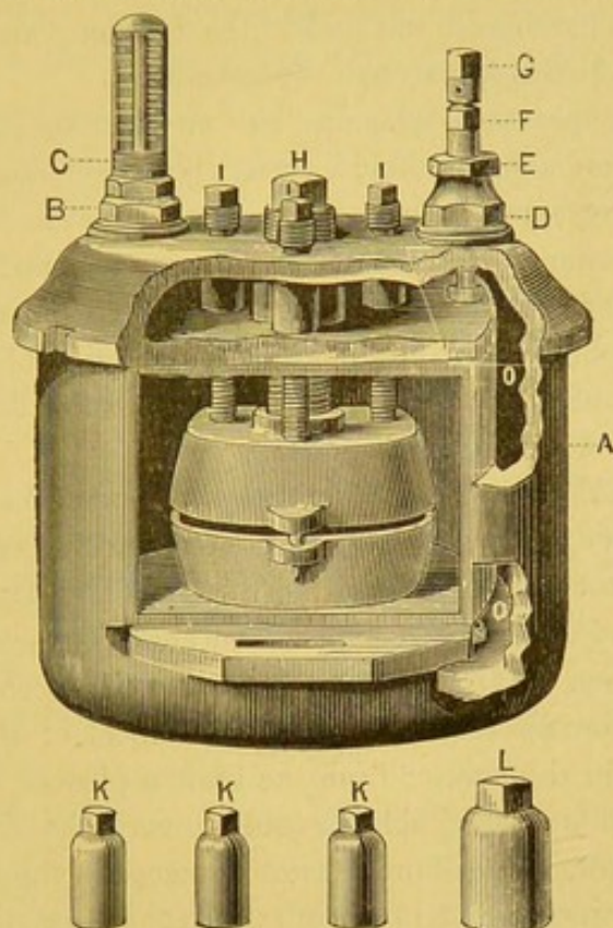
FIG. 338.—SECTIONAL VIEW OF NEW MODE HEATER.
