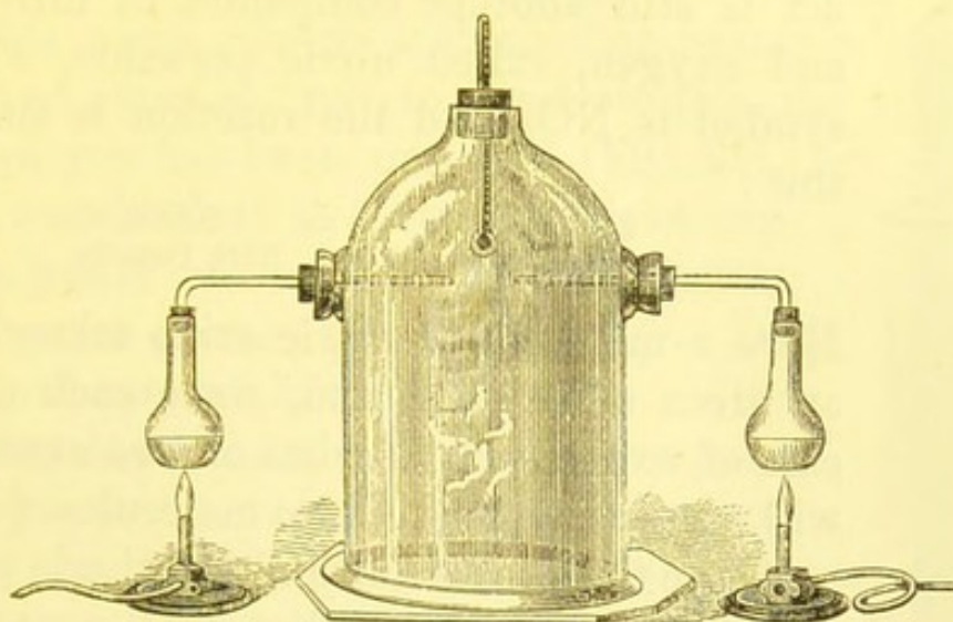
FIG. 26.—Combination of Ammonia and Hydrochloric-Acid Gases.
