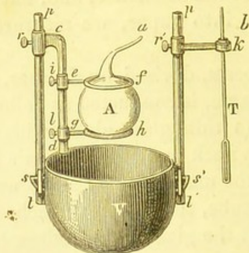
FIG. 18.—Dumas' Method of finding the Specific Gravity of Vapors.
