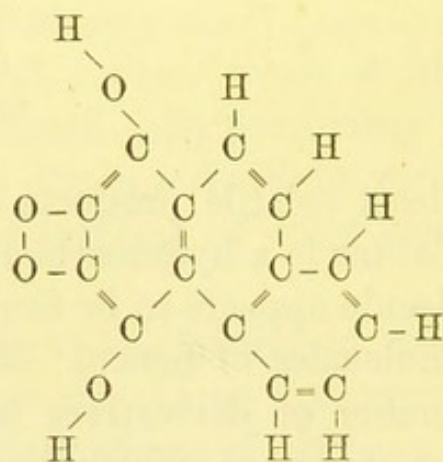
Anthraquinonic Acid (Alizarine).
