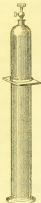
FIG. 27.—Combination of Nitric-oxide and Oxygen Gas.
