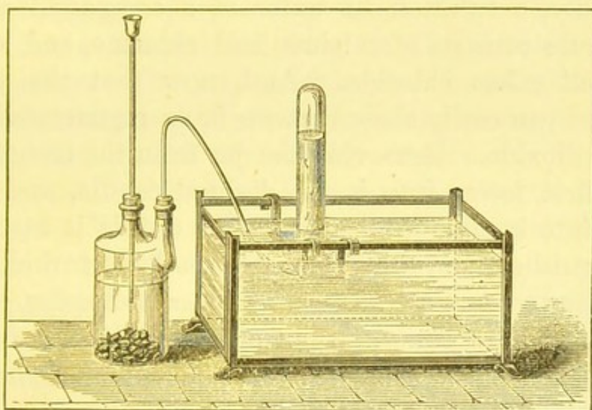
FIG. 22.—Pneumatic Trough, with Two-necked Gas-bottle.
