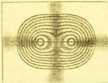
FIG. 15.—Rings, Biaxial Crystals.
