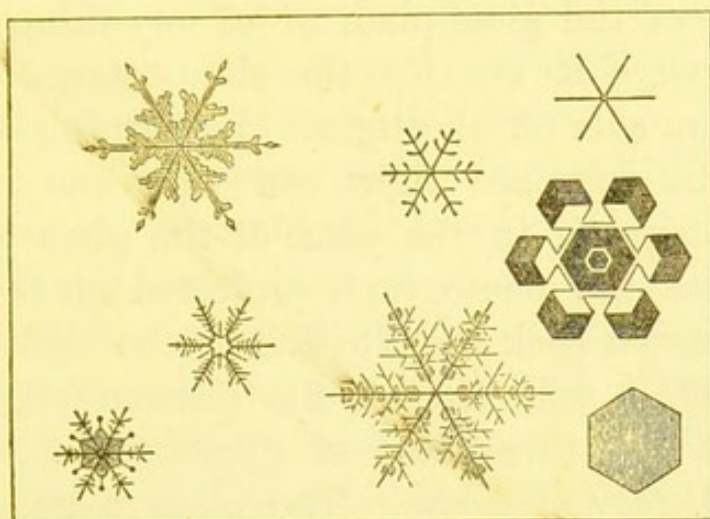
FIG. 11.—Snow-Crystals.
