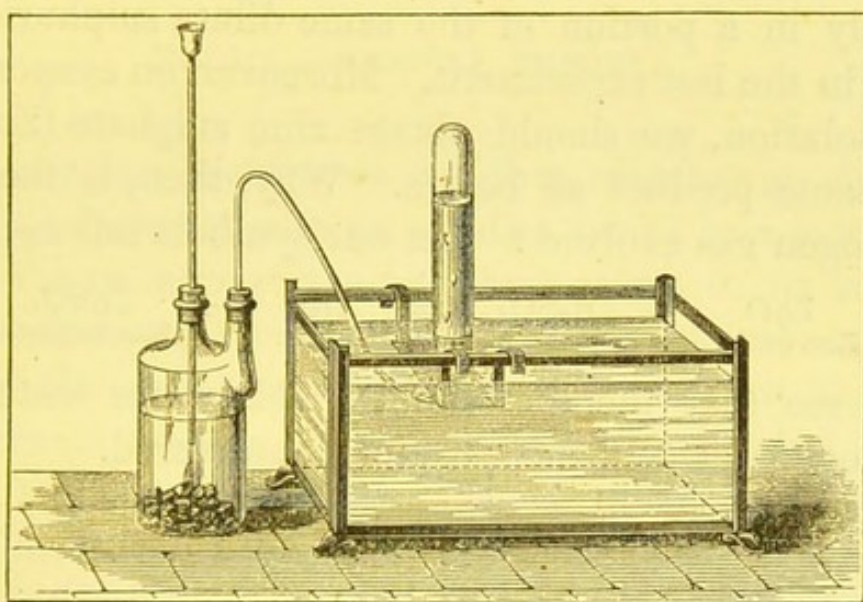
FIG. 31.—Preparation of Hydrogen Gas.
