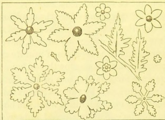
FIG. 10.—Ice-Flowers.
