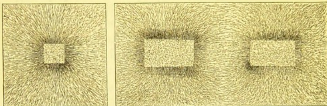
FIG. 13.—Magnetic Curves, two poles.
