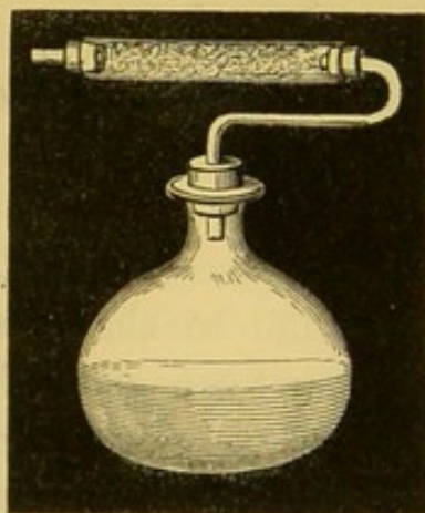
Apparatus for estimating the loss by weight of carbonic acid from fermentation.
