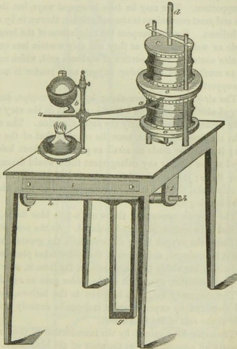
FIG. 182. aa Air-pipe leading from the bellows to the lamp; b Vapor-pipe; c c c A round bellows, 10 inches in diameter; d A rod attached to the upper movable head of the bellows, and passing through cross-piece e , which serves to keep the head in a horizontal position; f A rod attached in a similar manner to the lower movable head of the bellows and passing down through the table; g A stirrup attached at the upper end to shaft h h ; i i Support for shaft h h , by means of an arm projecting backwards from shaft h h , and attached to the lower end of rod f , the force is communicated from the foot of the artist to the bellows.
