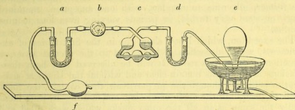
Arrangement of the Apparatus employed.
