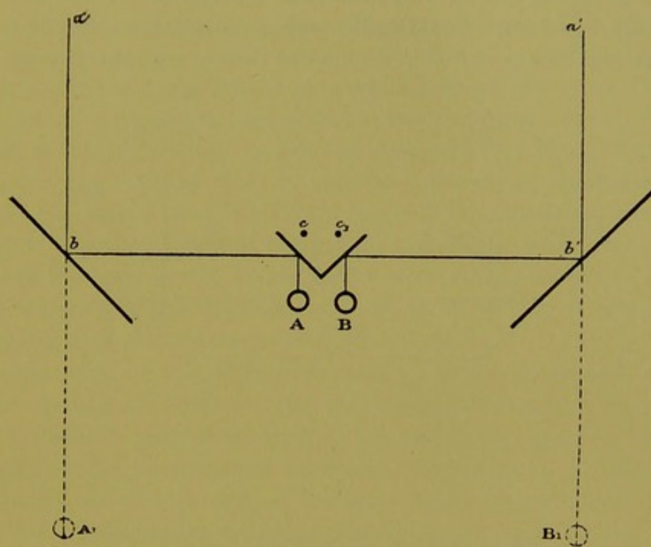
Fig. 191. — Telestereoscope of Helmholtz.
