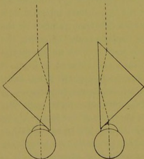
Fig. 190. — Pseudoscope of Wheatstone.
