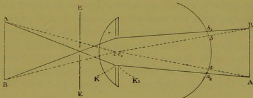
Fig. 56. — Magnification by means of the stenopaic opening.
