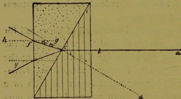
Fig. 37. — Prism of Wollaston.
