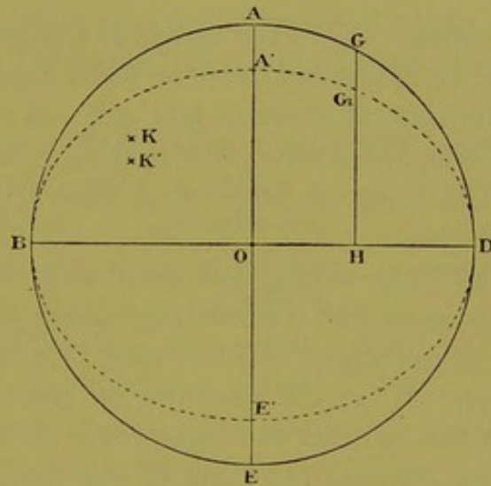
Fig. 79. — Construction of the elliptical diffusion spot.
