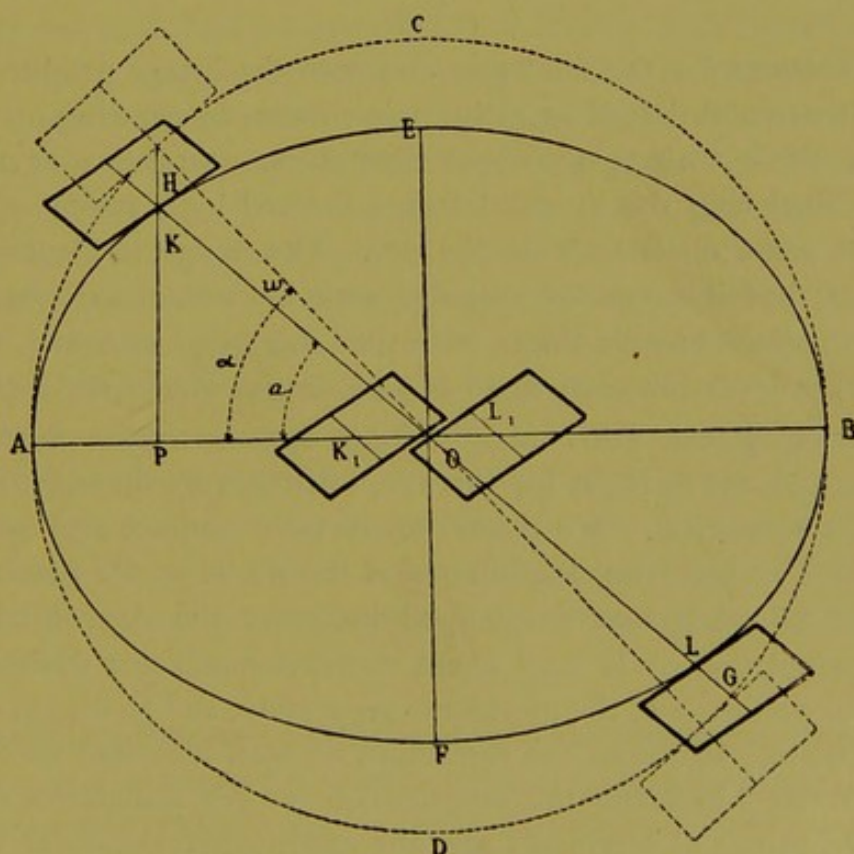
Fig. 83. — Explanation of the difference in the level ( dénivellation ).
