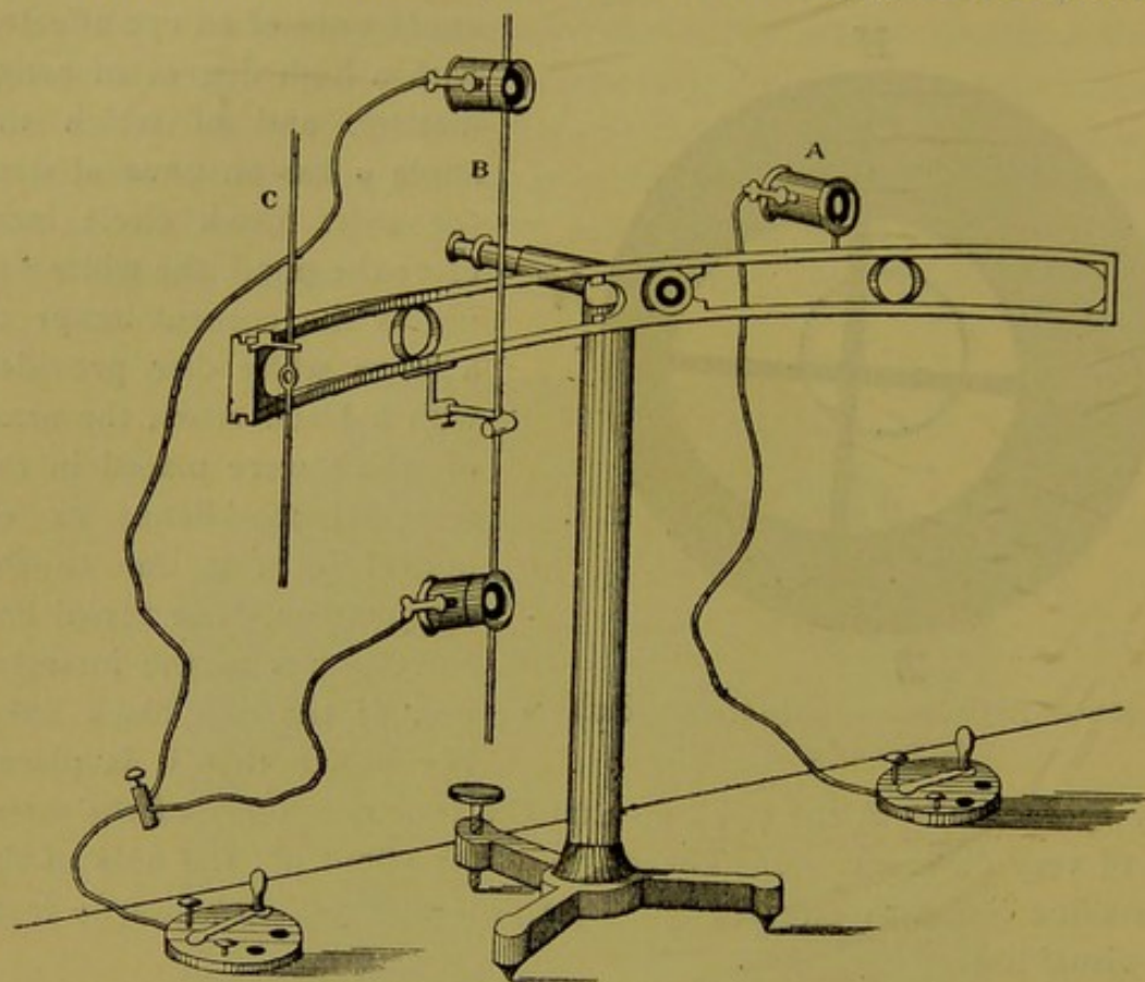
Fig. 47. — The ophthalmophakometer.
