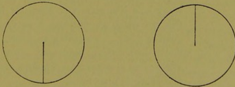
Fig. 180. — Discs of Volkman .
