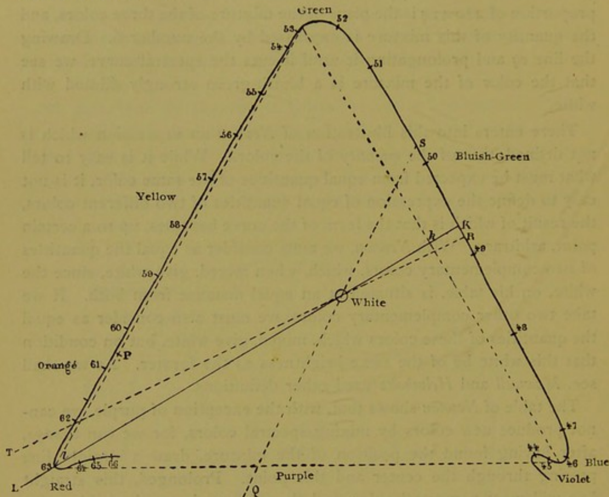
Fig. 160. — Color table of Maxwell .
