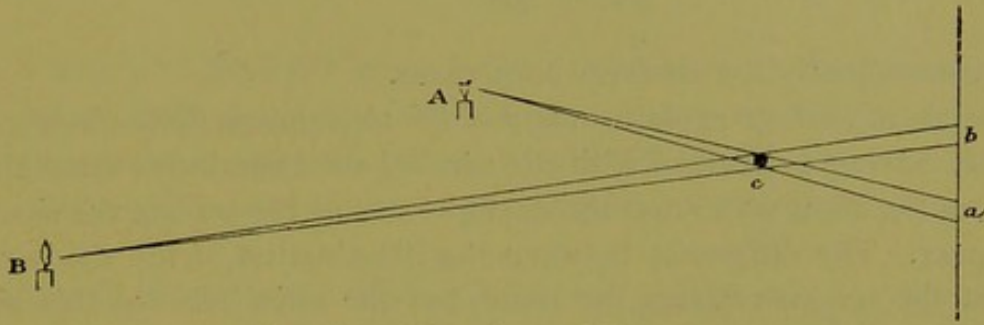
Fig. 147. — Experiment of Bouguer .
