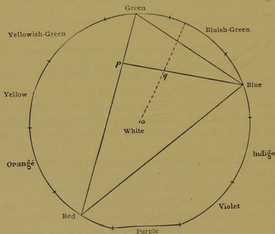
Fig. 159. — Table of colors after Newton .
