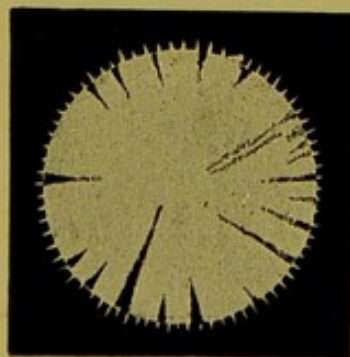
Fig. 101. — Incipient cataract, seen entoptically. (After Darier.)
