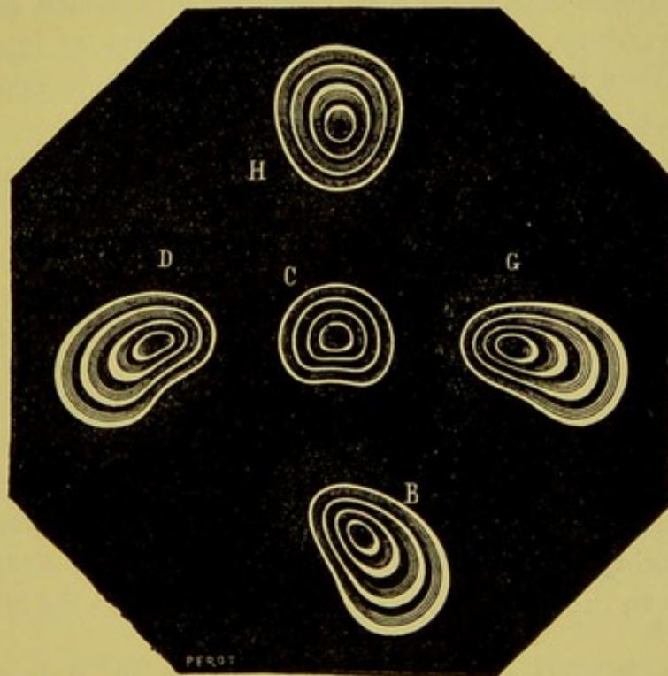
Fig. 84. — Keratoscopic images of a case of keratoconus.
