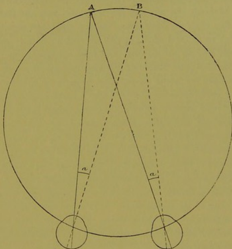
Fig. 185.—Horopter of Johannes Müller.
