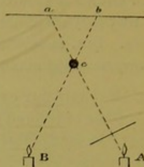
Fig. 154. Experiment with colored shadows.
