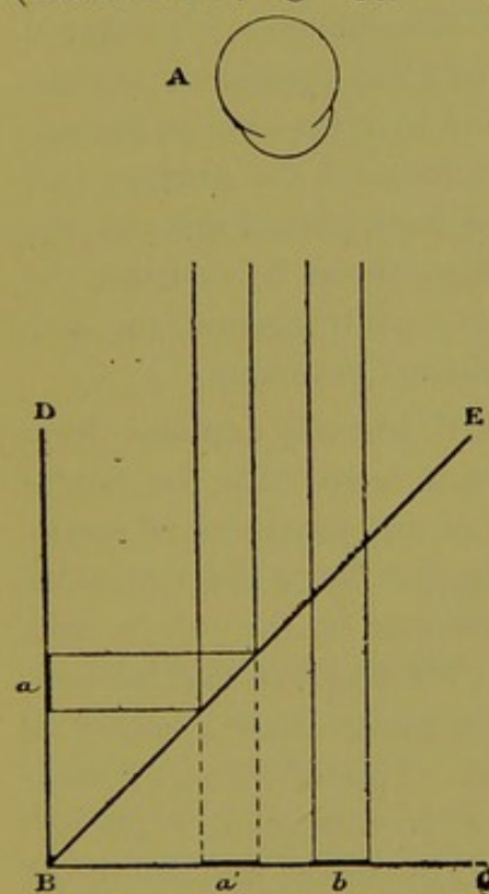
Fig. 153. Experiment of Ragona Scina .
