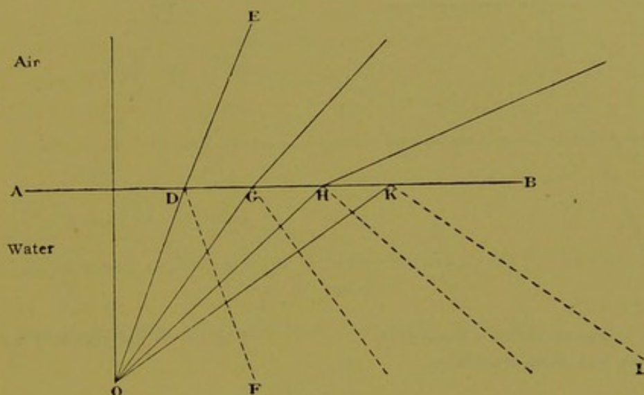
Fig. 8.—Total Reflection.
