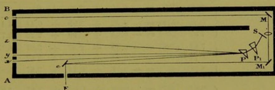
Fig. 161. — "Color box" of Maxwell.
