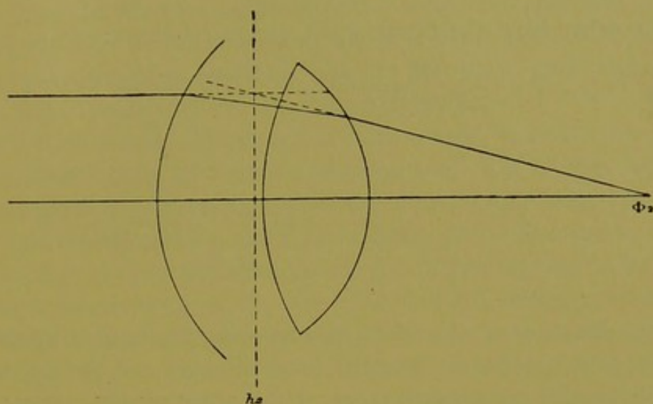
Fig. 19. — Construction to find the second principal plane.
