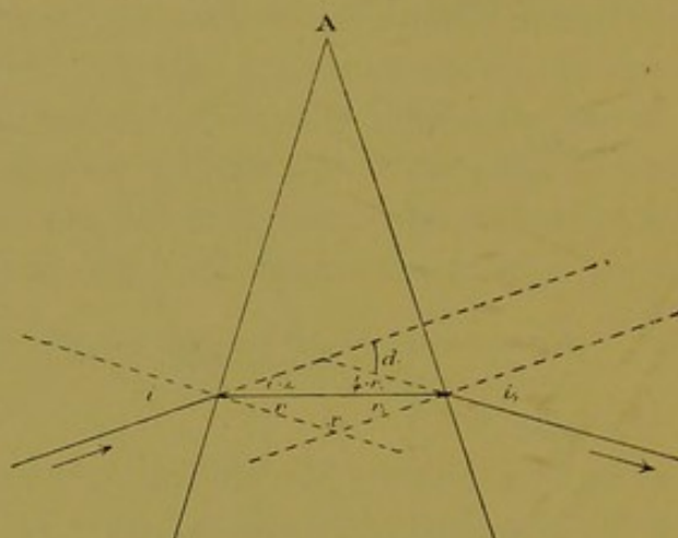
Fig. 11. — Refraction by a prism.
