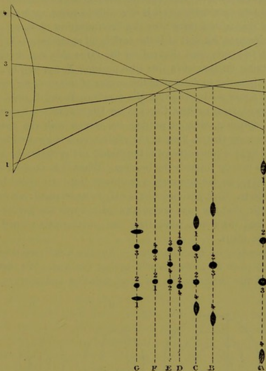
Fig. 62.—Spherical aberration of a lens.
