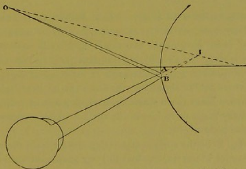
Fig. 6. — Construction of the utilized part AB of a mirror.
