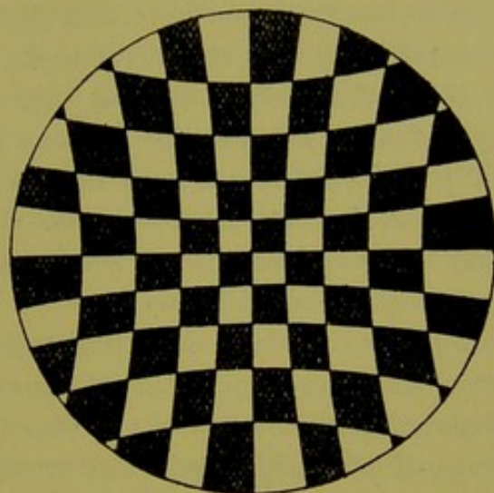
Fig. 144. — Hyperbolic chess-board of Helmholtz .
