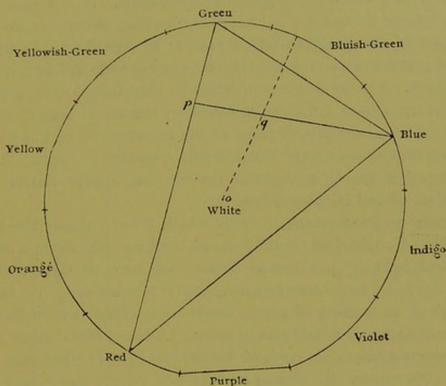
Fig. 152. — Table of colors after Newton.
