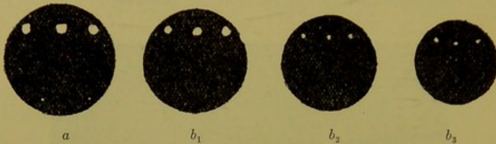
Fig. 114. — Reflection images, on the anterior surface of the crystalline of my right eye, of three lamps placed on a horizontal line, a , in a state of repose; b 1 b 2 b 3 , in different stages of accommodation. Highest accommodation 3 D. with cocaine.
