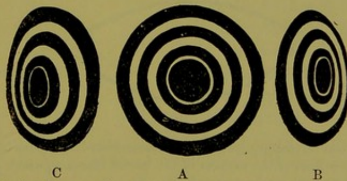
Fig. 122a. — Reflection images on the anterior surface of the dead crystalline lens. A, at the center; B and C, towards the borders.
