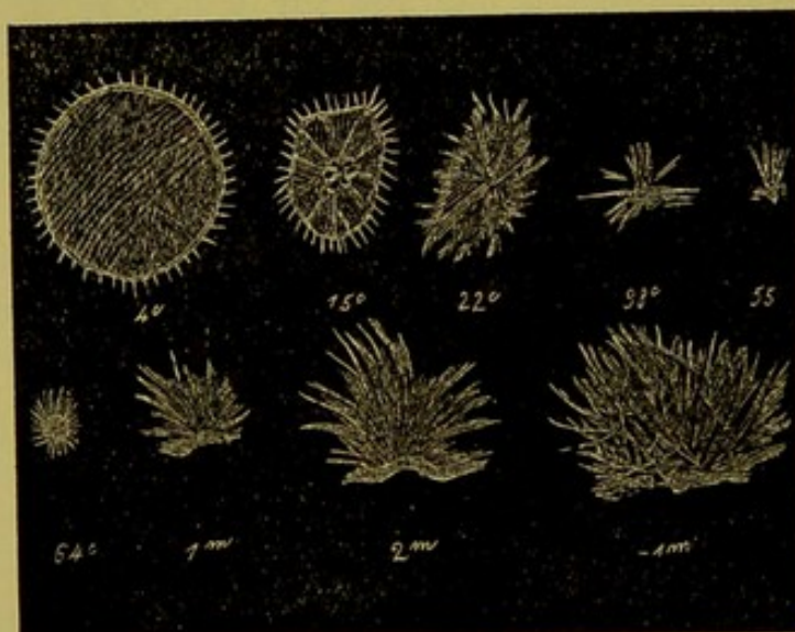
Fig. 92. — Irregular eye (Diplopia). After Rée .
