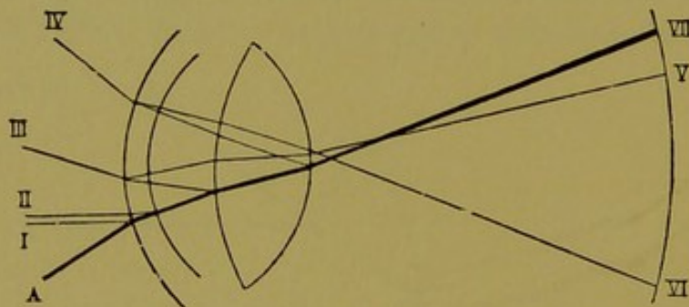
Fig. 29. — Manner in which a luminous ray is divided in the eye. A, incident ray. — I, II, III, IV, lost rays corresponding to the four images of Purkinje ; V and VI, harmful rays corresponding to the fifth and sixth image; VII, useful ray.
