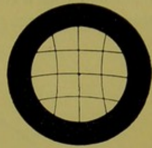
Fig. 93. — Aberroscopic phenomena of my right eye.
