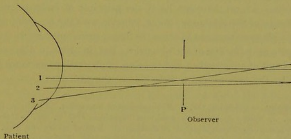
Fig. 141. — Theory of the paracentral shadow.
