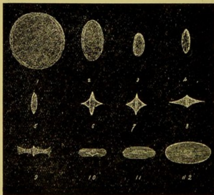
Fig. 87. — Figures of a luminous point obtained by combining an ordinary strong spherical lens with a cylindrical lens (astigmatism with spherical aberration). After Rée .
