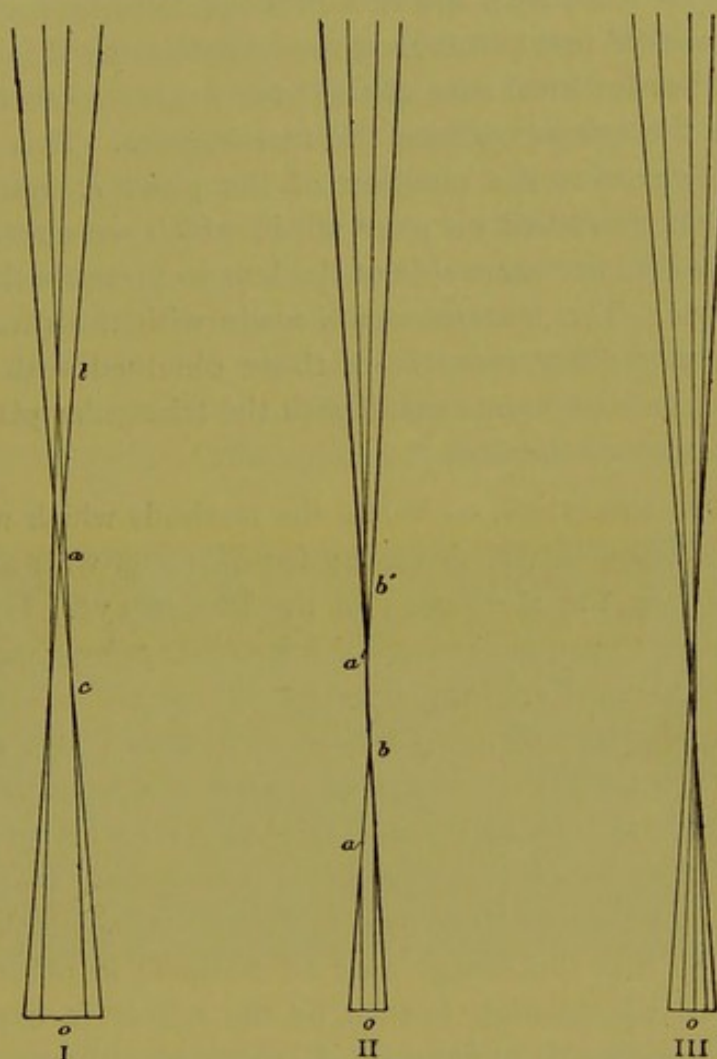
Fig. 68. — I and II. The appearance assumed by the line of the optometer of Young , seen through four slits by one eye with strong spherical aberration. O, position of the eye; a ( a' ) far point of the peripheral parts; b ( b' ) far point of the central parts.
