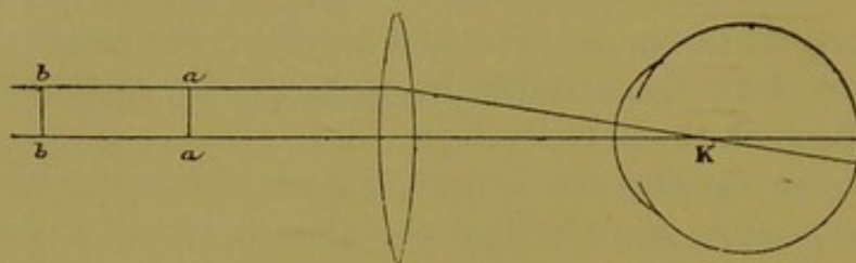
Fig. 58. — Principle of Badal .
