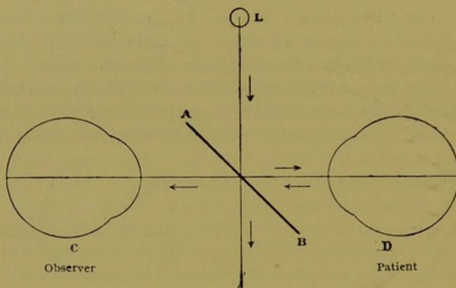
Fig. 127. — Principle of the ophthalmoscope of Helmholtz.
