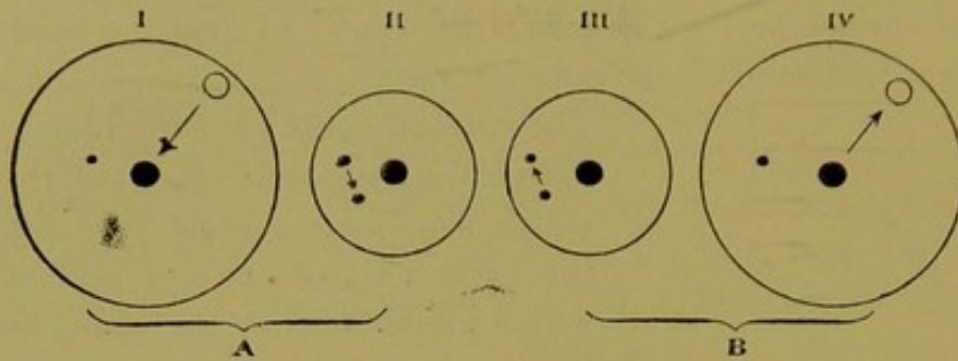
Fig. 120. — The four apparent phases of accommodation. ● Corneal image. — ○ Image of the anterior surface of the crystalline. — • Image of the posterior surface of the crystalline. A, accommodation; B, relaxation.
