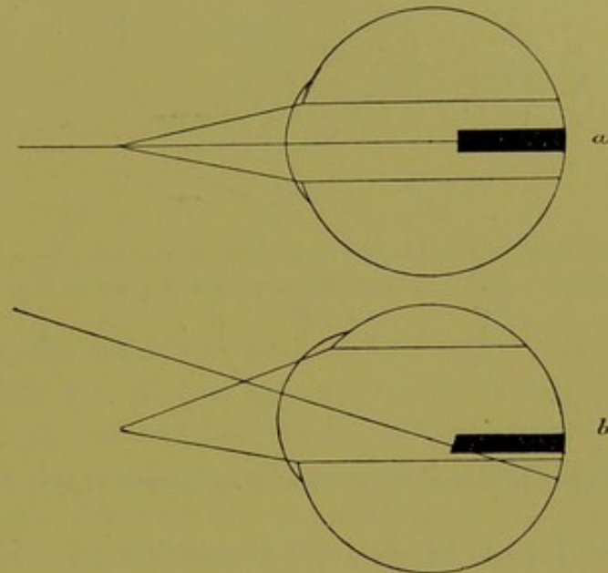
Fig. 102. — Parallax of the entoptic phenomena.
