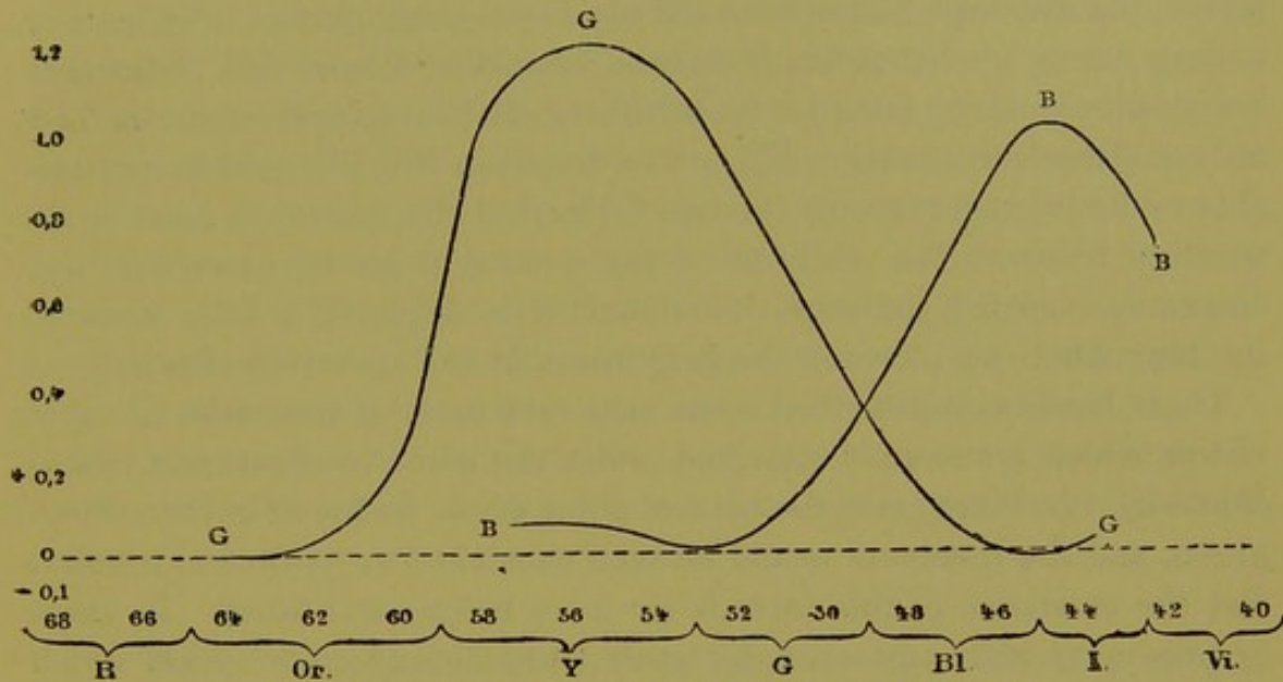
Fig. 166.—Color curves of a dichromatic, after Maxwell.
