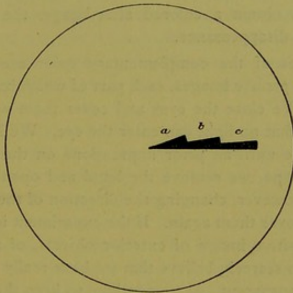
Fig. 155. — Disc of Masson .
