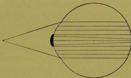
Fig. 104. — The drop on the cornea causes convergence of the rays which pass through it so that we see a luminous center surrounded by a shadow.
