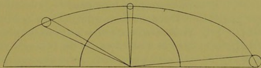
Fig. 186. After Young. — The curve indicates the apparent form of the sky. The sun, although seen under the same angle, seems of variable size.
