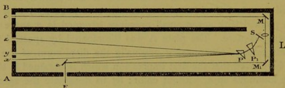
Fig. 157. — "Color box" of Maxwell .
