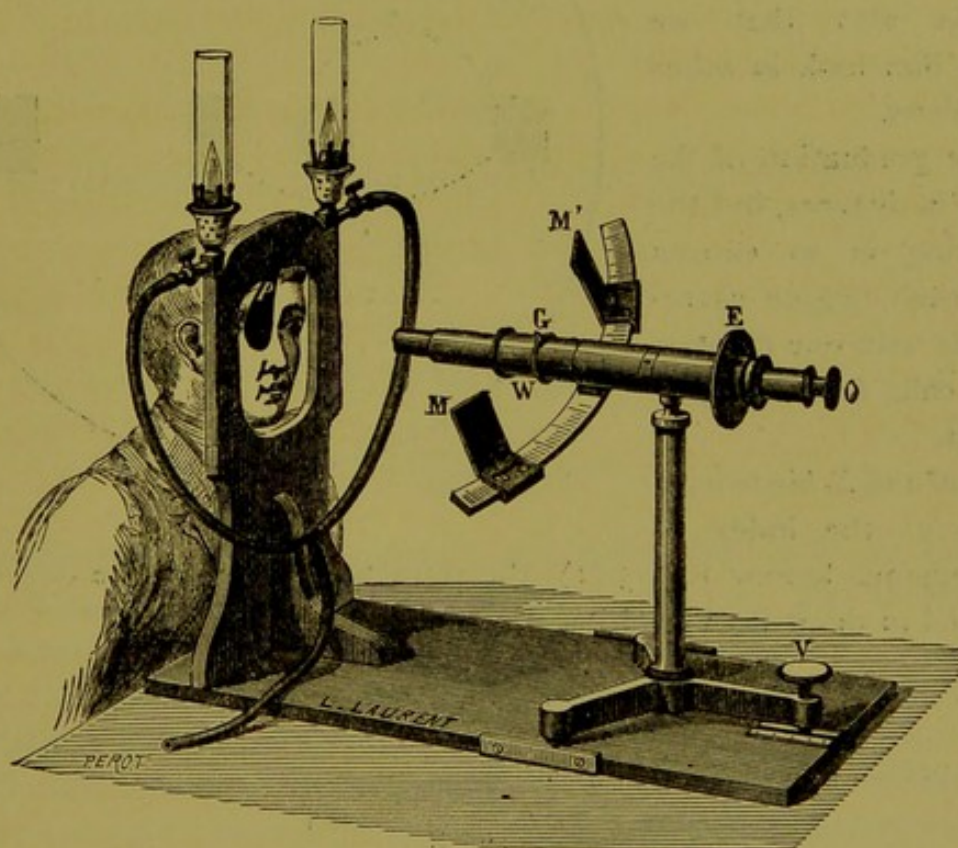
Fig. 38. — Ophthalmometer of Javal and Schioetz .
