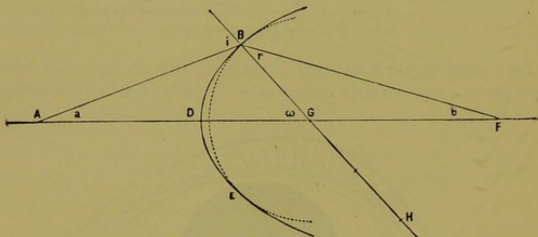
Fig. 118. — Refraction by a parabolic surface.
