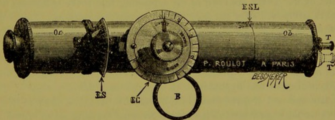
Fig. 168.—Chromatoptometer of Chibret .
