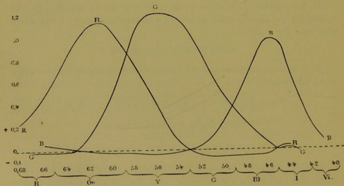
Fig. 162. — Color-curves of Maxwell.
