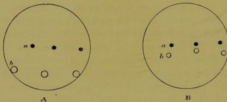
Fig. 115. — Reflection images of the right eye of Mme T. — A , in a state of repose; B , during accommodation (after a drawing of Professor Koster). — a , corneal images; b , images of anterior surface of the crystalline lens. Accommodation of 6 D.
