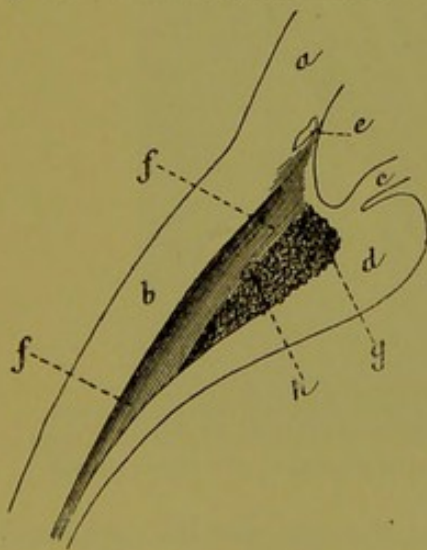
Fig. 109. — Ciliary muscle of man. (After H. Müller .)
