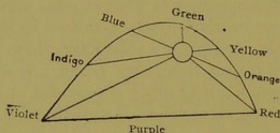
Fig. 164. — Color table of Helmholtz .
