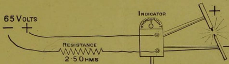
Diagram of connections for 8 ampère A pattern "Newtonian" Lamp on 65 volt circuit.
