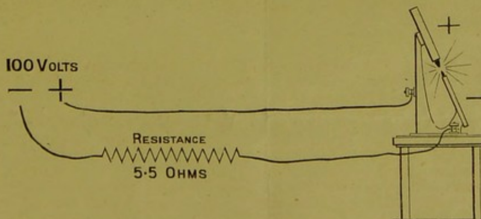
Diagram of connections for 10 ampère B pattern "Newtonian" Lamp on 100 volt circuit.
