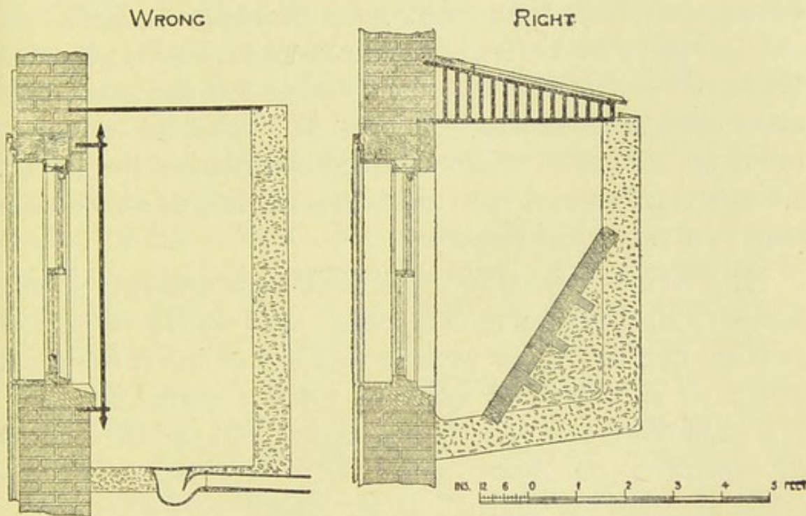
CELLAR WINDOW.
