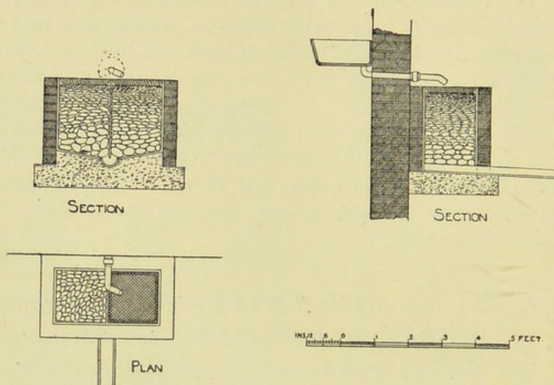
FIG. 28.—KITCHEN SINK WITH DUPLICATED OUTSIDE FILTER.
