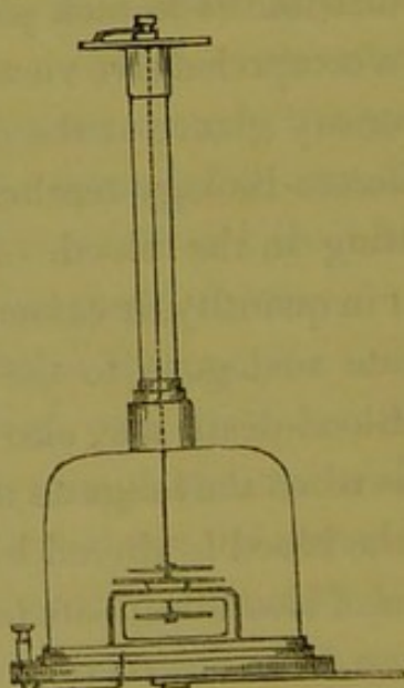
ASTATIC GALVANOMETER.
