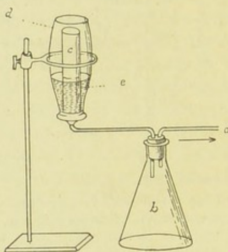
FIG. 31. — Chamberland's bougie arranged with lamp funnel for filtering a small quantity of fluid.
