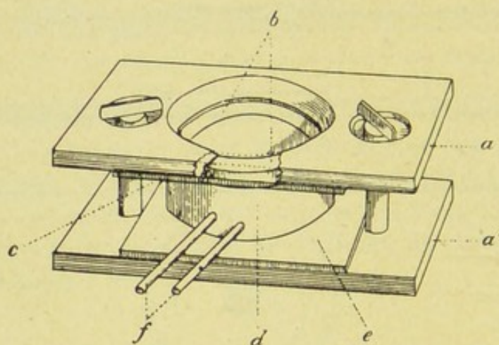
FIG. 27.—Graham Brown's chamber for anærobic hanging-drops.
