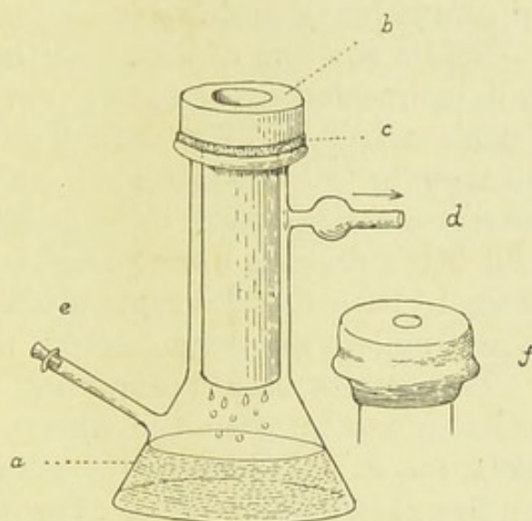
FIG. 33.—Muencke's modification of Chamberland's filter.
