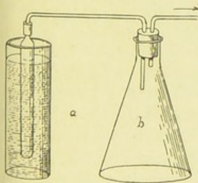
FIG. 30.—Chamberland's candle and flask arranged for filtration.
