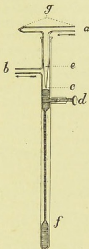
FIG. 36.—Reichert's gas regulator.
