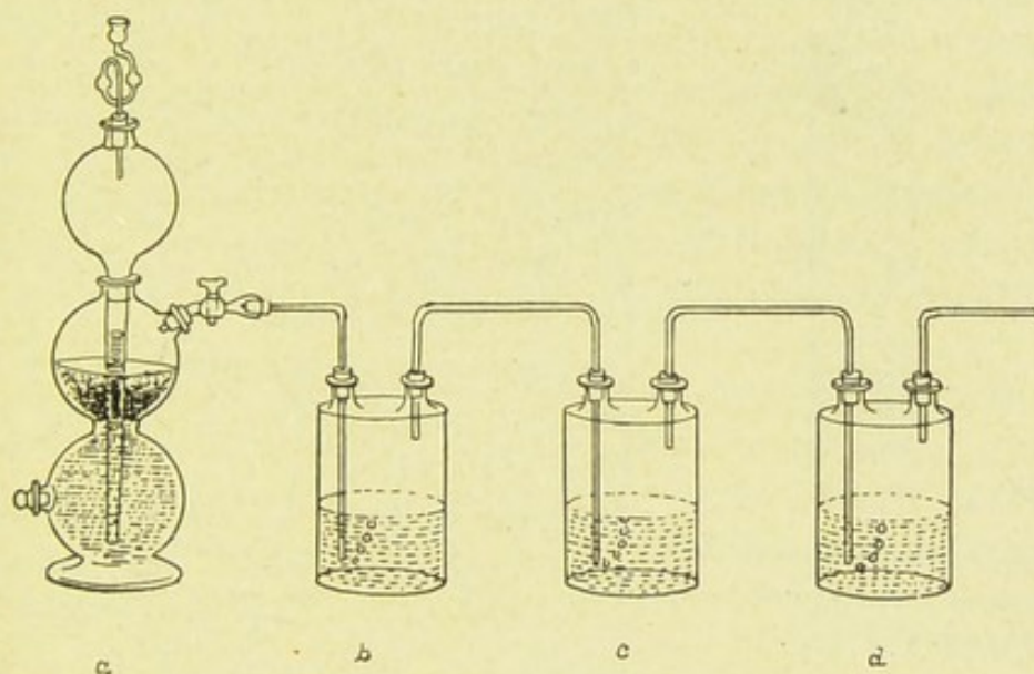
FIG. 21.—Apparatus for supplying hydrogen for anærobic cultures.
