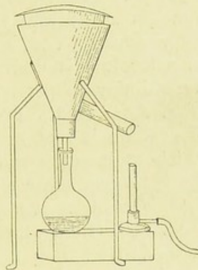
FIG. 7.—Hot-water funnel.
