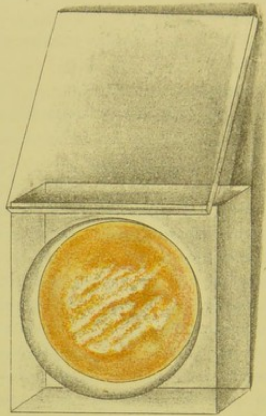
FIG. 56.—Tubercle bacillus upon solid serum.
