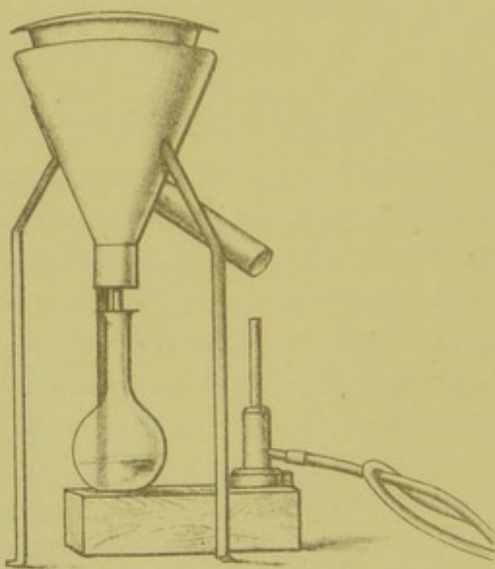
FIG. 32.—Hot water funnel for filtering meat jelly.
