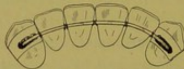
Diagram showing lingual view of Mitchell's splint, with two bands and bar.
