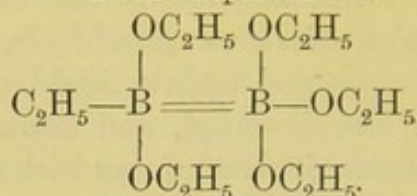
Boron-ethopentethoxide.
