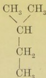
Isopentane.
