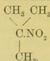
Tertiary Nitrobutane.
