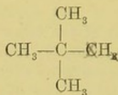
Isobutane.
