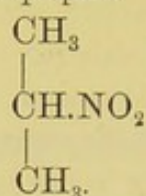
Secondary Nitropropane.
