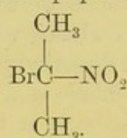
Secondary Bromnitropropane.
