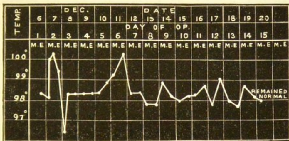
FIG. 12.—Temperature Chart.
