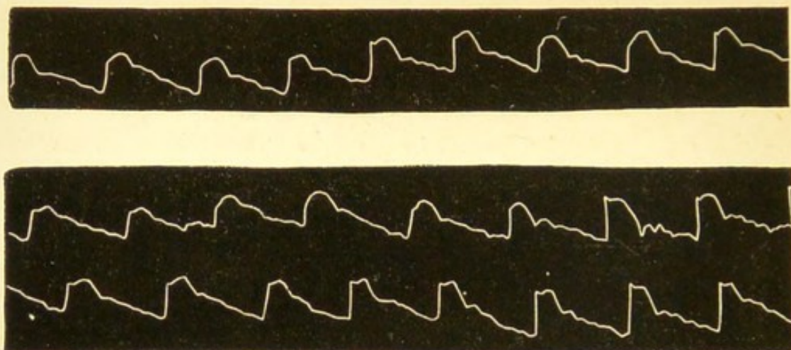
FIG. 6.—Sphygmographic Tracings.
