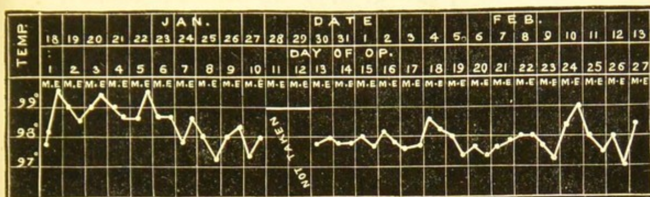
FIG. 7.—Temperature Chart.
