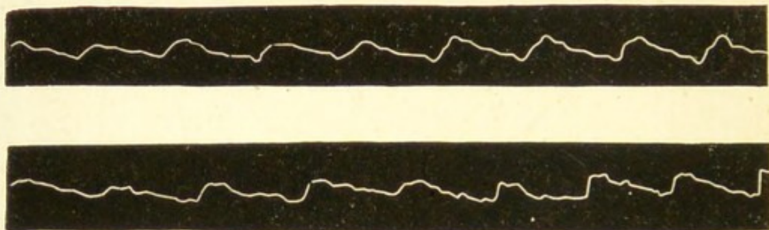
FIG. 11.—Sphygmographic Trace.
