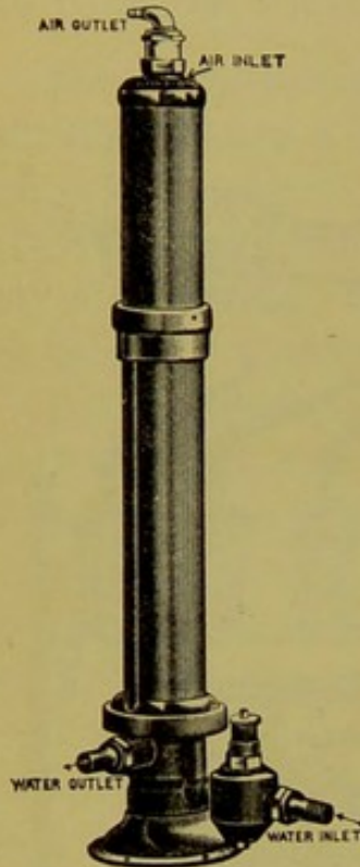
FIG. 19.—HYDRAULIC PUMP.
