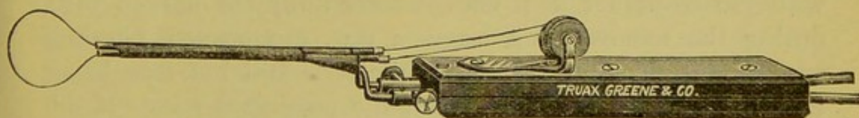
FIG. 136.—AMERICAN CAUTERY HANDLE, WITH WINDLASS.
