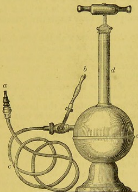
FIG. 62.—FORCE-PUMP.
