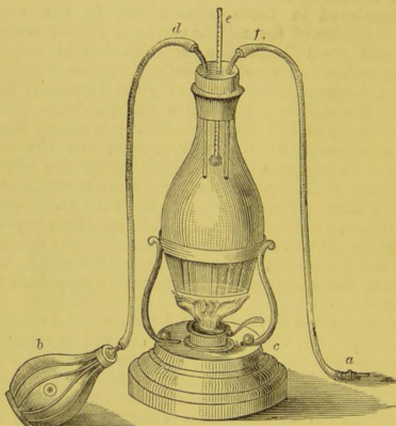
FIG. 65.—VOLATILIZATION APPARATUS.
