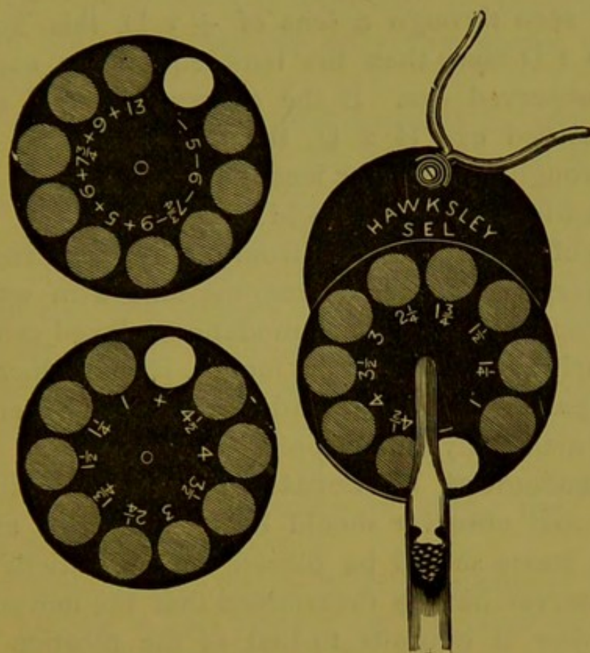
FIG. 28.—Oldham's Ophthalmoscope.
