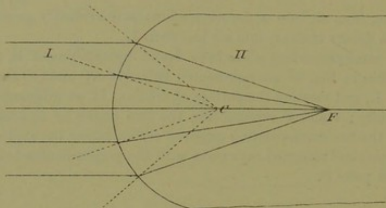
FIG. 69.—Shows the deflection of rays towards a focus, f , when the denser medium is bounded by a curved surface whose centre is at c .
