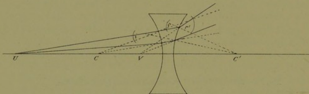
FIG. 76.—Showing the action of a concave lens in dispersing incident rays.
