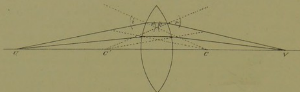
FIG. 75.—Showing the action of a convex lens in bringing rays to a focus.
