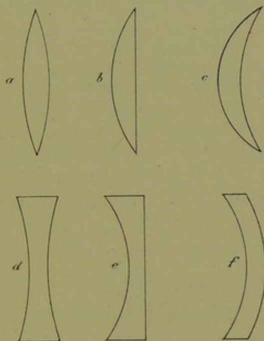
FIG. 74.—Different forms of convex and concave spherical lenses.
