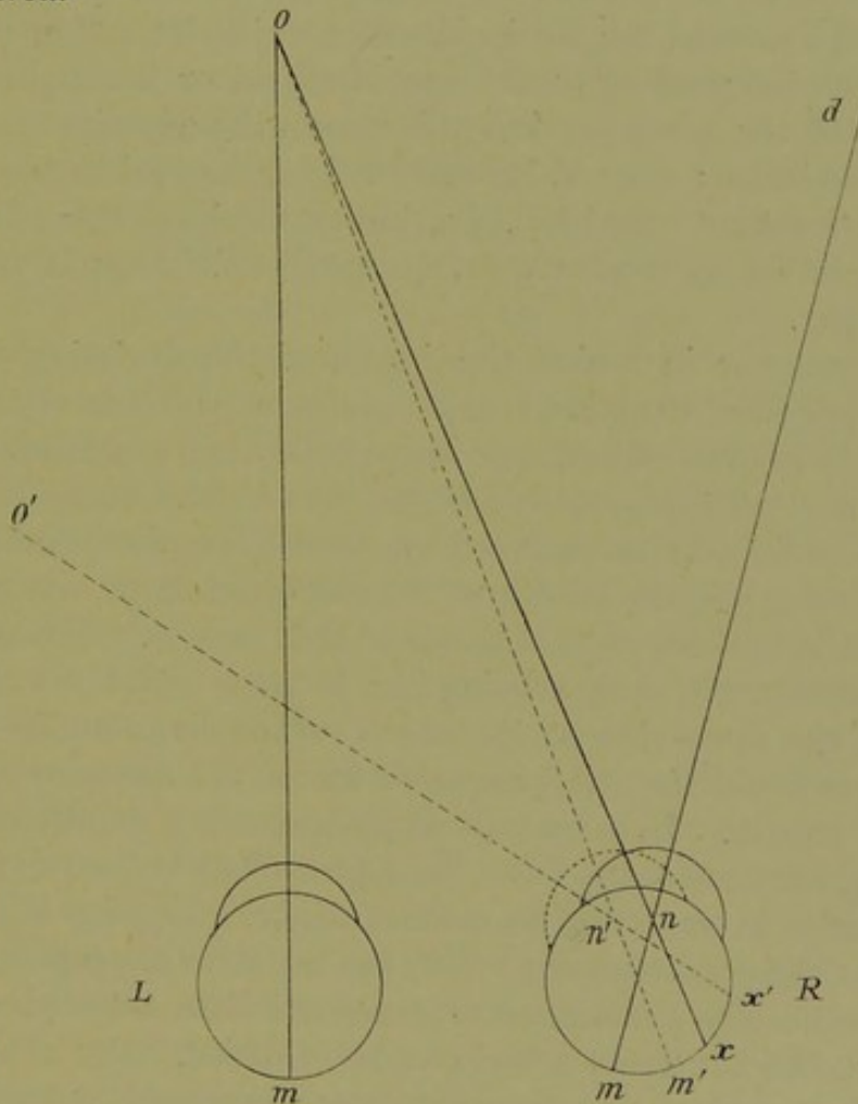
FIG. 107.—Shows manner of projection in abnormal divergence. Lettering as in Fig. 106. x' n' O' , direction in which image of O is projected by right eye.
