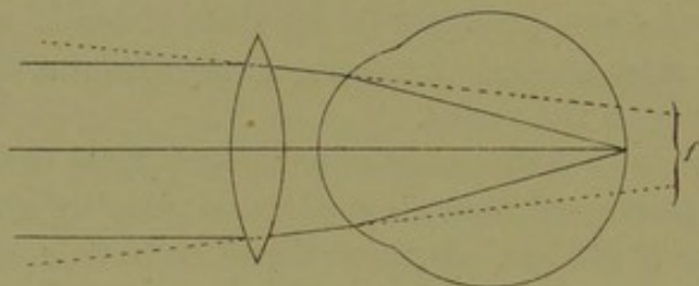
FIG. 78.—Showing action of a convex lens placed in front of the eye, causing parallel rays to enter the eye, as if directed to a point at a finite distance behind the eye.
