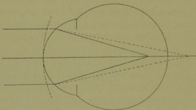
FIG. 72.—Showing the stronger refracting power of the more highly curved cornea (continuous line).
