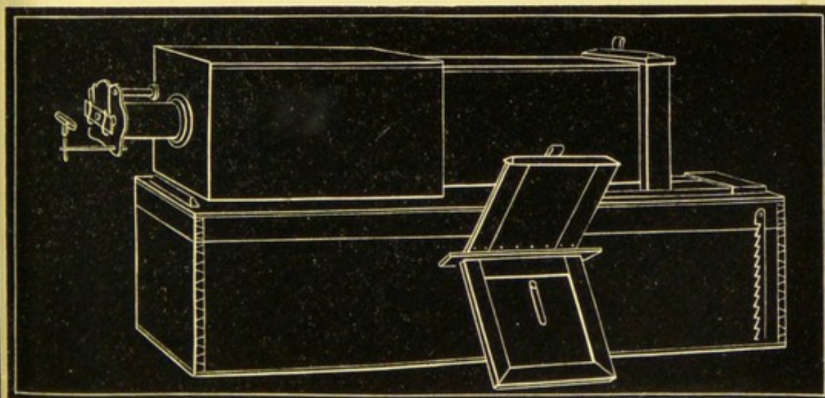
Fig. 140. Inverted microscope of Dr. Lawrence Smith, for examining objects in acid solutions, corrosive fluids, &c. a . Tube of microscope with eye-piece. b . Object glass over the box which contains the prism resembling that represented at g . c . Stage with slide upon it. d . Support on which polarizing apparatus or condenser may be placed. e . Mirror. f . Screw by which the stage is elevated or depressed in focussing. g . Prism showing the direction in which the rays of light passing through it are refracted. h . Position of achromatic object glass.
